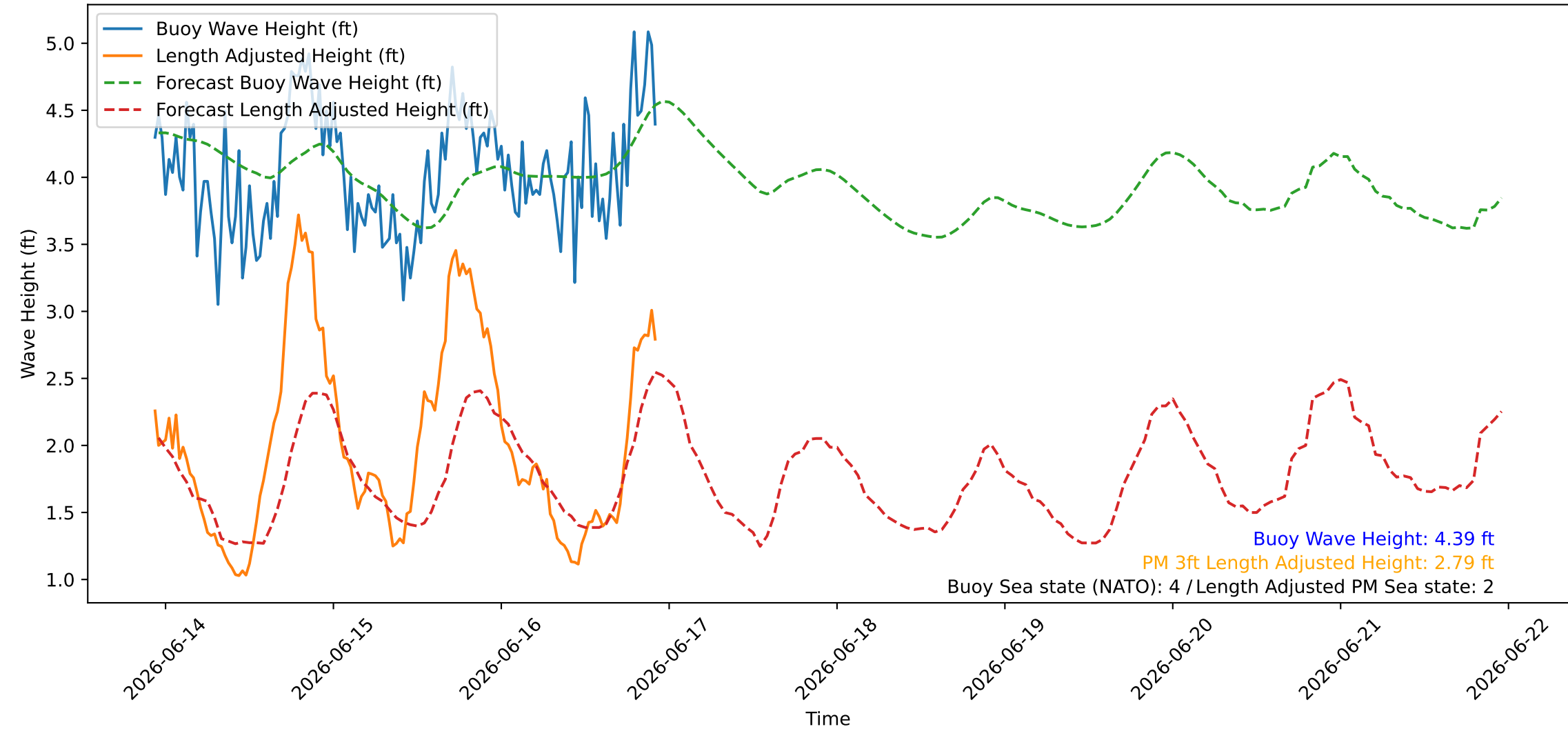
Wave Heights over Time for Green Beach at 2026-06-16 22:41:08
