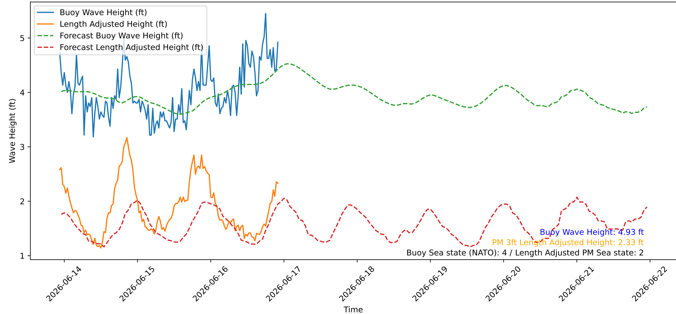
Wave Heights over Time for Oceanside Harbor at 2026-06-16 22:40:26
