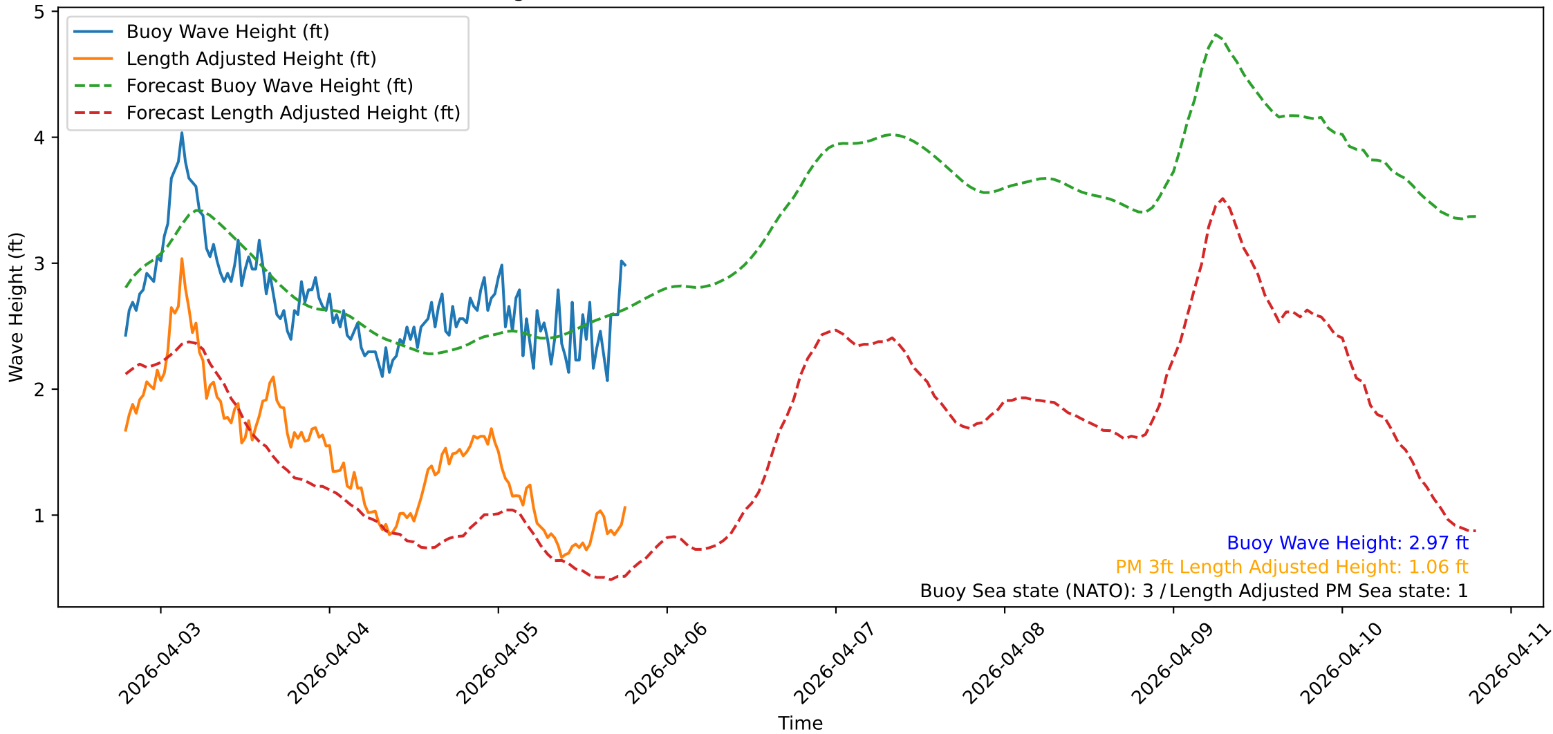
Wave Heights over Time for Oceanside Harbor at 2026-04-05 18:50:33
