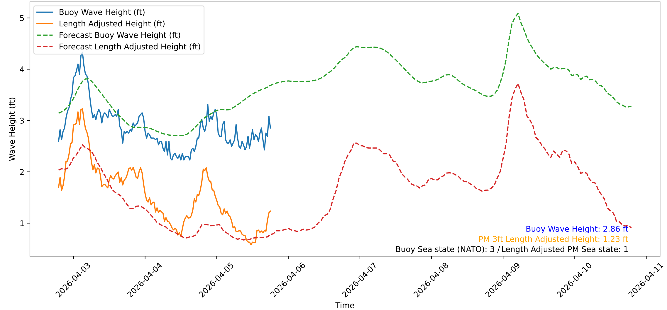
Wave Heights over Time for Green Beach at 2026-04-05 18:51:15
