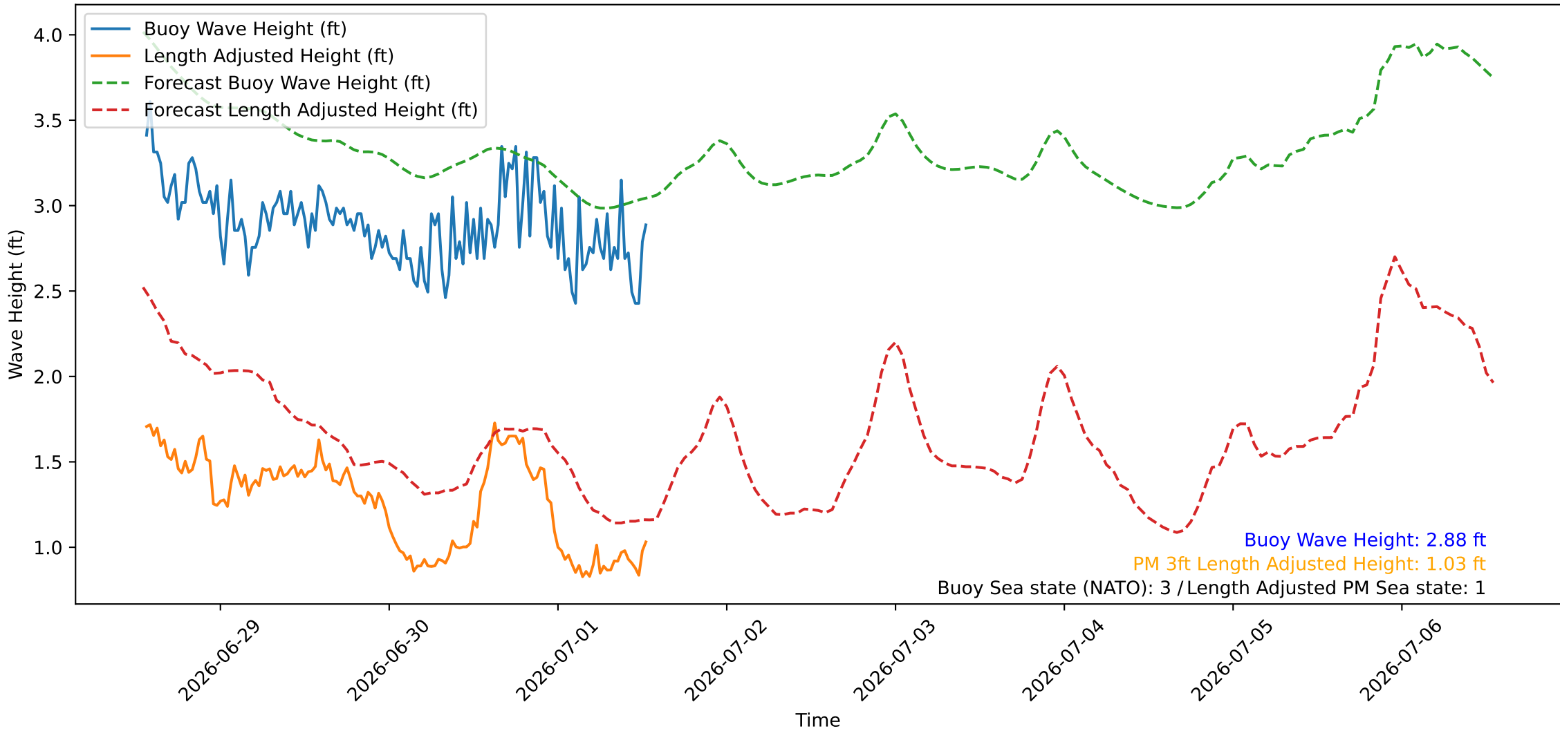
Wave Heights over Time for Red Beach at 2026-07-01 13:20:47
