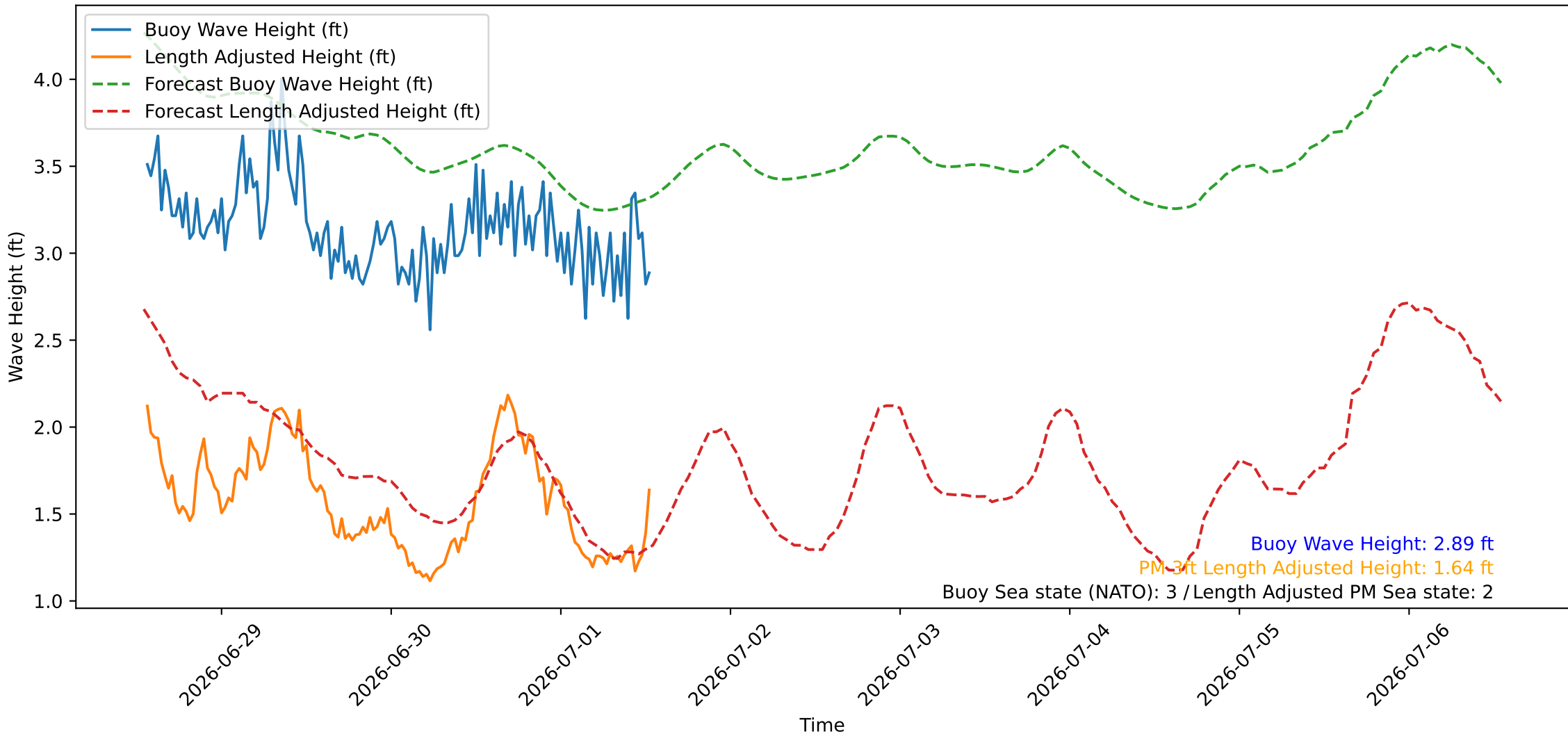
Wave Heights over Time for Oceanside Harbor at 2026-07-01 13:20:27
