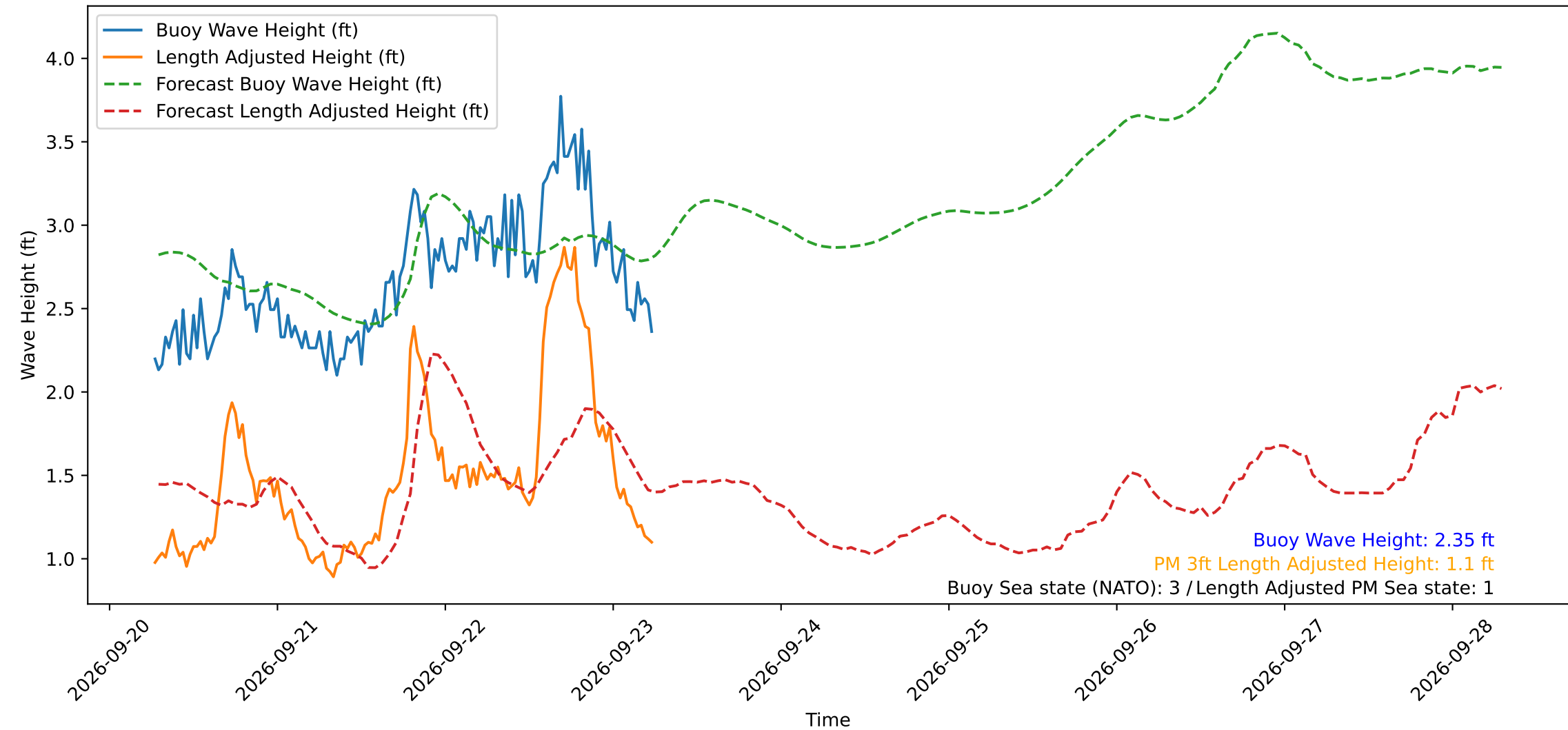
Wave Heights over Time for Oceanside Harbor at 2026-09-23 06:30:29
