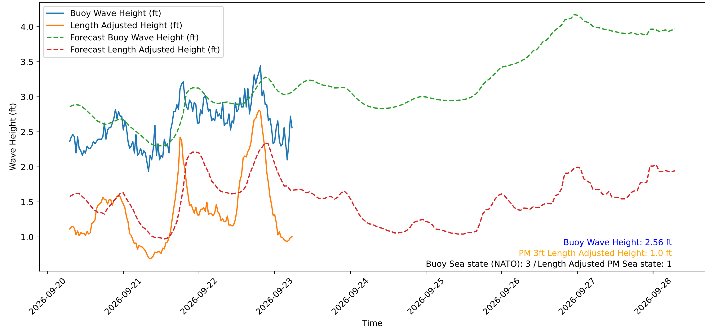
Wave Heights over Time for Green Beach at 2026-09-23 06:31:12
