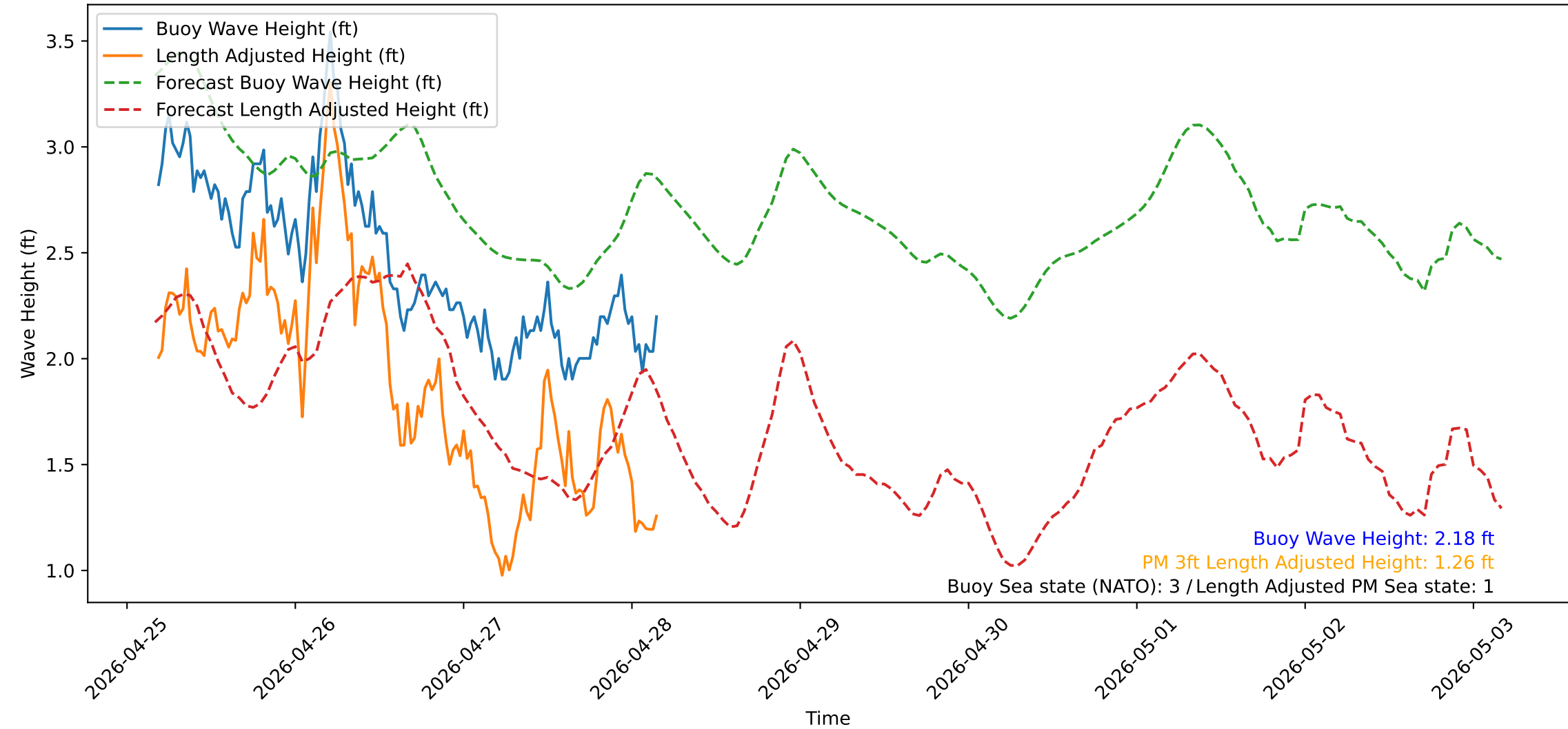
Wave Heights over Time for Red Beach at 2026-04-28 04:10:51
