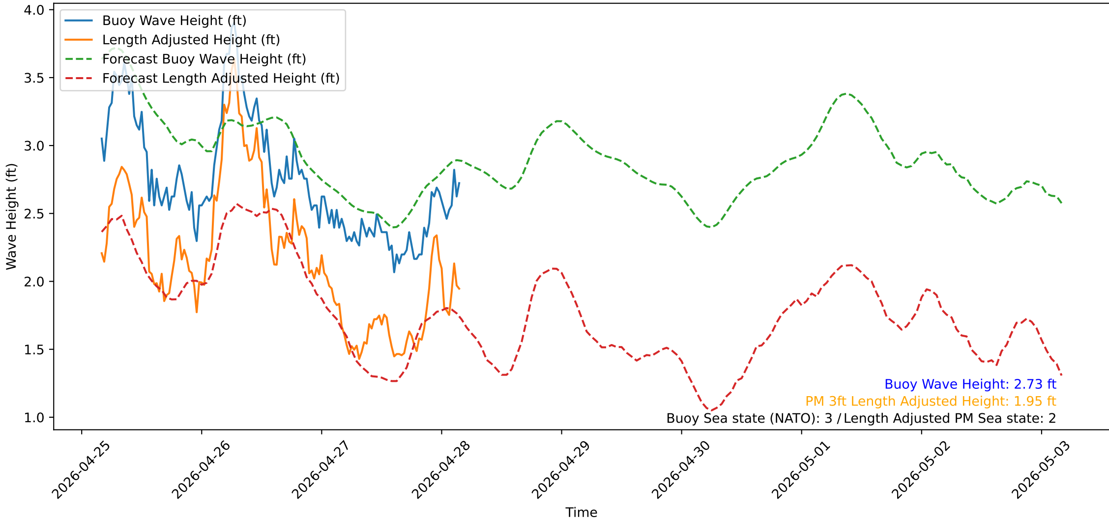
Wave Heights over Time for Oceanside Harbor at 2026-04-28 04:10:32
