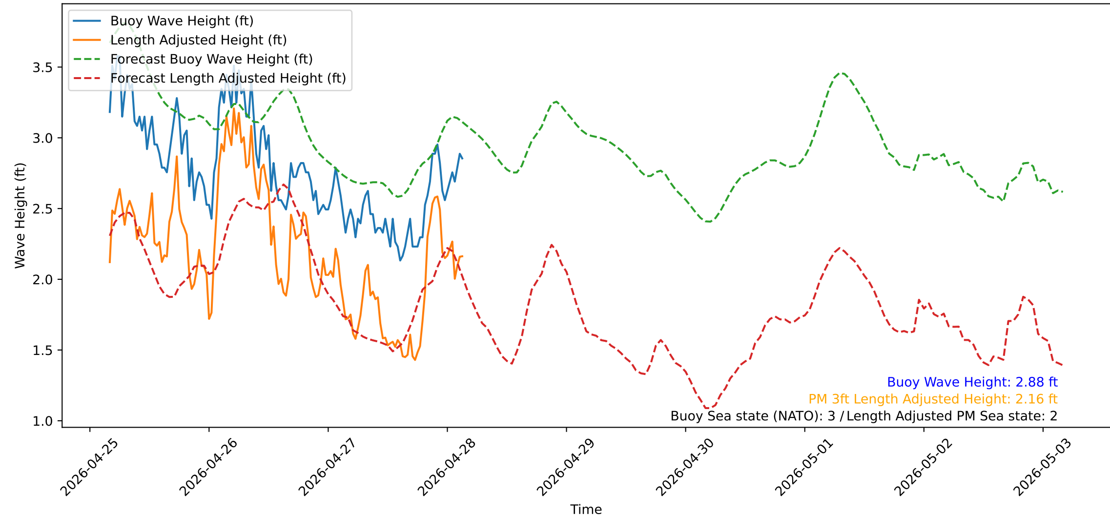
Wave Heights over Time for Green Beach at 2026-04-28 04:11:13
