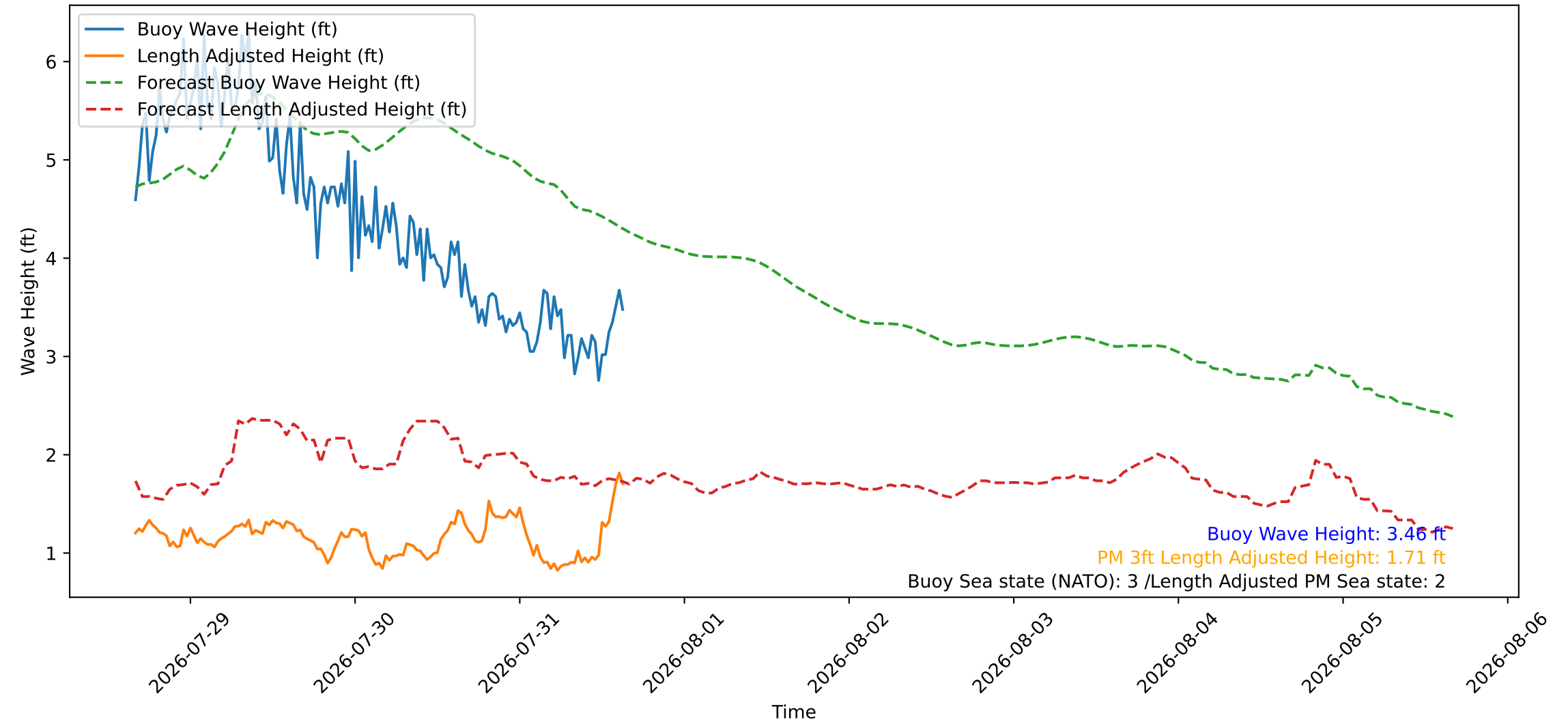
Wave Heights over Time for Green Beach at 2026-07-31 15:51:10
