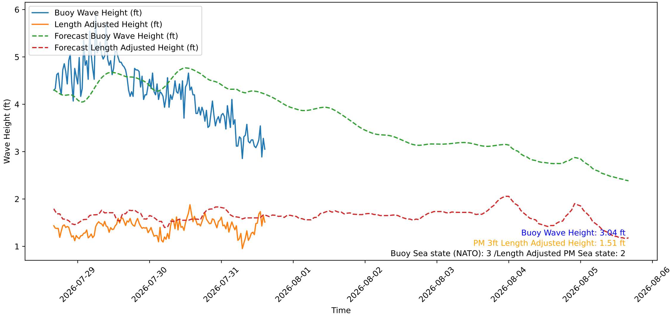
Wave Heights over Time for Oceanside Harbor at 2026-07-31 15:50:26
