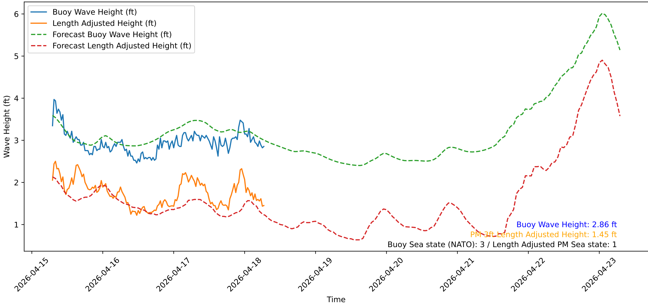
Wave Heights over Time for Green Beach at 2026-04-18 07:11:12
