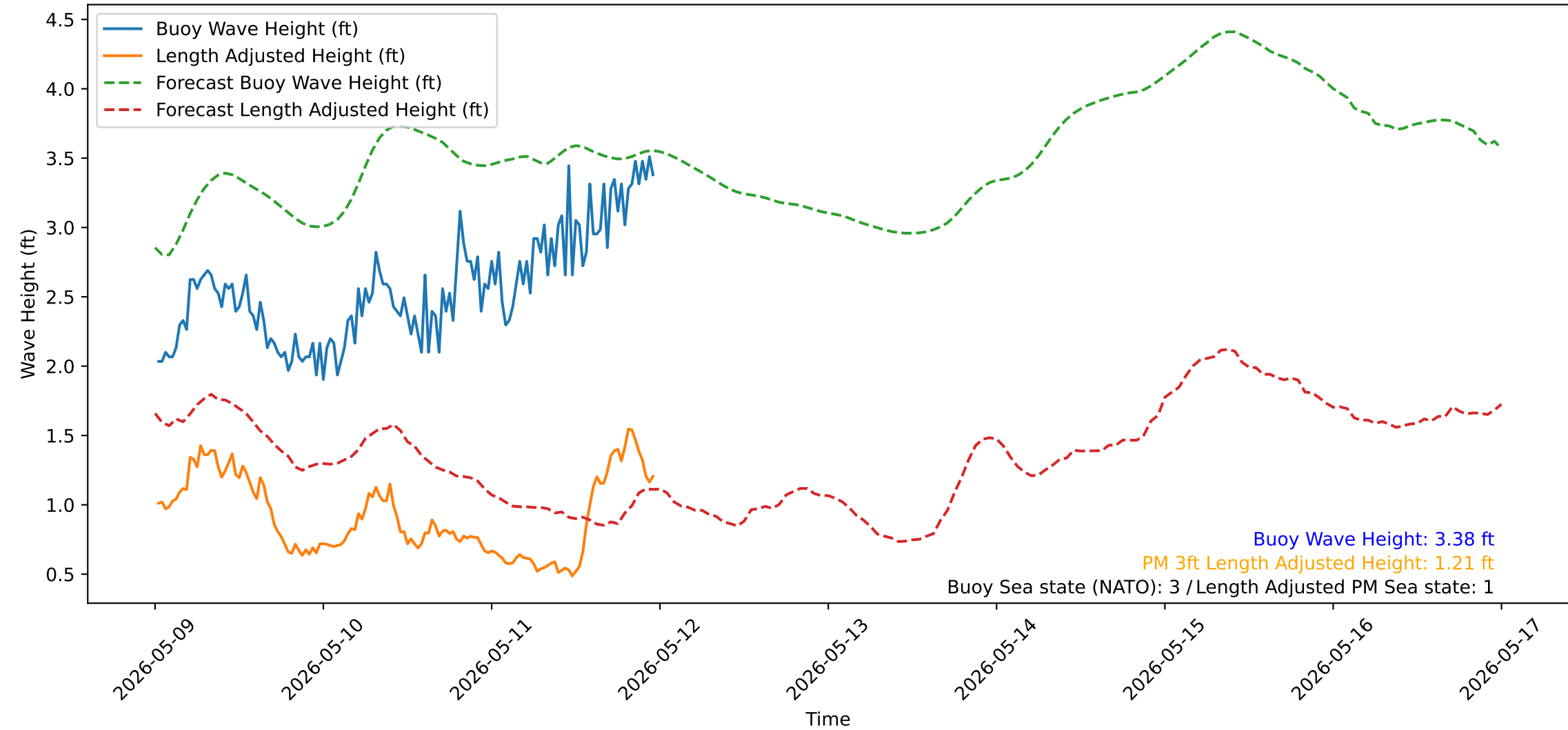
Wave Heights over Time for Green Beach at 2026-05-12 00:21:14
