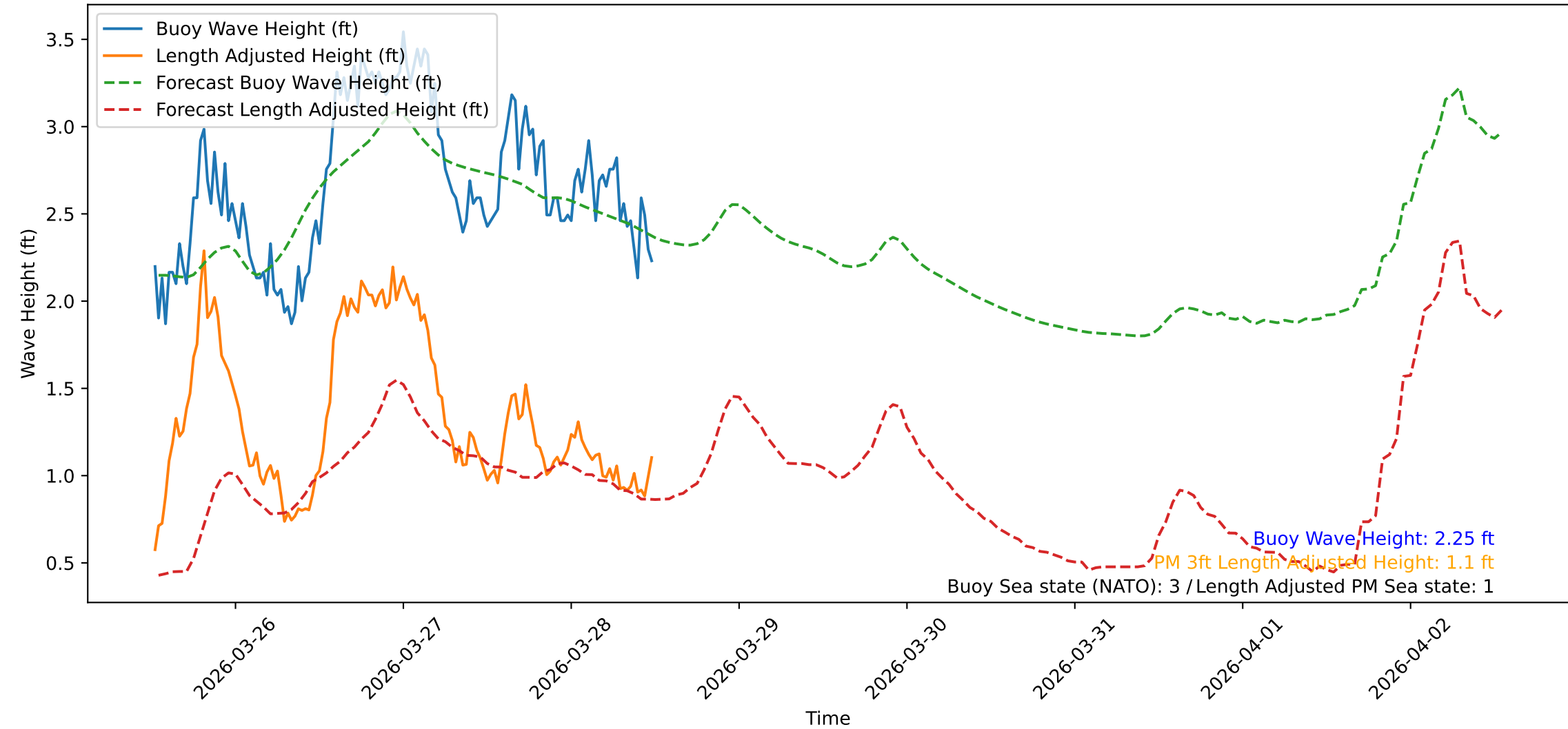
Wave Heights over Time for Green Beach at 2026-03-28 12:31:10
