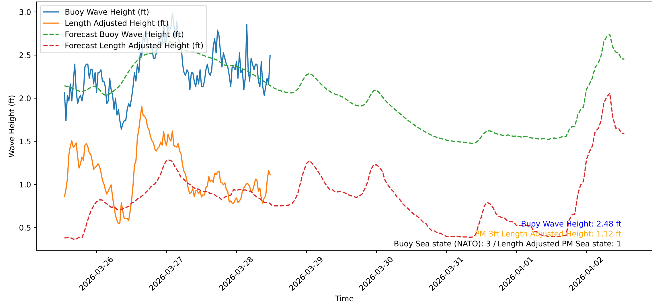
Wave Heights over Time for Red Beach at 2026-03-28 12:30:47
