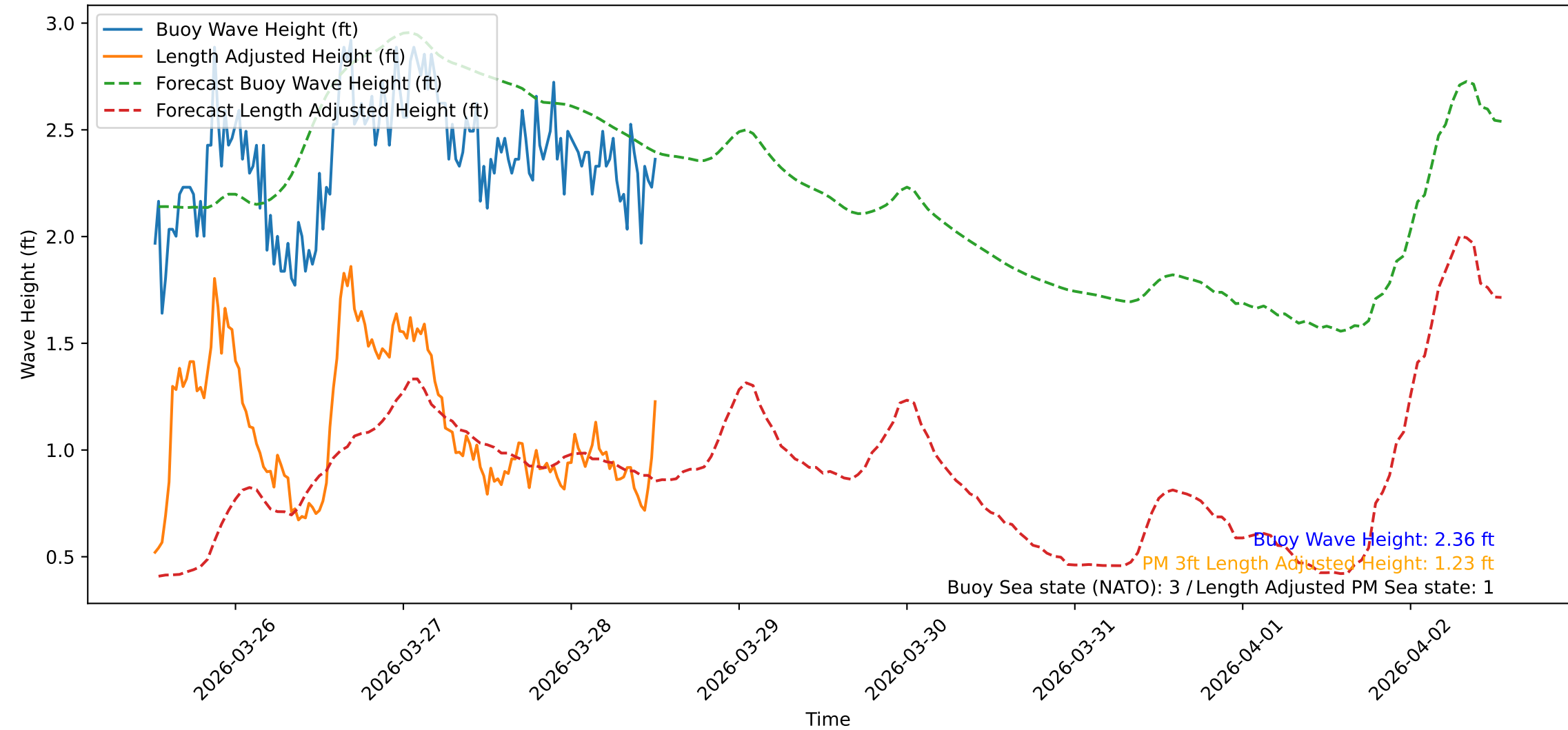
Wave Heights over Time for Oceanside Harbor at 2026-03-28 12:30:31
