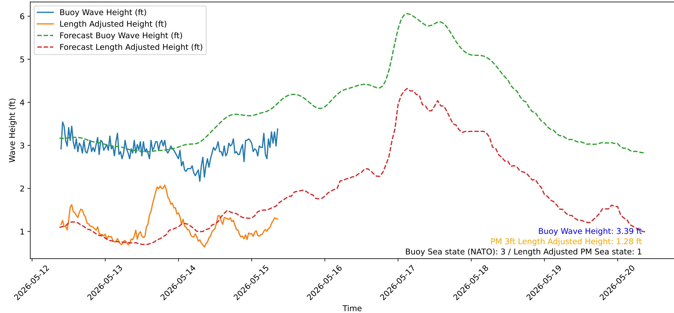
Wave Heights over Time for Oceanside Harbor at 2026-05-15 09:20:32
