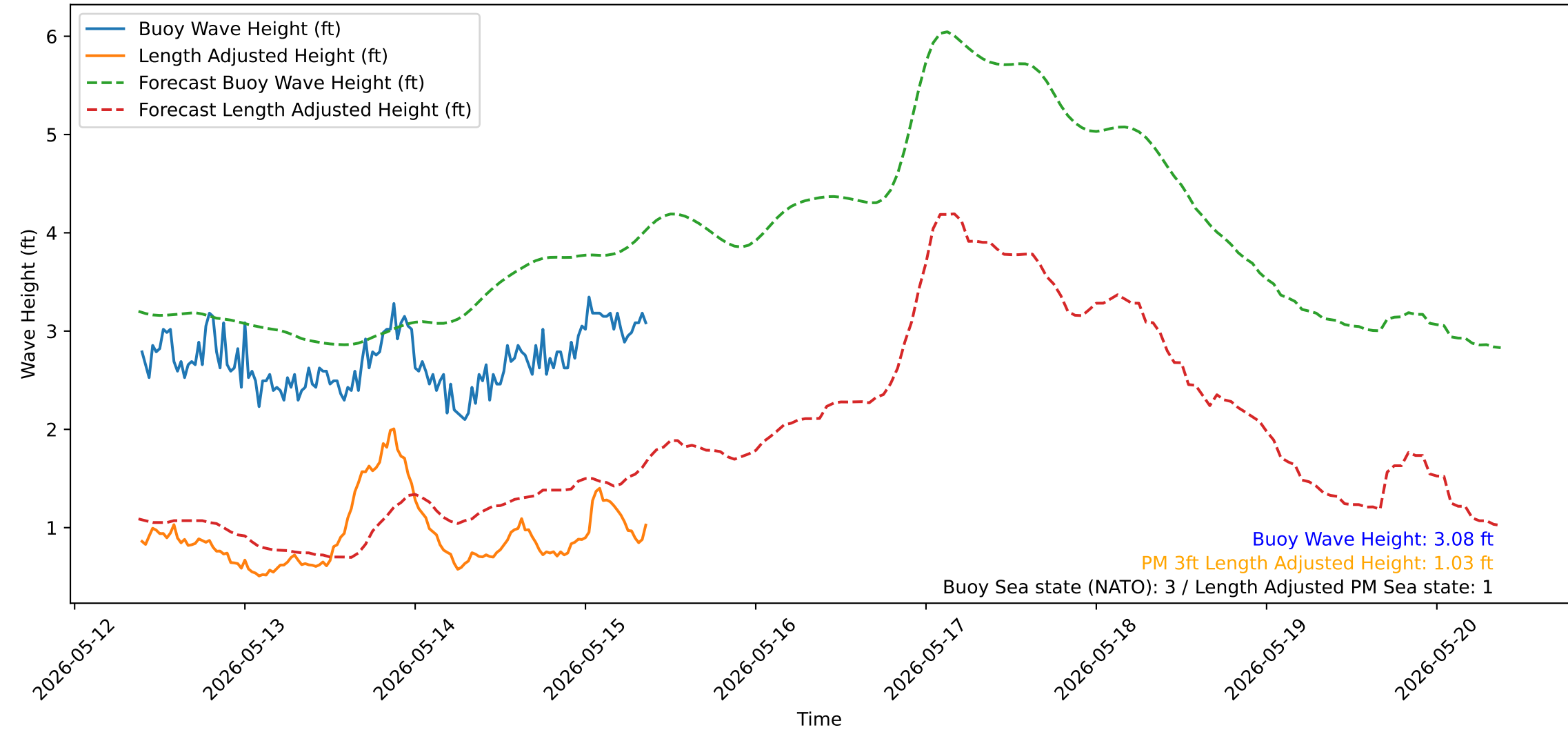
Wave Heights over Time for Green Beach at 2026-05-15 09:21:15
