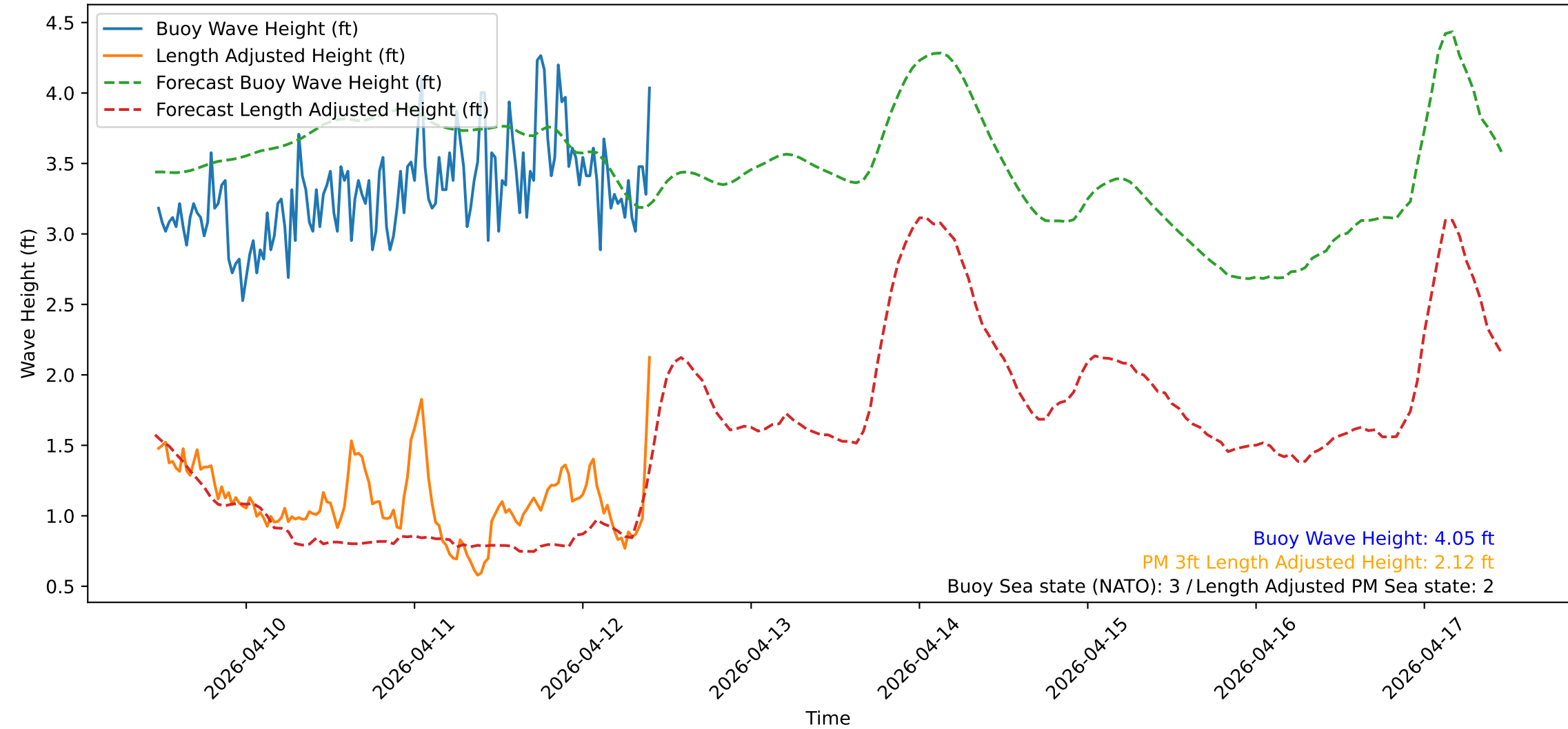
Wave Heights over Time for Red Beach at 2026-04-12 11:00:50
