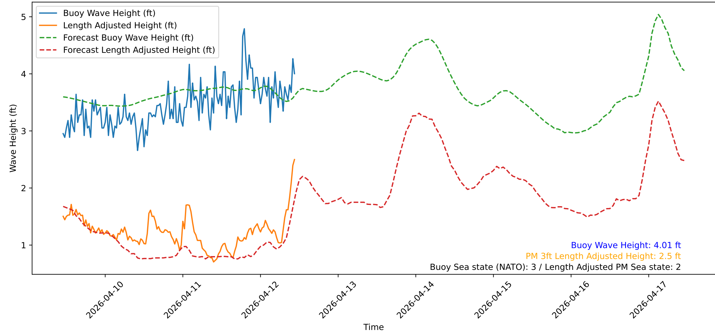
Wave Heights over Time for Oceanside Harbor at 2026-04-12 11:00:31
