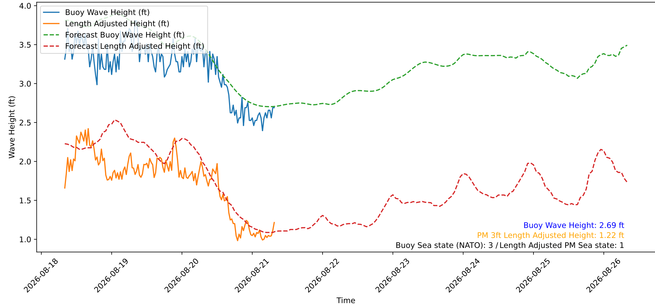
Wave Heights over Time for Oceanside Harbor at 2026-08-21 08:10:27
