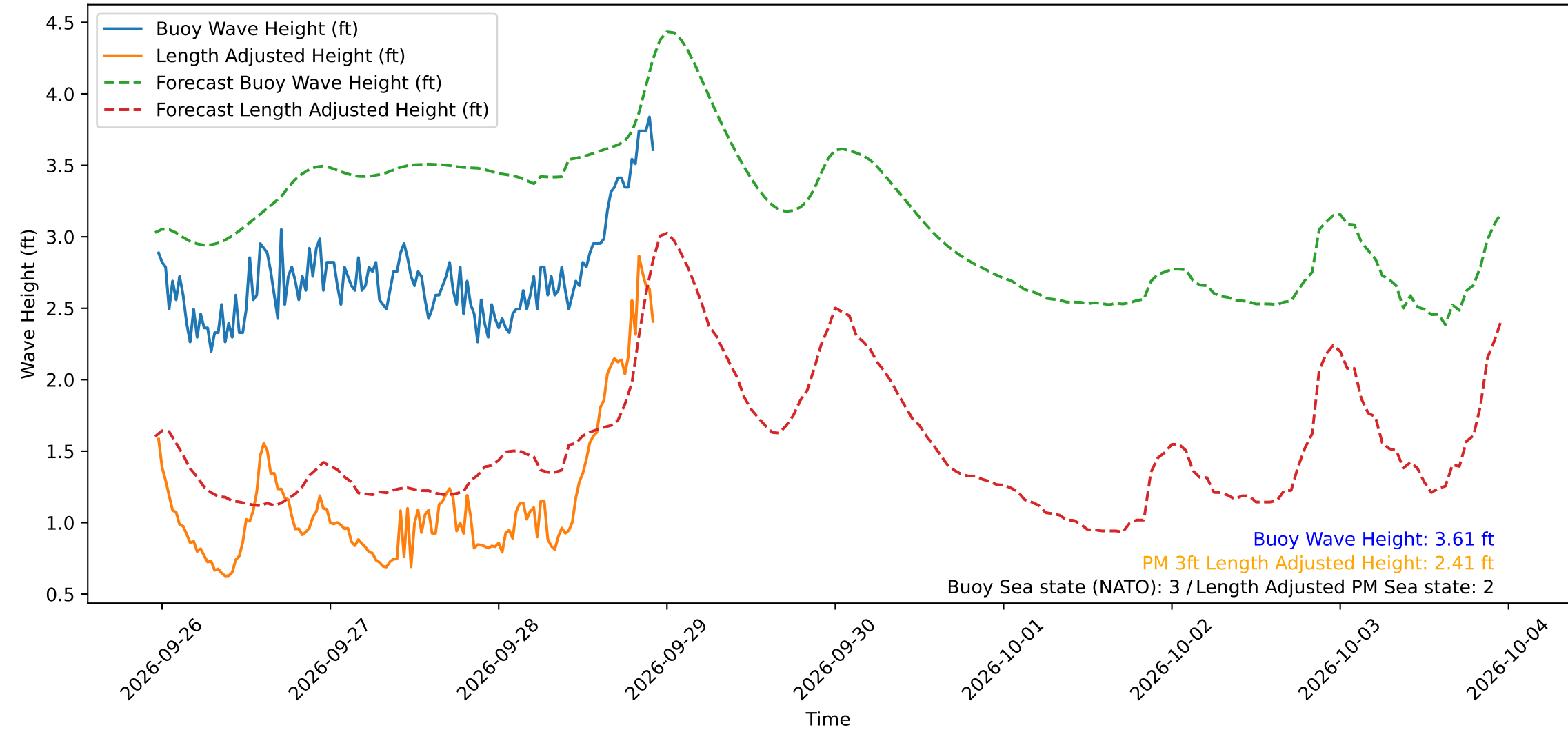
Wave Heights over Time for Red Beach at 2026-09-28 23:00:50
