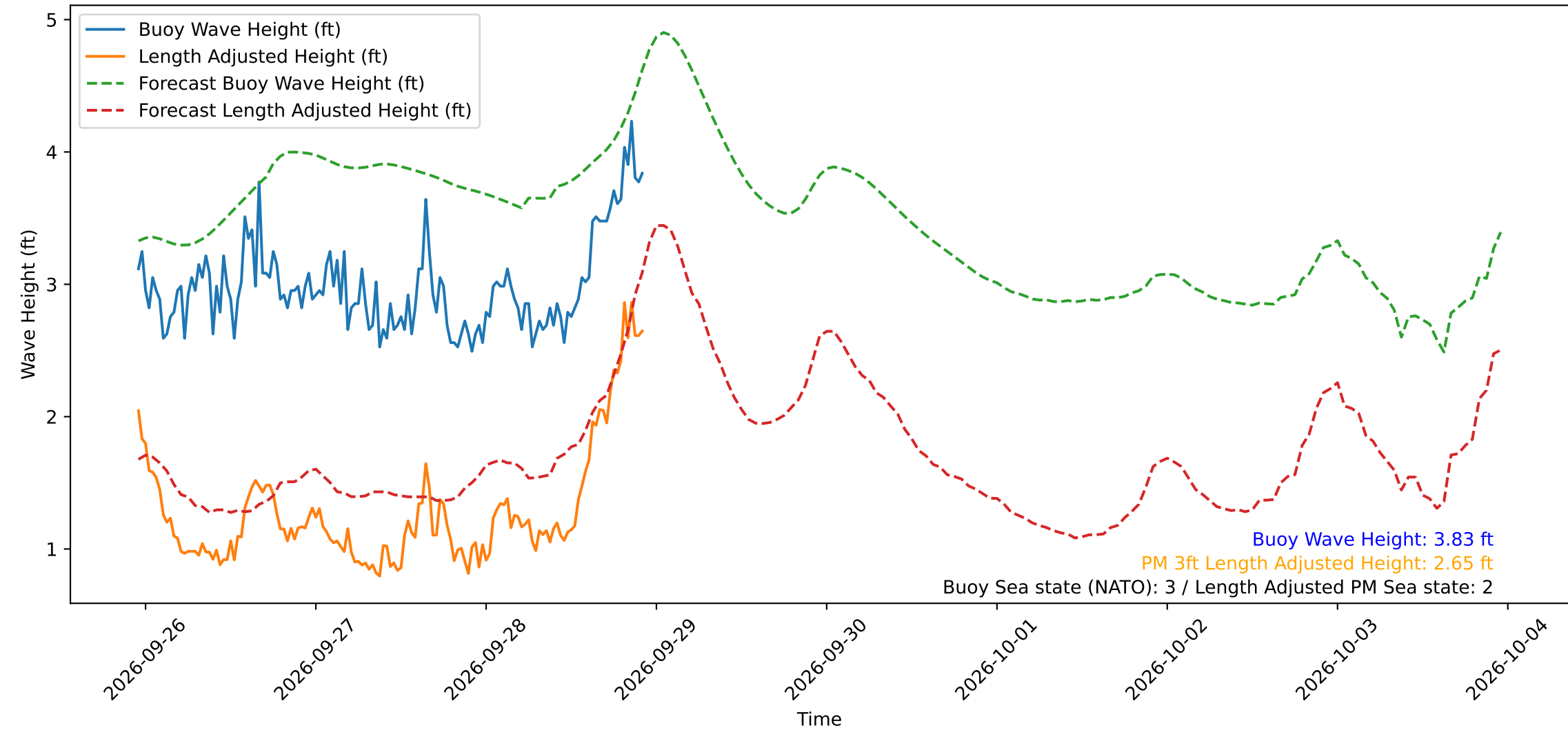
Wave Heights over Time for Oceanside Harbor at 2026-09-28 23:00:30
