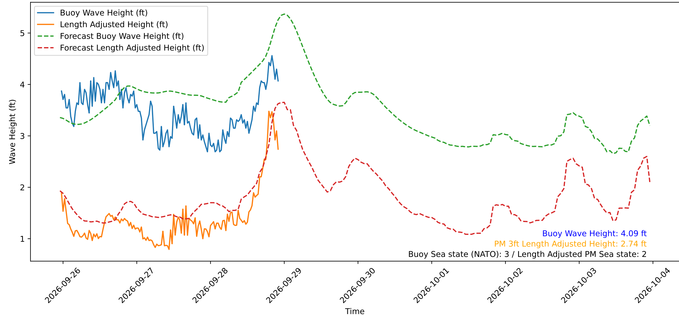
Wave Heights over Time for Green Beach at 2026-09-28 23:01:13
