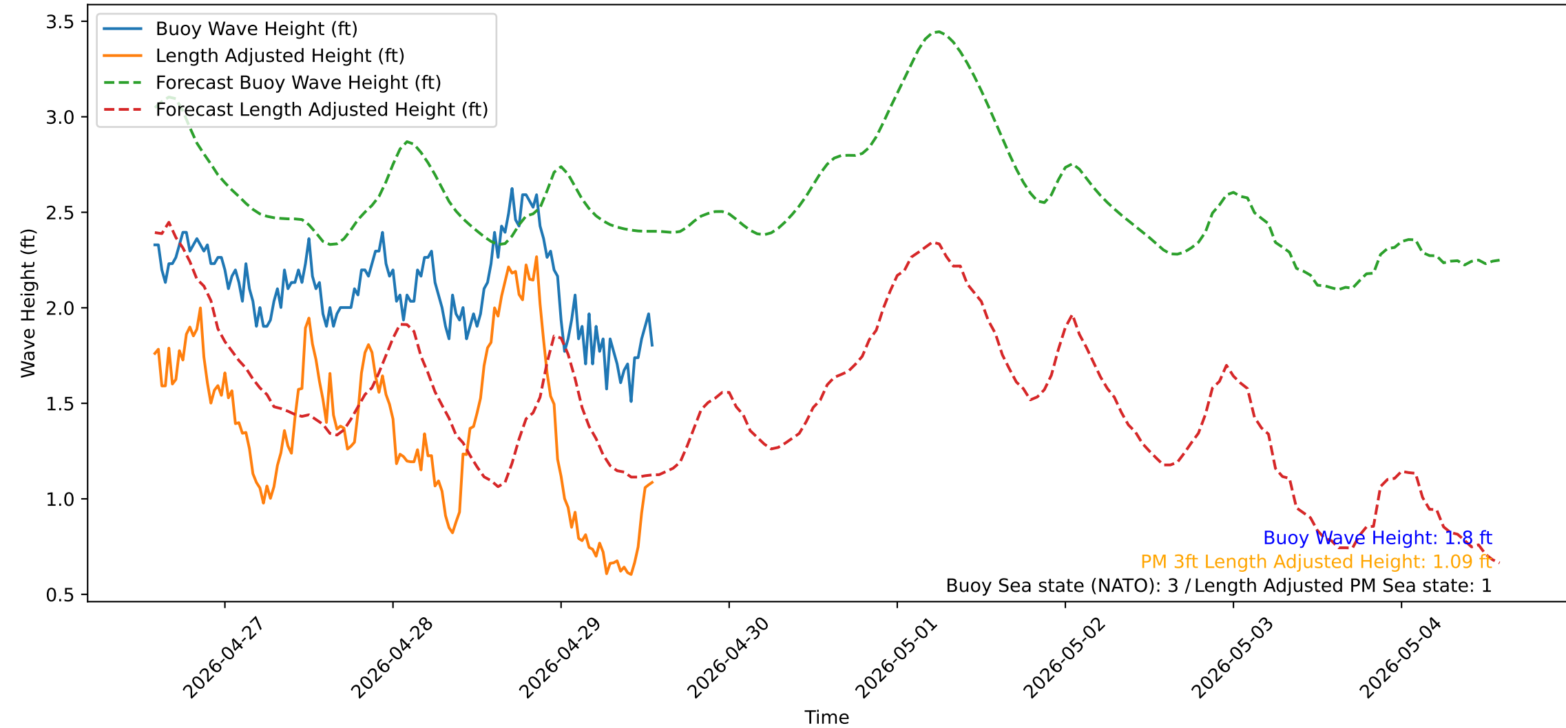
Wave Heights over Time for Red Beach at 2026-04-29 13:50:52
