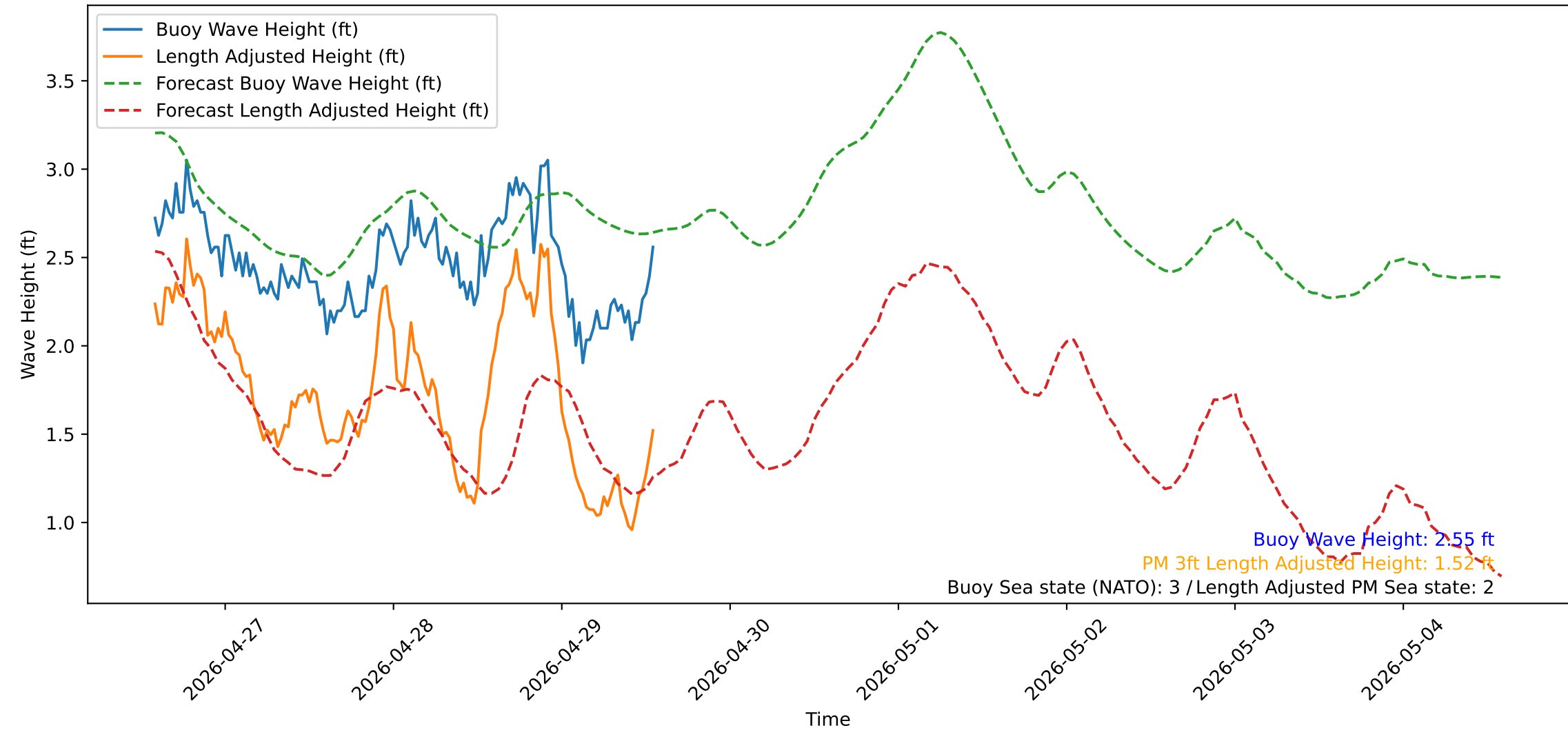
Wave Heights over Time for Oceanside Harbor at 2026-04-29 13:50:31
