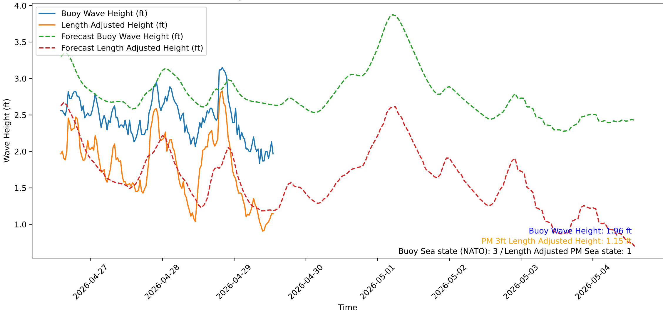
Wave Heights over Time for Green Beach at 2026-04-29 13:51:15
