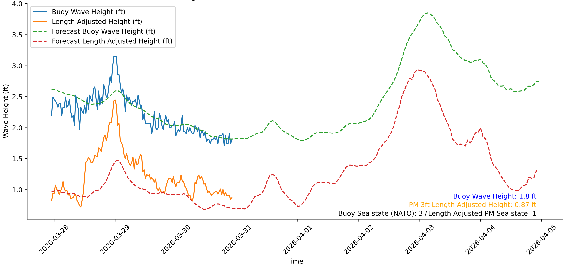
Wave Heights over Time for Oceanside Harbor at 2026-03-30 22:50:32
