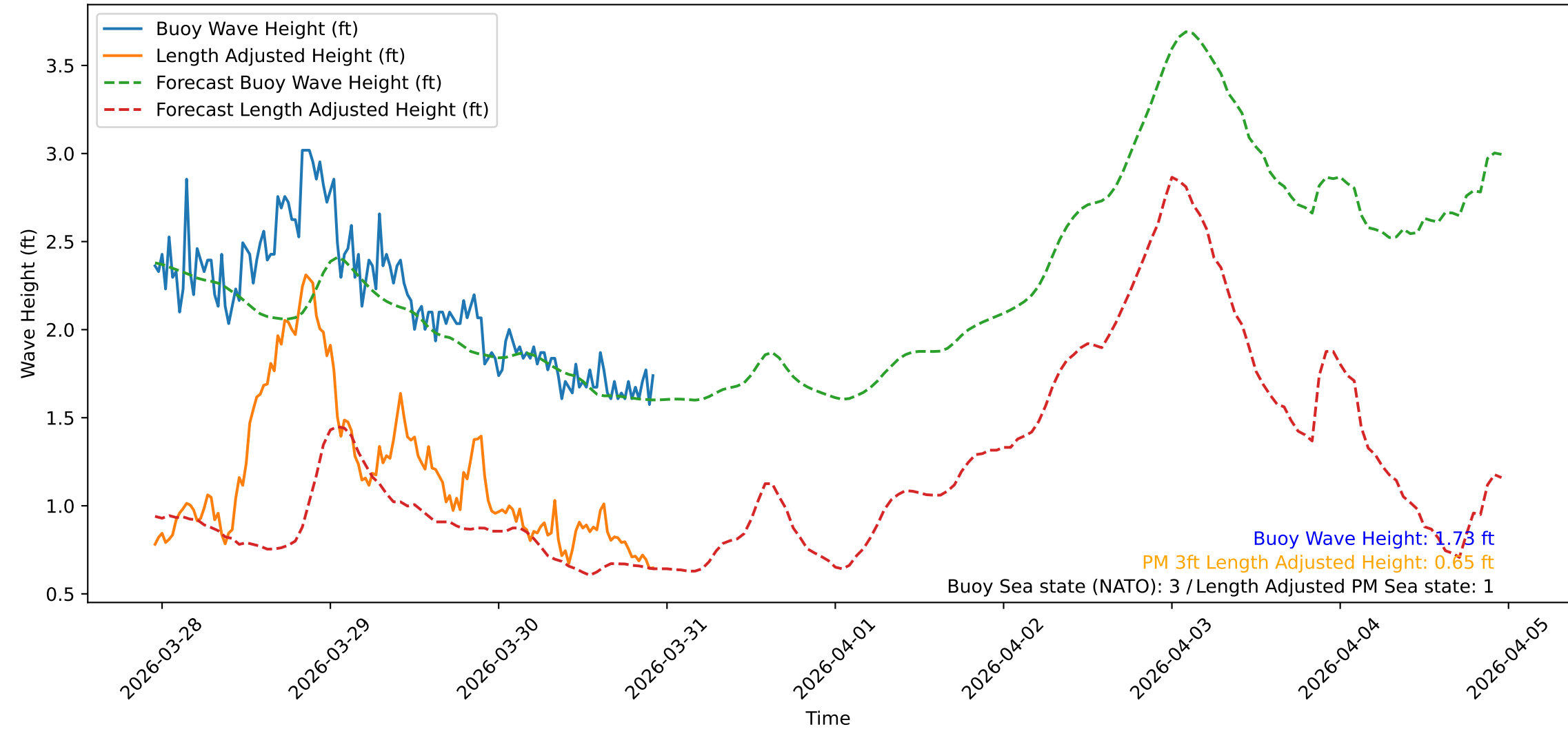
Wave Heights over Time for Red Beach at 2026-03-30 22:50:47
