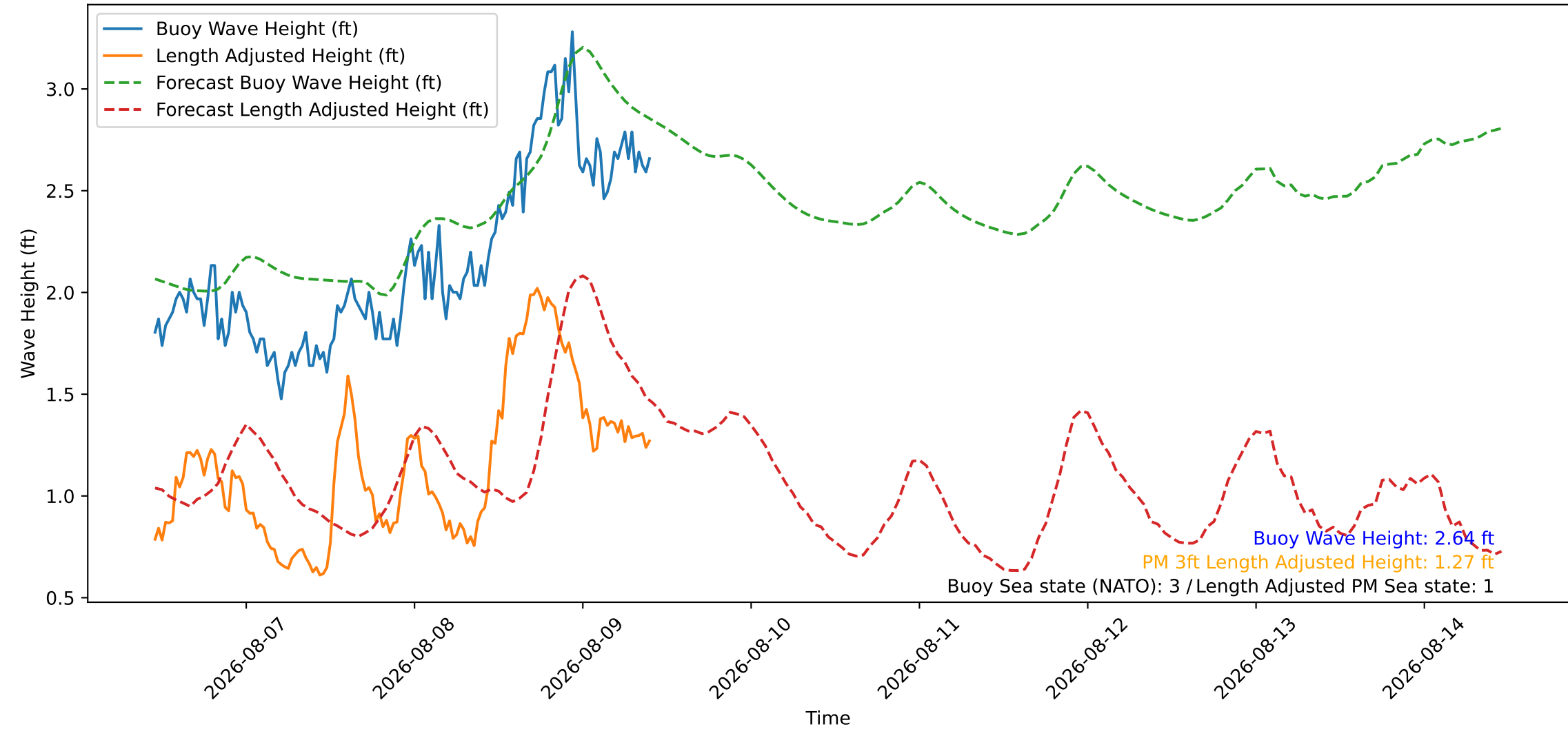
Wave Heights over Time for Red Beach at 2026-08-09 10:40:46
