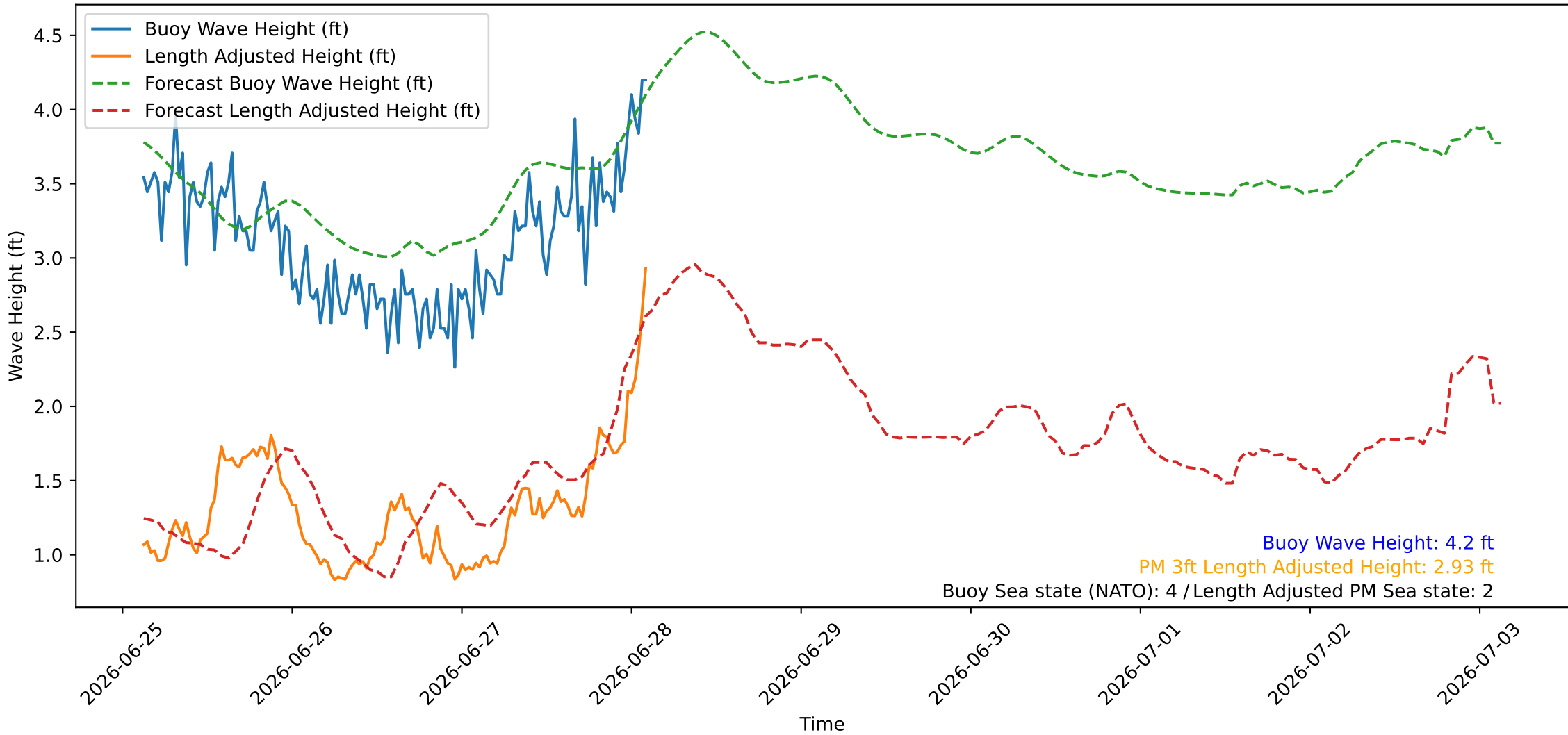
Wave Heights over Time for Green Beach at 2026-06-28 03:01:07
