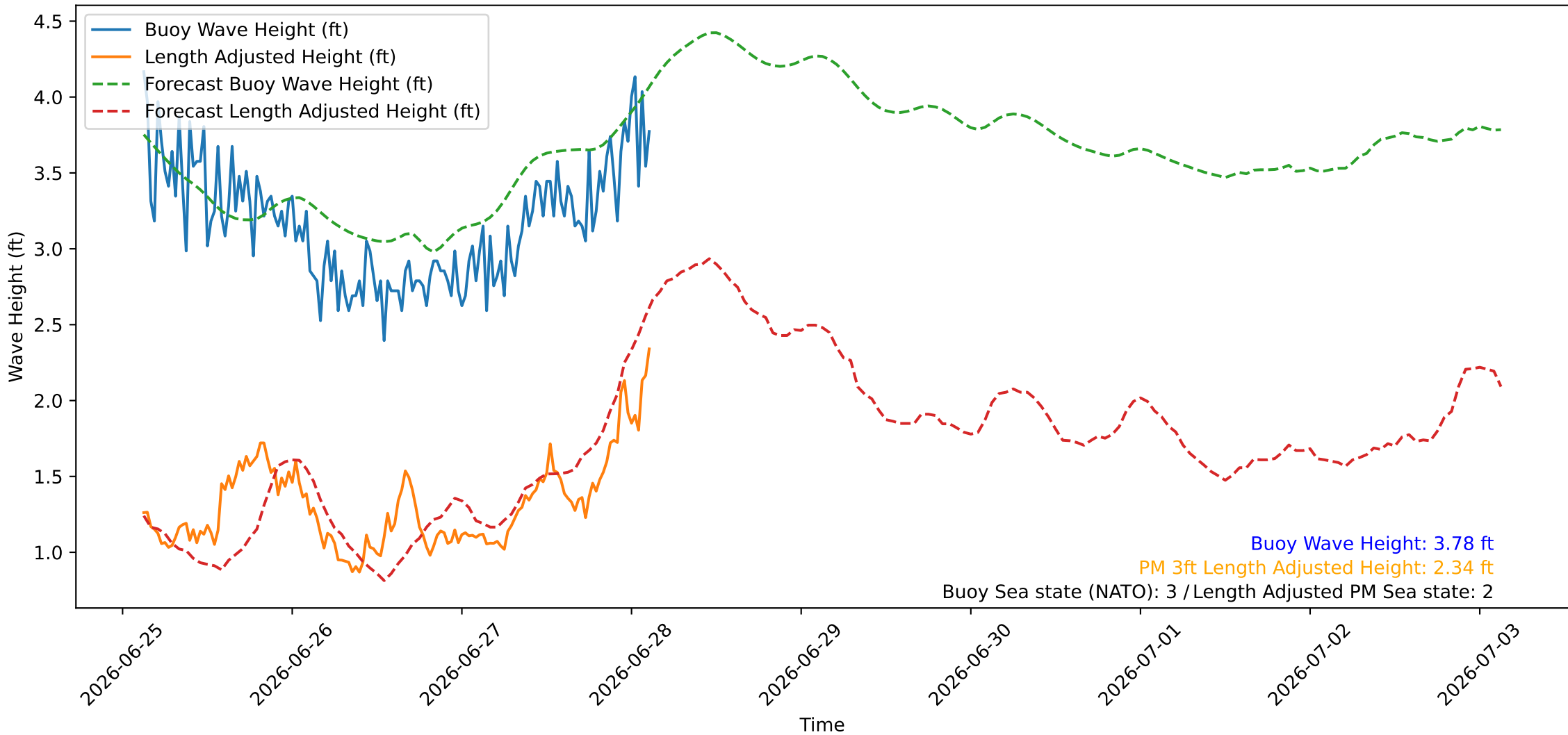
Wave Heights over Time for Oceanside Harbor at 2026-06-28 03:00:25
