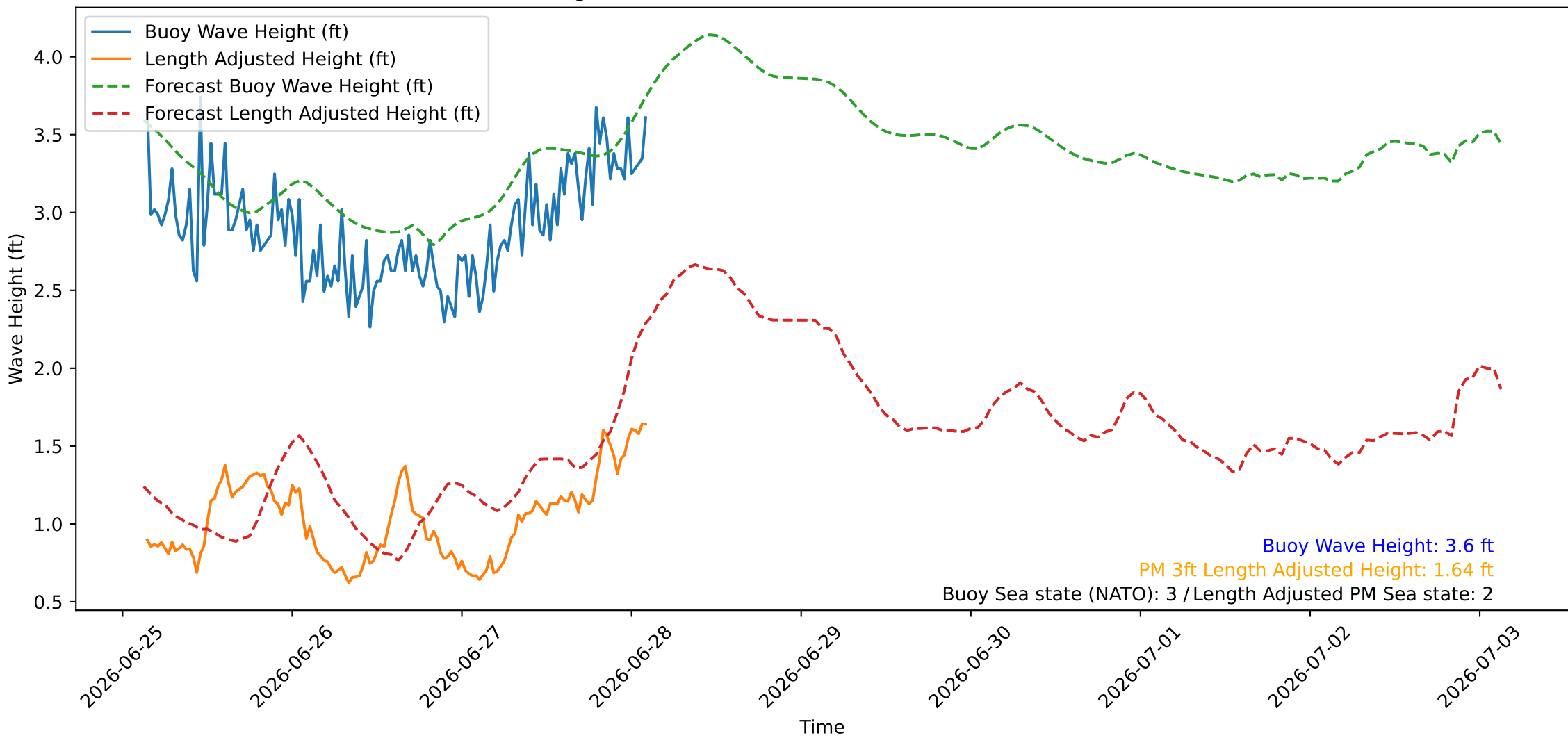
Wave Heights over Time for Red Beach at 2026-06-28 03:00:44
