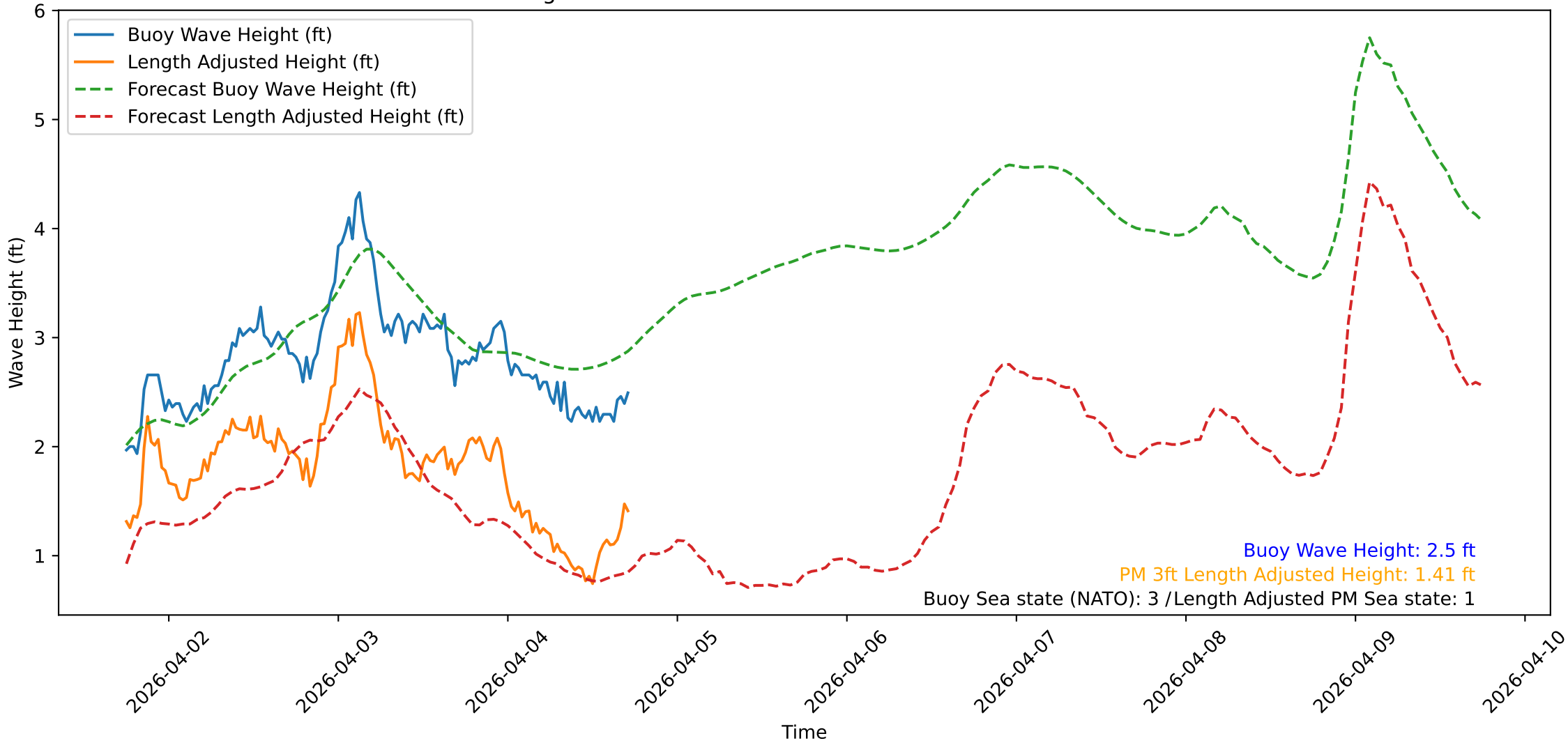
Wave Heights over Time for Green Beach at 2026-04-04 17:51:15
