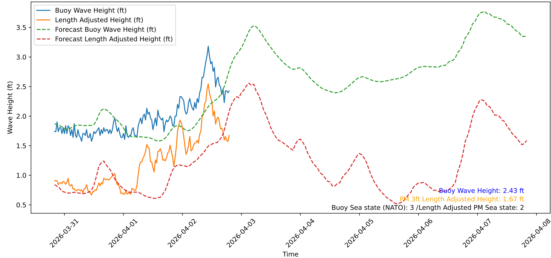
Wave Heights over Time for Oceanside Harbor at 2026-04-02 19:50:31
