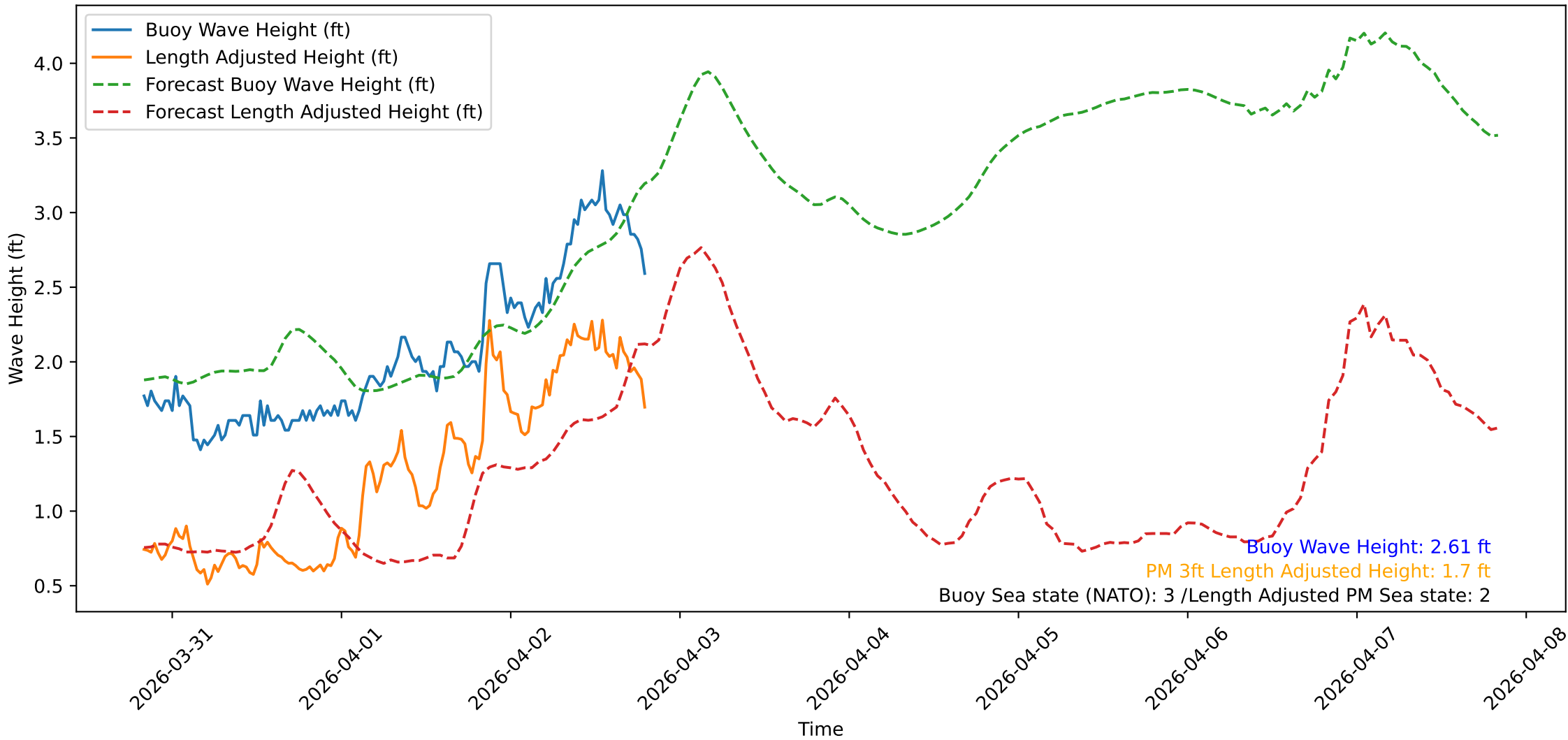
Wave Heights over Time for Green Beach at 2026-04-02 19:51:10
