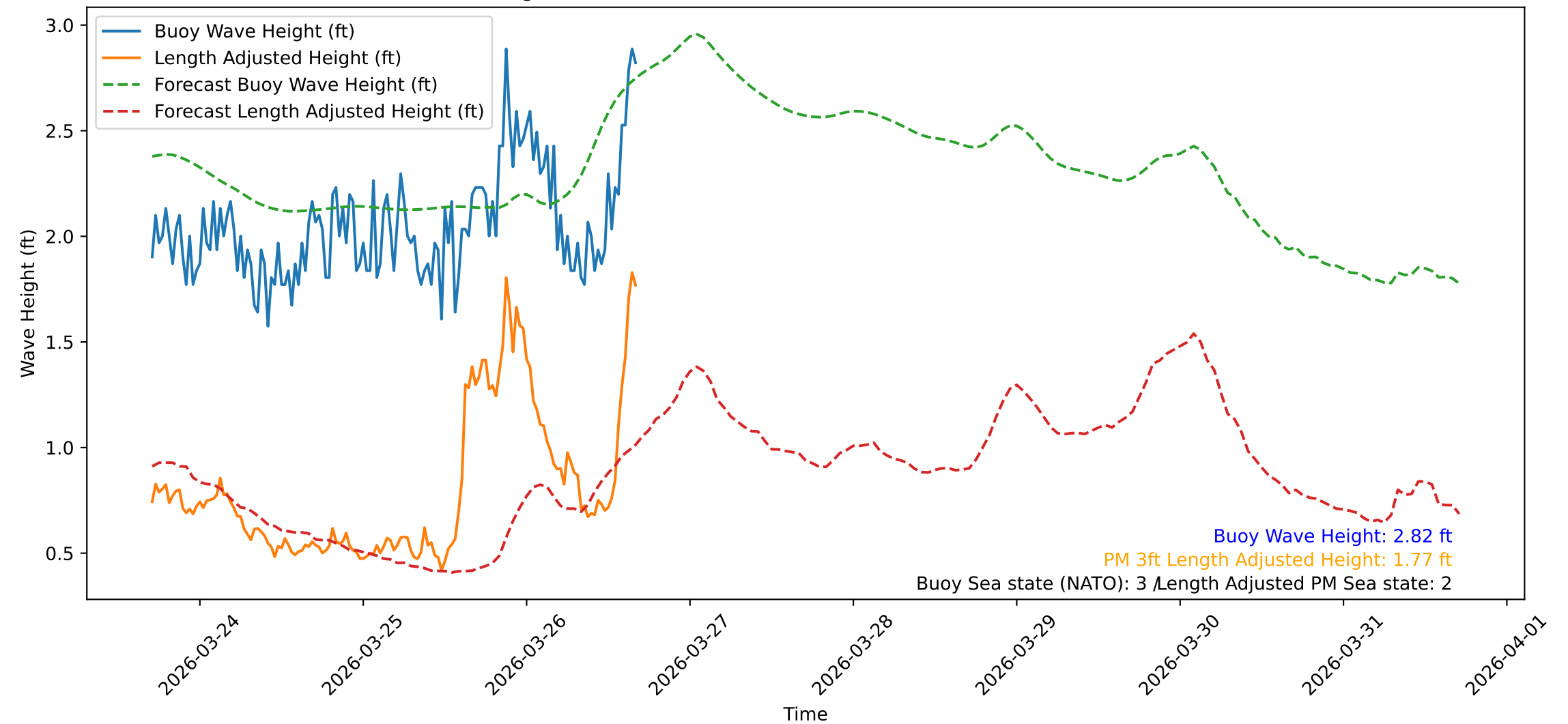
Wave Heights over Time for Oceanside Harbor at 2026-03-26 17:10:31
