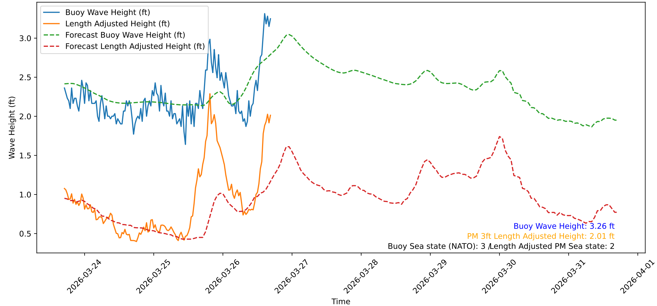
Wave Heights over Time for Green Beach at 2026-03-26 17:11:09
