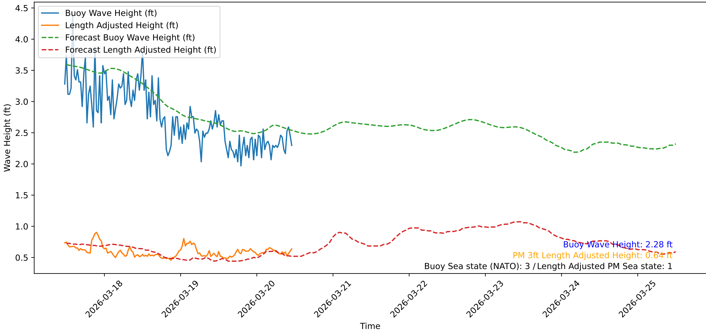
Wave Heights over Time for Oceanside Harbor at 2026-03-20 11:30:32
