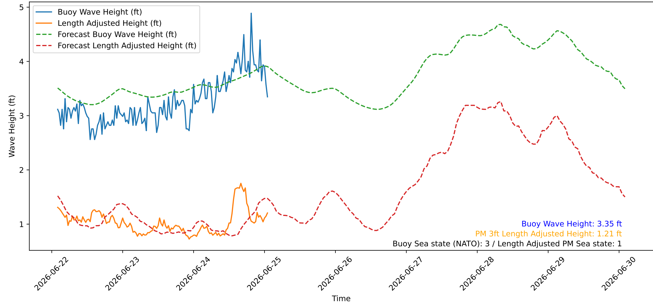
Wave Heights over Time for Oceanside Harbor at 2026-06-25 02:00:26
