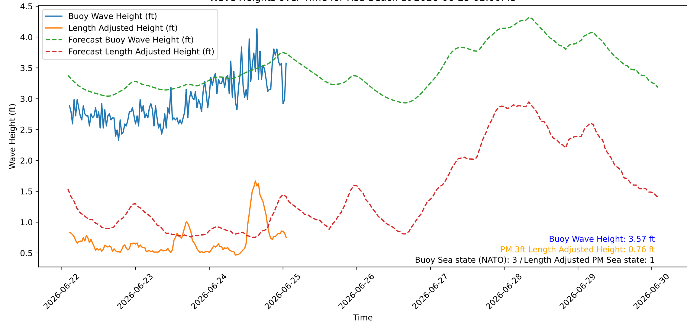
Wave Heights over Time for Red Beach at 2026-06-25 02:00:45
