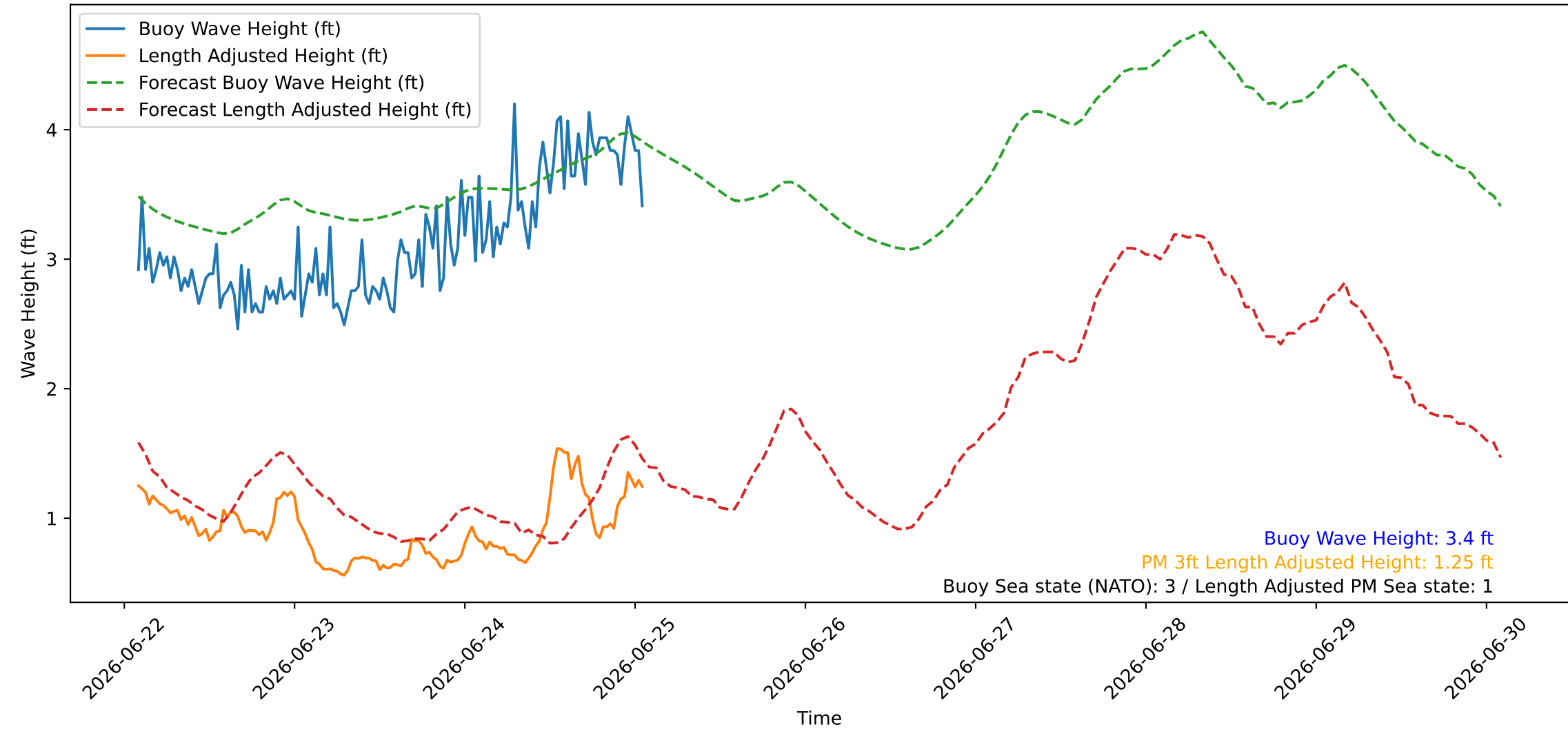
Wave Heights over Time for Green Beach at 2026-06-25 02:01:07
