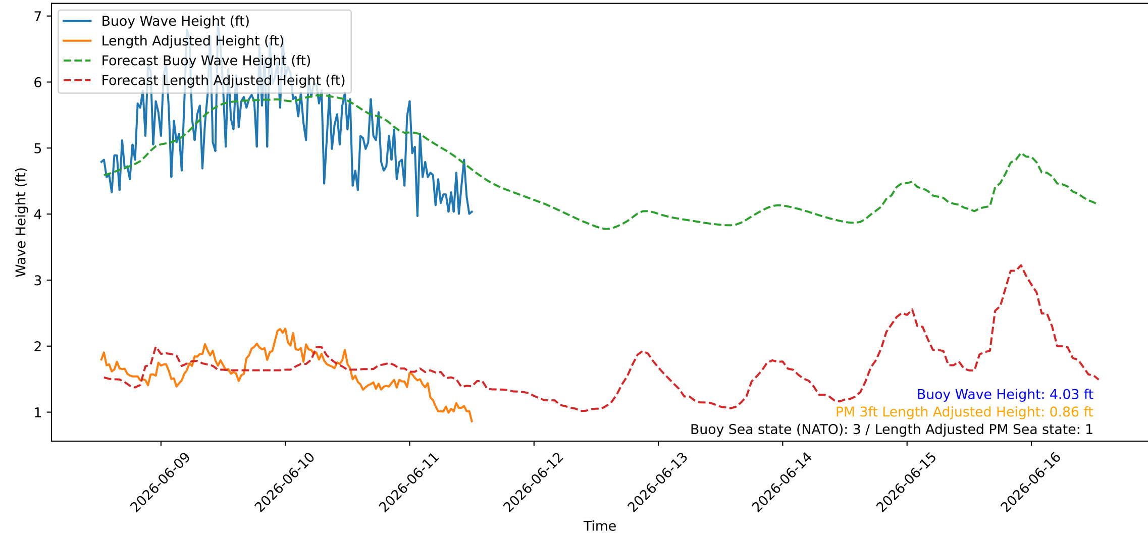
Wave Heights over Time for Green Beach at 2026-06-11 12:41:09
