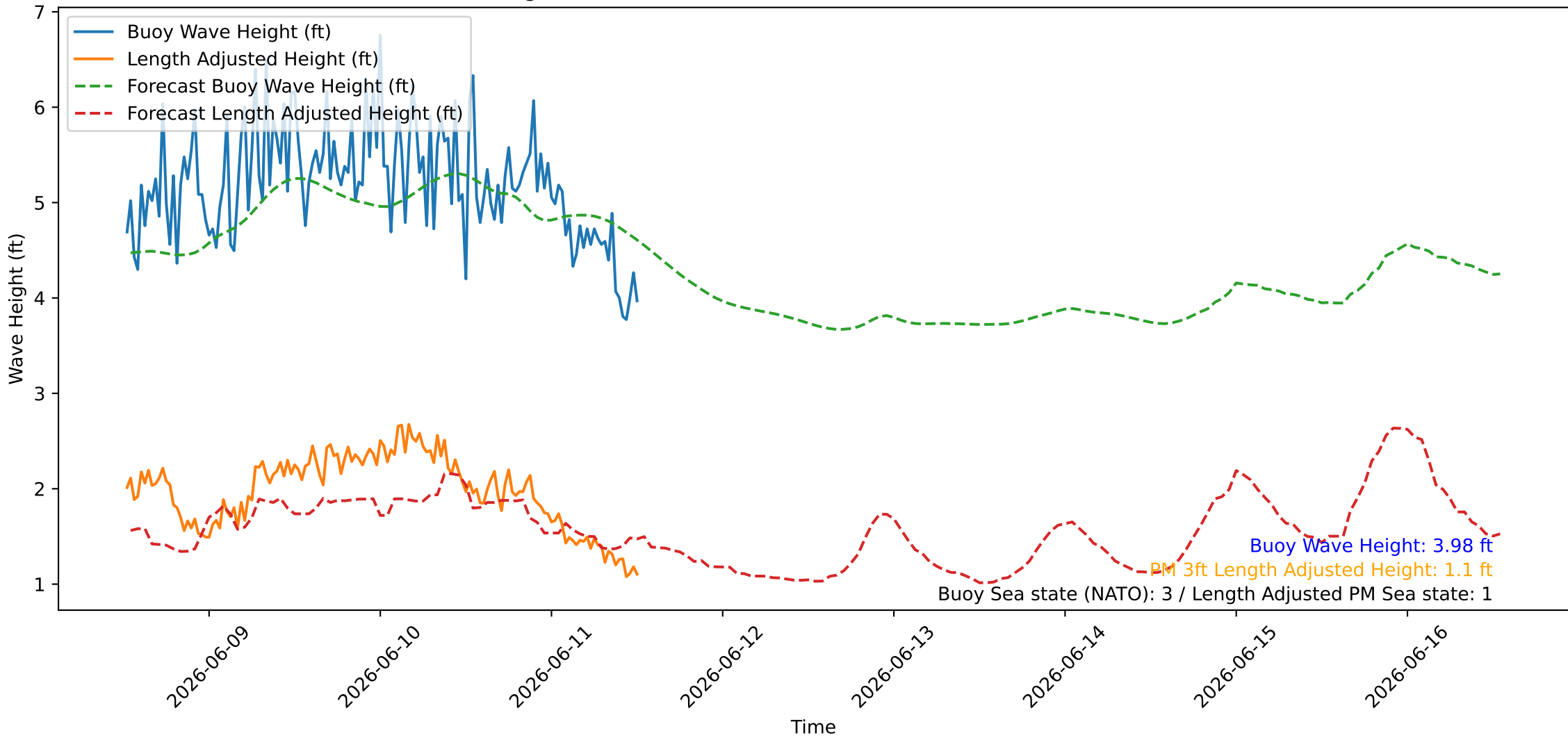
Wave Heights over Time for Oceanside Harbor at 2026-06-11 12:40:26
