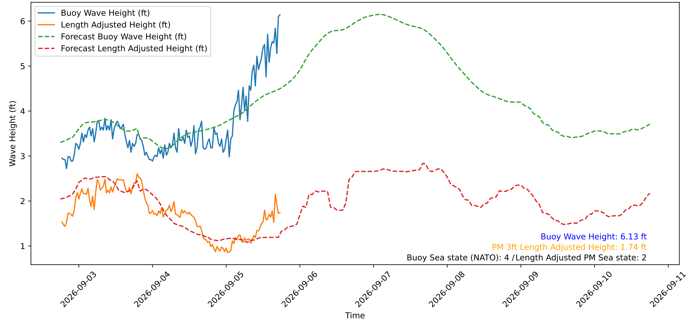
Wave Heights over Time for Oceanside Harbor at 2026-09-05 18:20:29
