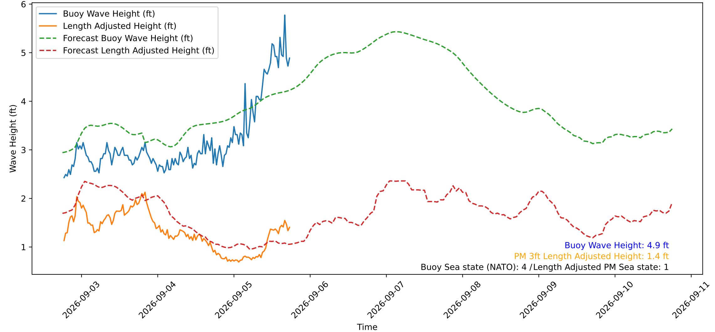
Wave Heights over Time for Red Beach at 2026-09-05 18:20:50
