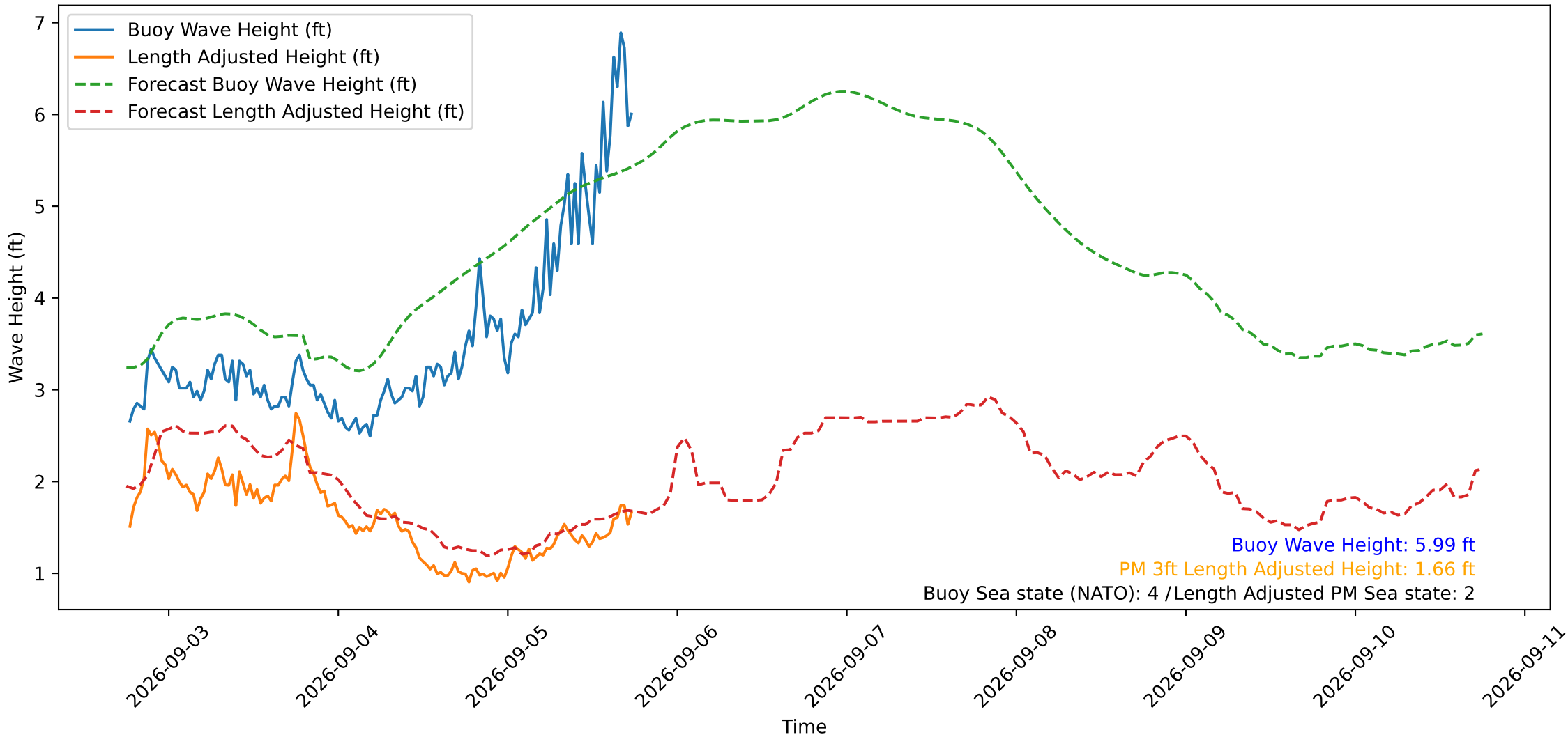
Wave Heights over Time for Green Beach at 2026-09-05 18:21:14
