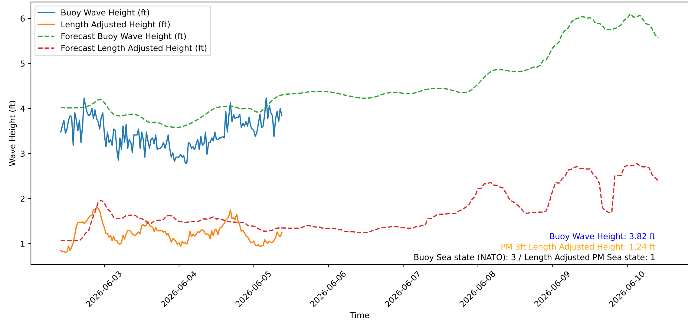
Wave Heights over Time for Green Beach at 2026-06-05 10:01:08
