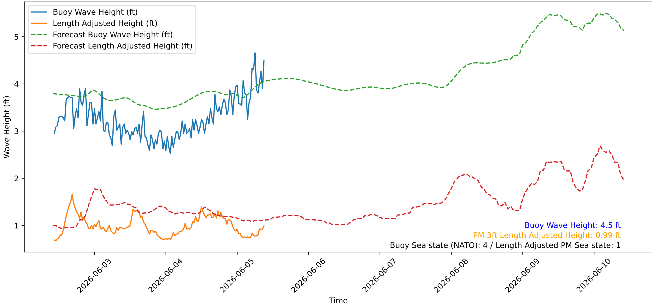
Wave Heights over Time for Red Beach at 2026-06-05 10:00:46
