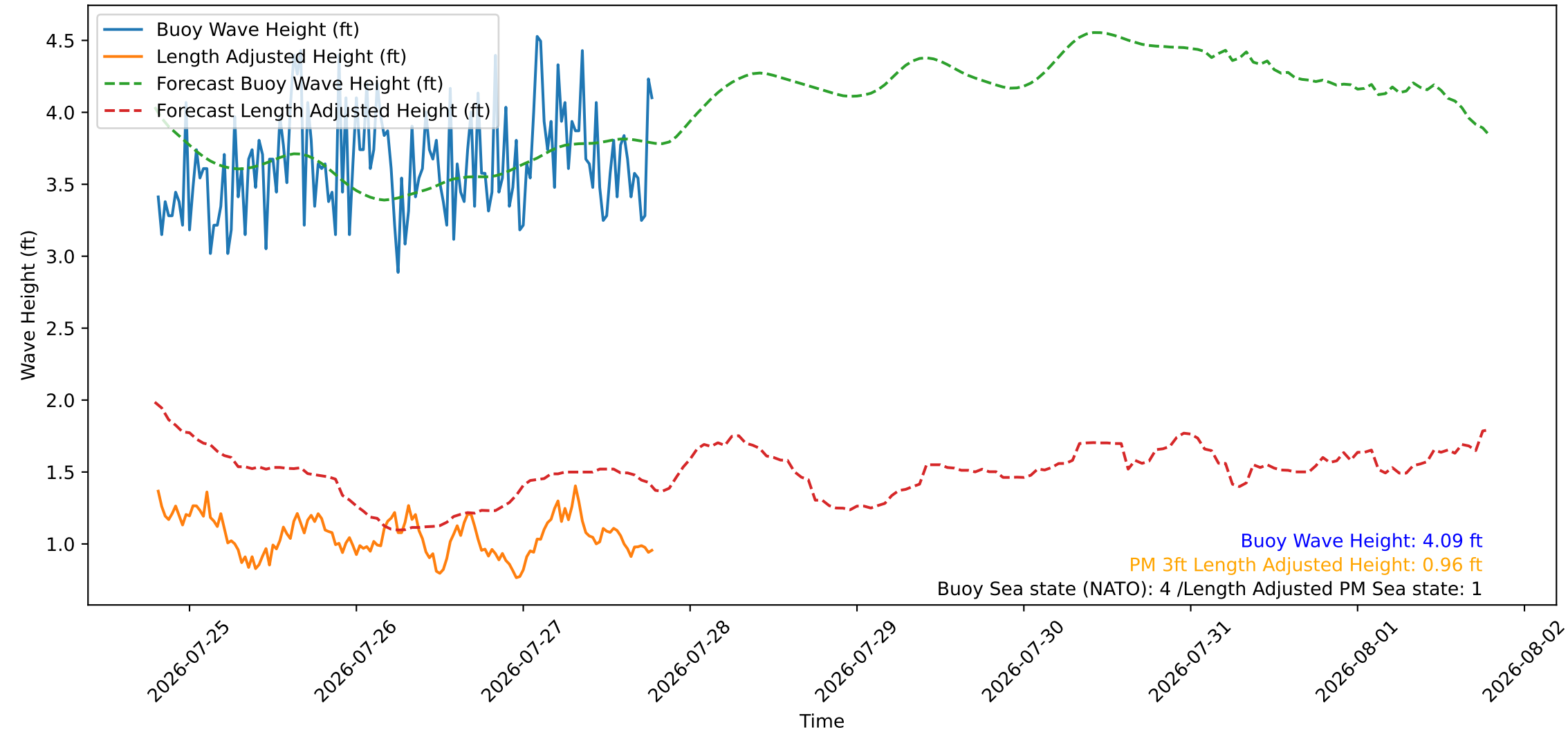
Wave Heights over Time for Red Beach at 2026-07-27 19:20:48
