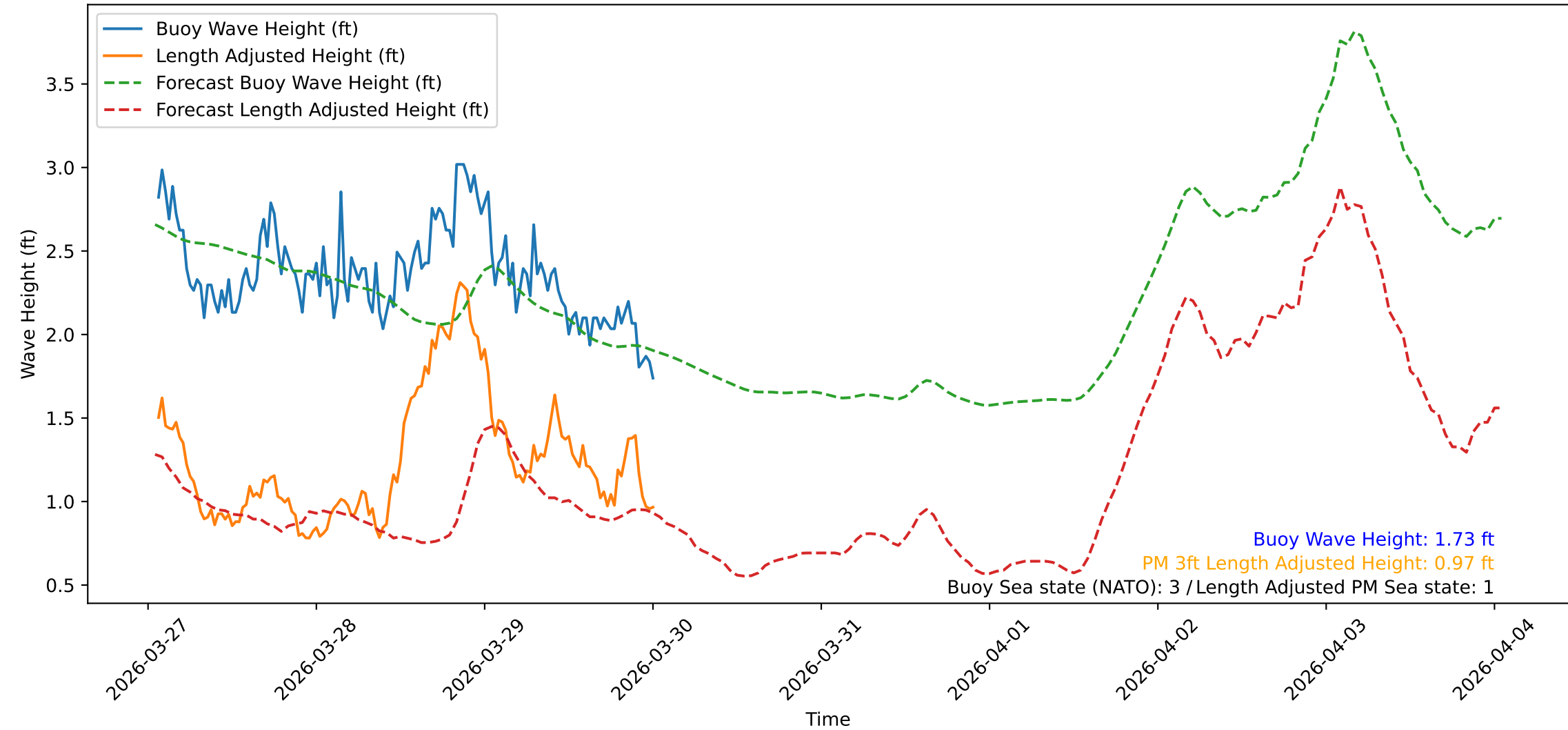
Wave Heights over Time for Red Beach at 2026-03-30 01:00:47
