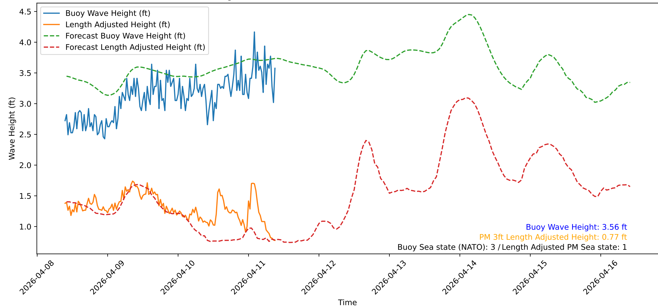
Wave Heights over Time for Oceanside Harbor at 2026-04-11 09:30:31
