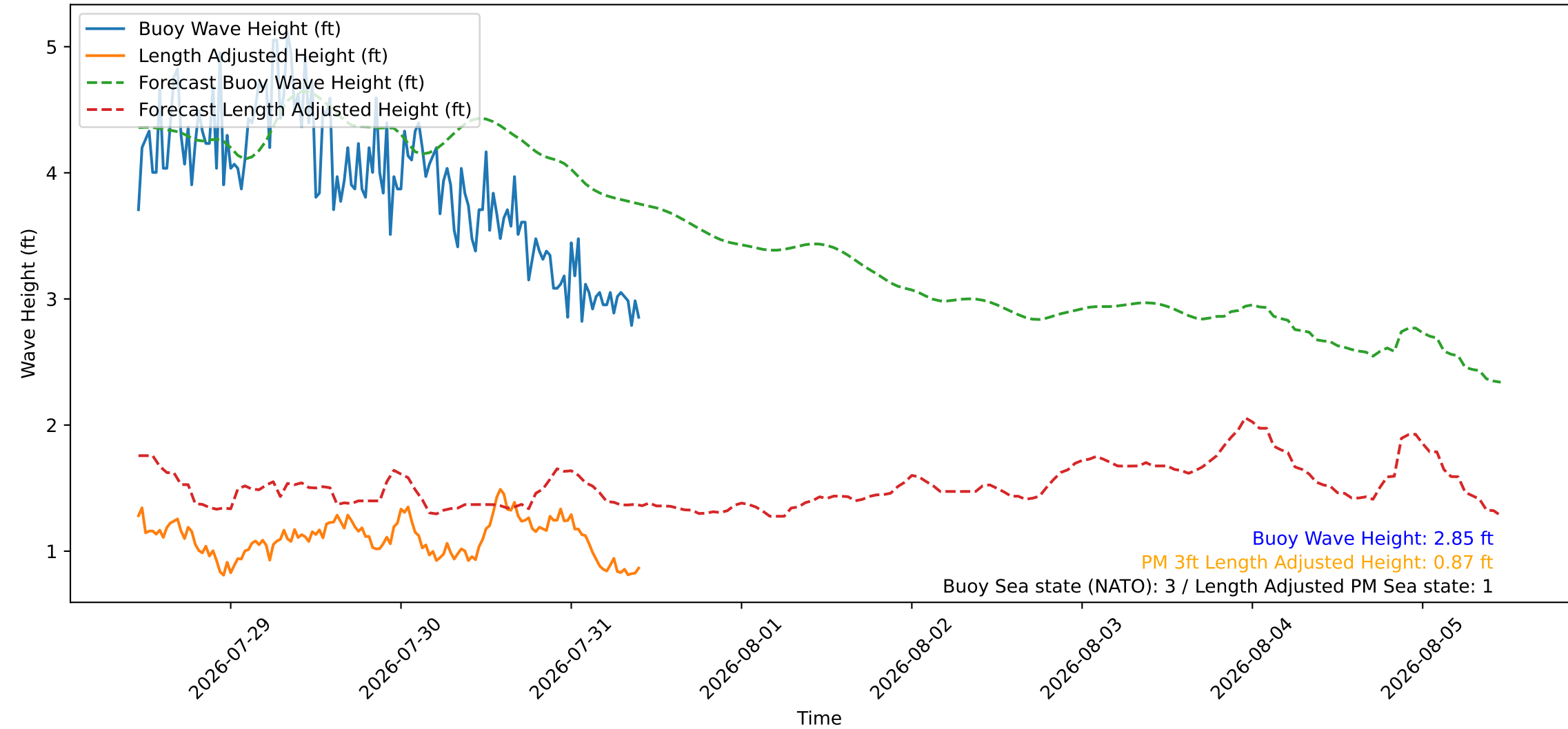
Wave Heights over Time for Red Beach at 2026-07-31 10:40:46
