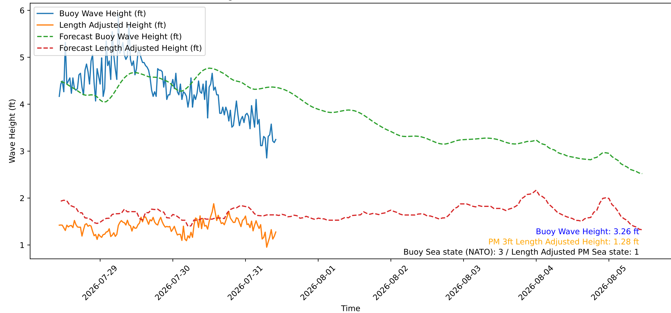
Wave Heights over Time for Oceanside Harbor at 2026-07-31 10:40:26
