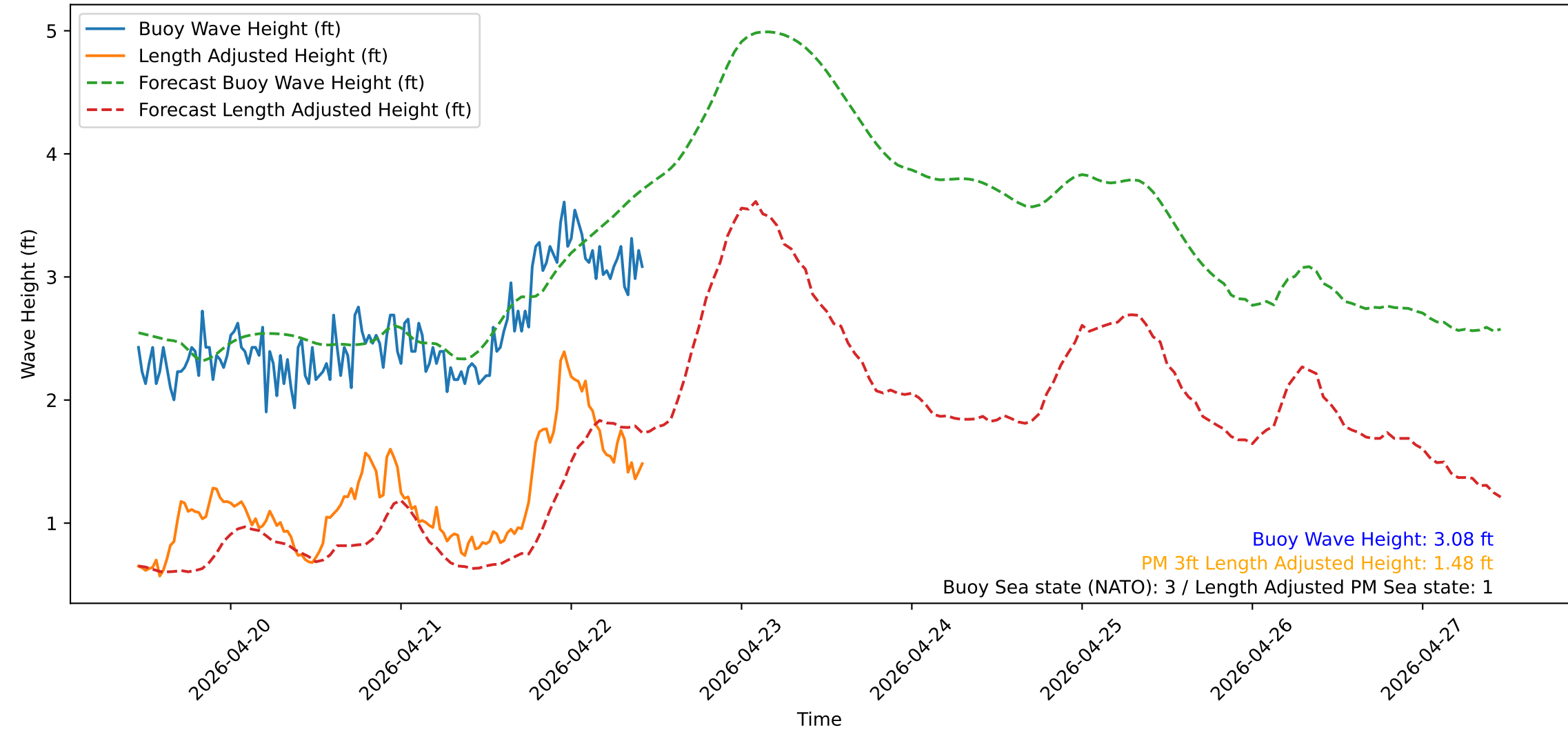
Wave Heights over Time for Oceanside Harbor at 2026-04-22 11:00:31
