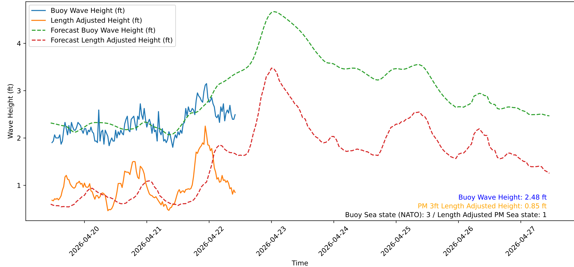
Wave Heights over Time for Red Beach at 2026-04-22 11:00:50
