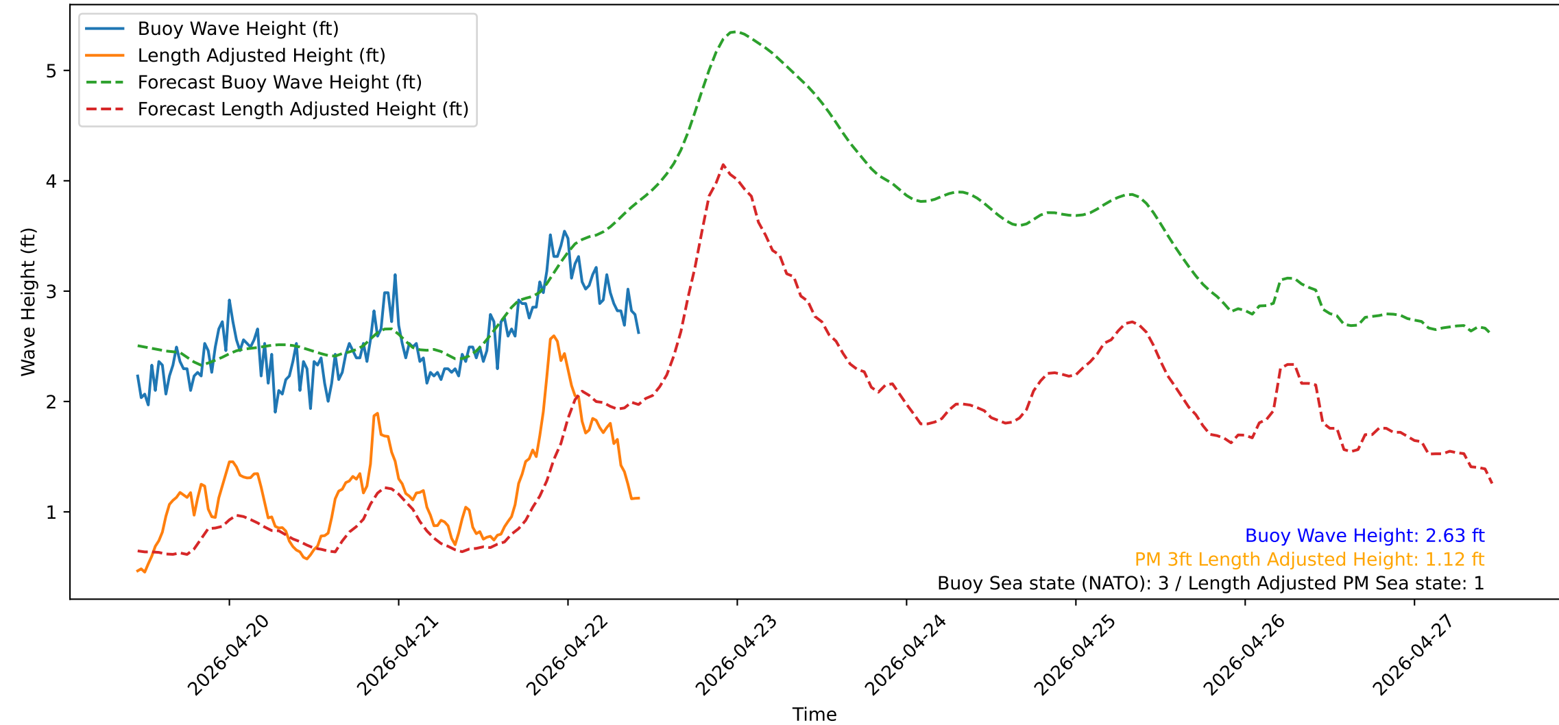
Wave Heights over Time for Green Beach at 2026-04-22 11:01:12
