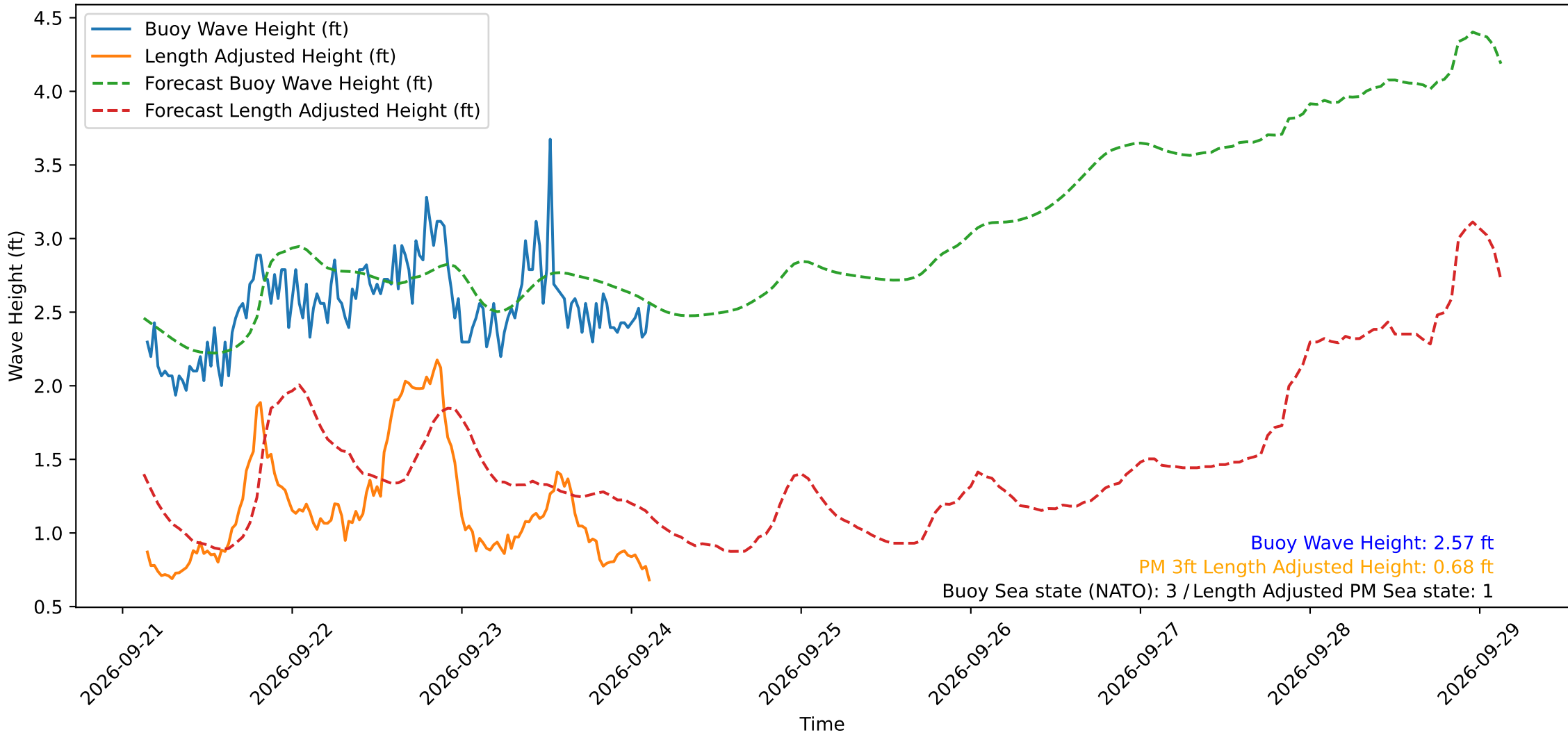
Wave Heights over Time for Red Beach at 2026-09-24 03:10:50
