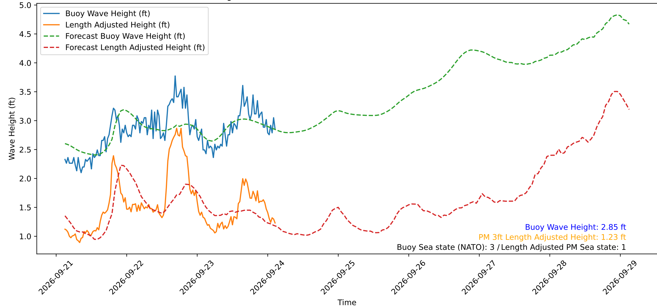
Wave Heights over Time for Oceanside Harbor at 2026-09-24 03:10:29
