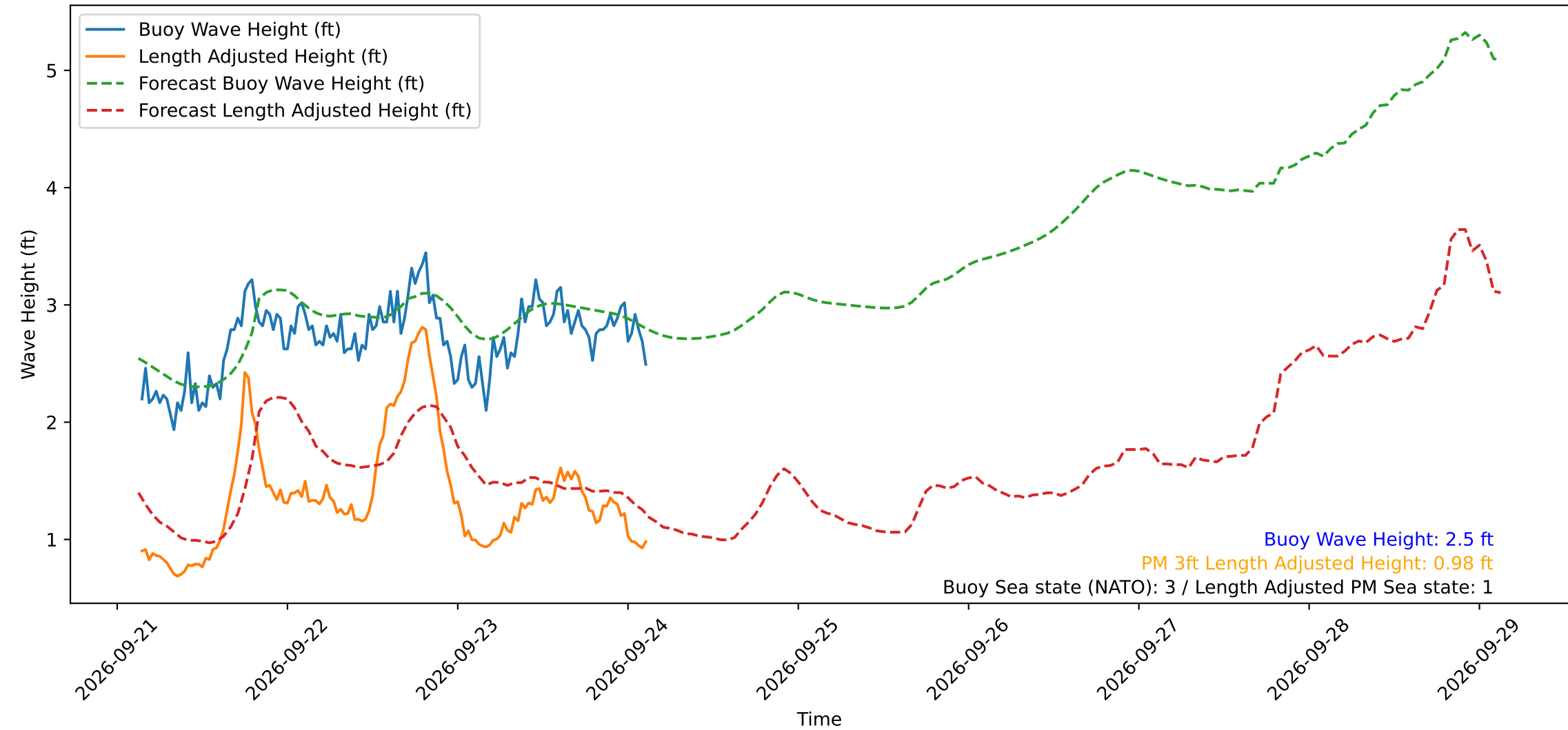
Wave Heights over Time for Green Beach at 2026-09-24 03:11:12
