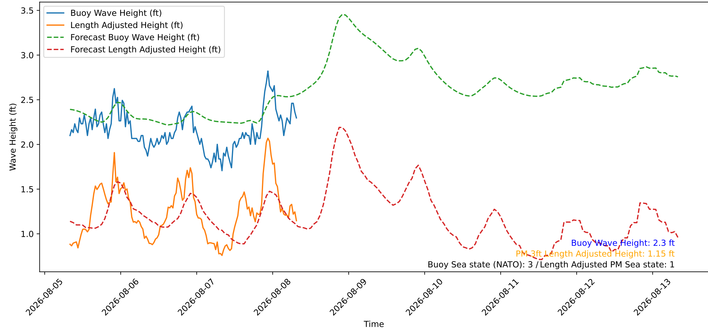
Wave Heights over Time for Green Beach at 2026-08-08 08:11:08
