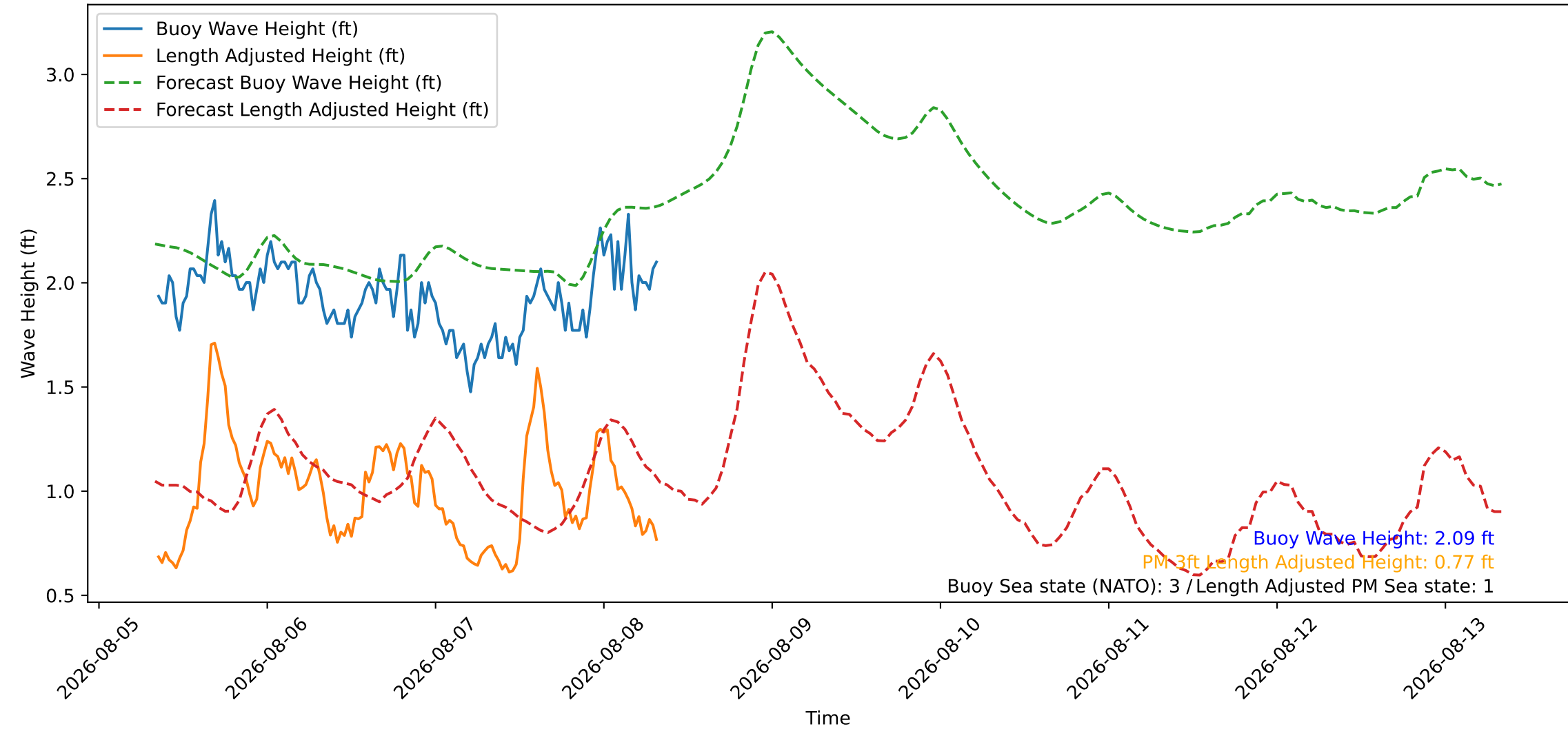
Wave Heights over Time for Red Beach at 2026-08-08 08:10:45
