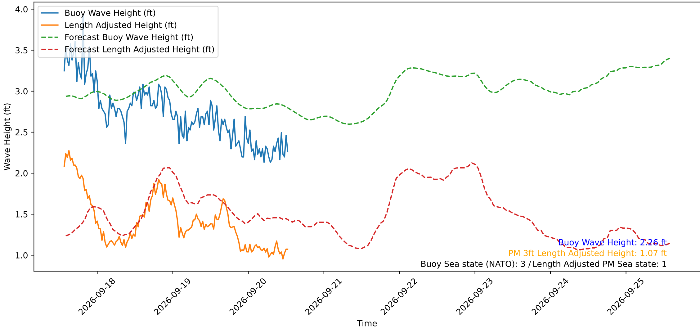
Wave Heights over Time for Oceanside Harbor at 2026-09-20 13:30:29
