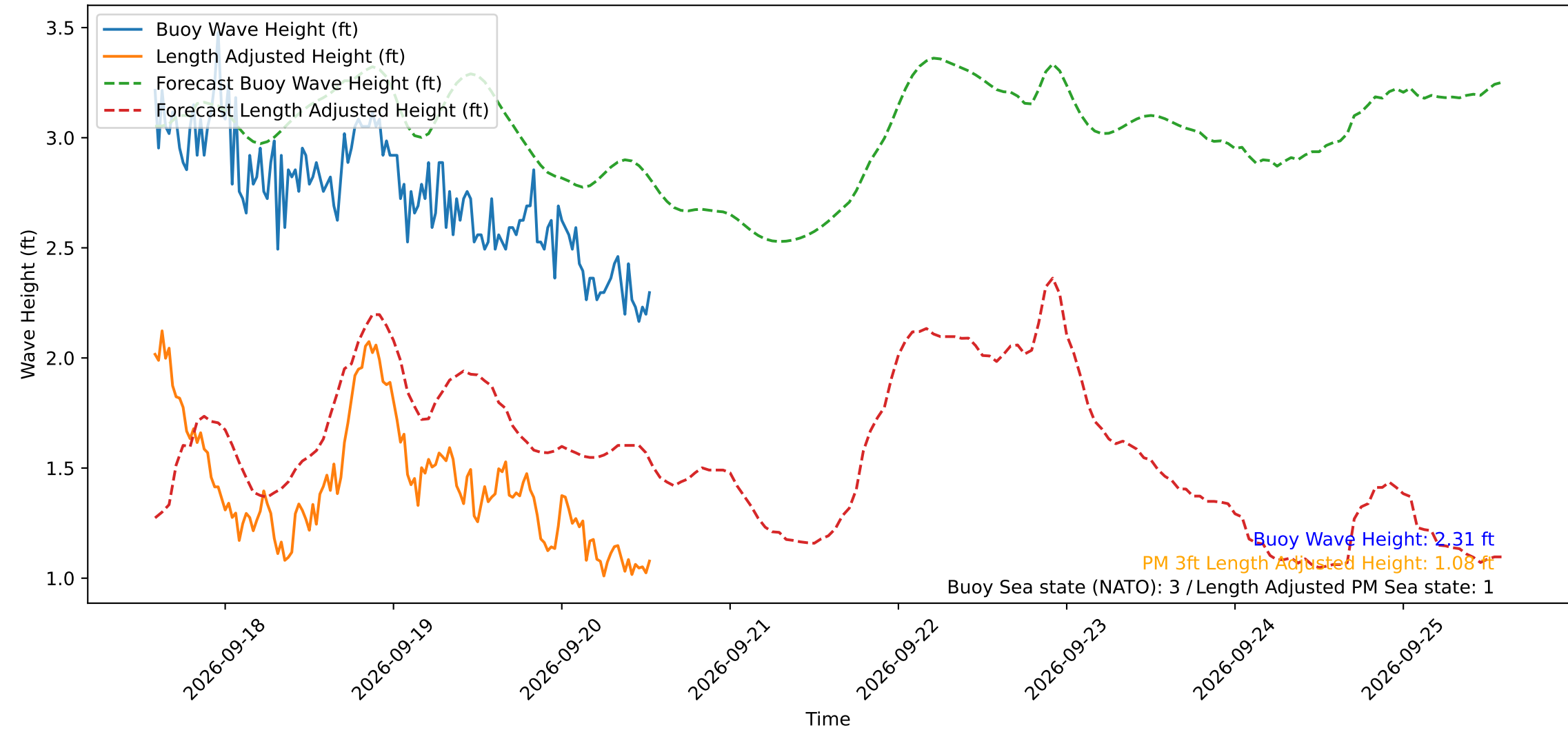
Wave Heights over Time for Green Beach at 2026-09-20 13:31:12
