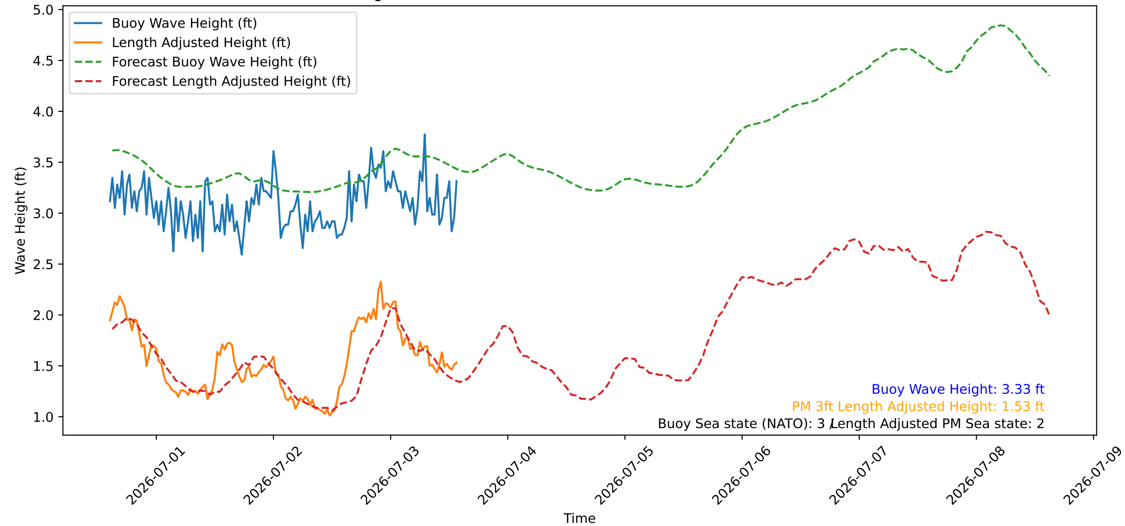
Wave Heights over Time for Oceanside Harbor at 2026-07-03 14:30:26
