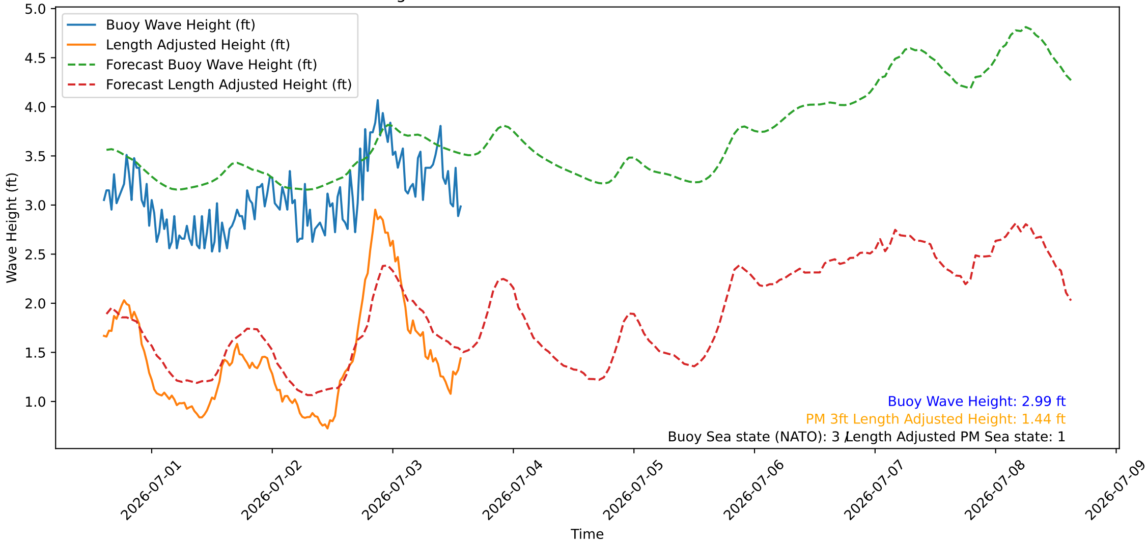
Wave Heights over Time for Green Beach at 2026-07-03 14:31:08
