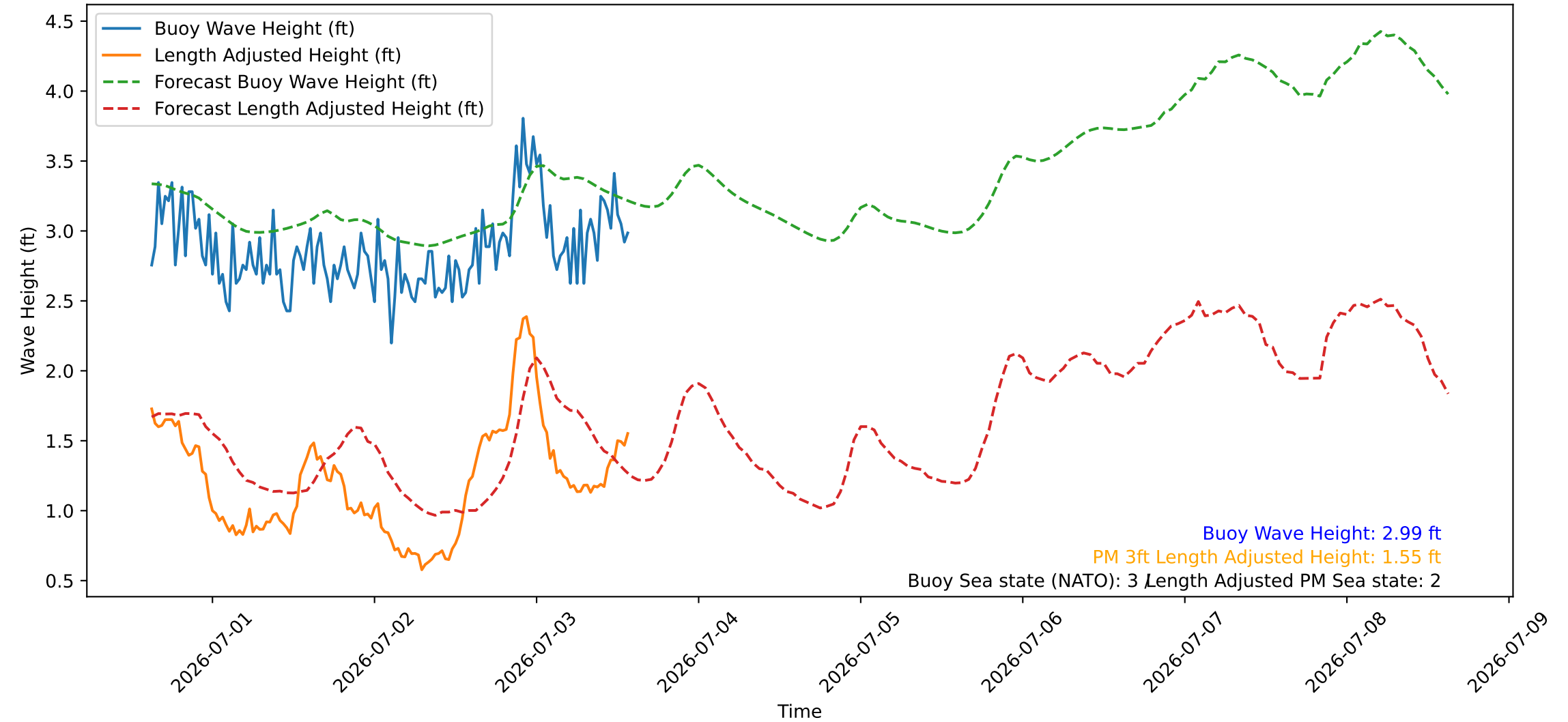
Wave Heights over Time for Red Beach at 2026-07-03 14:30:46
