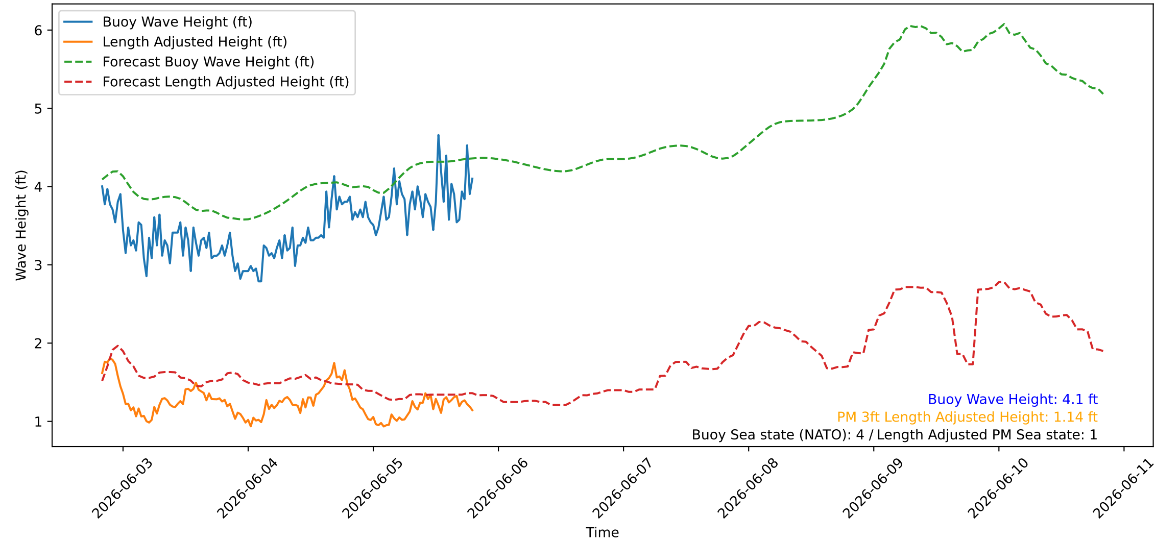
Wave Heights over Time for Green Beach at 2026-06-05 19:51:09
