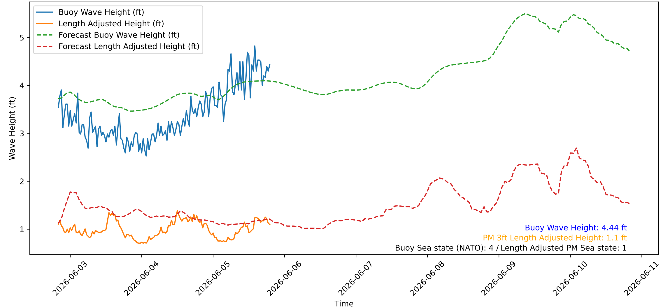
Wave Heights over Time for Red Beach at 2026-06-05 19:50:46
