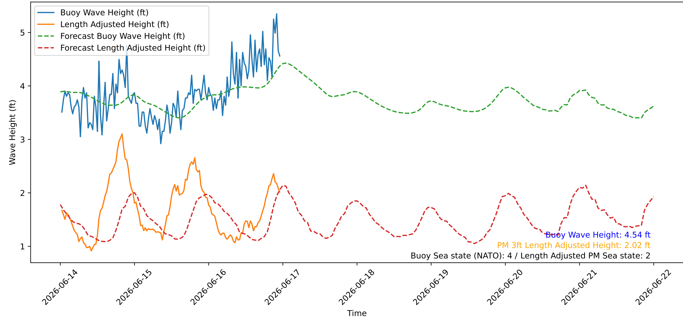
Wave Heights over Time for Red Beach at 2026-06-17 00:00:45
