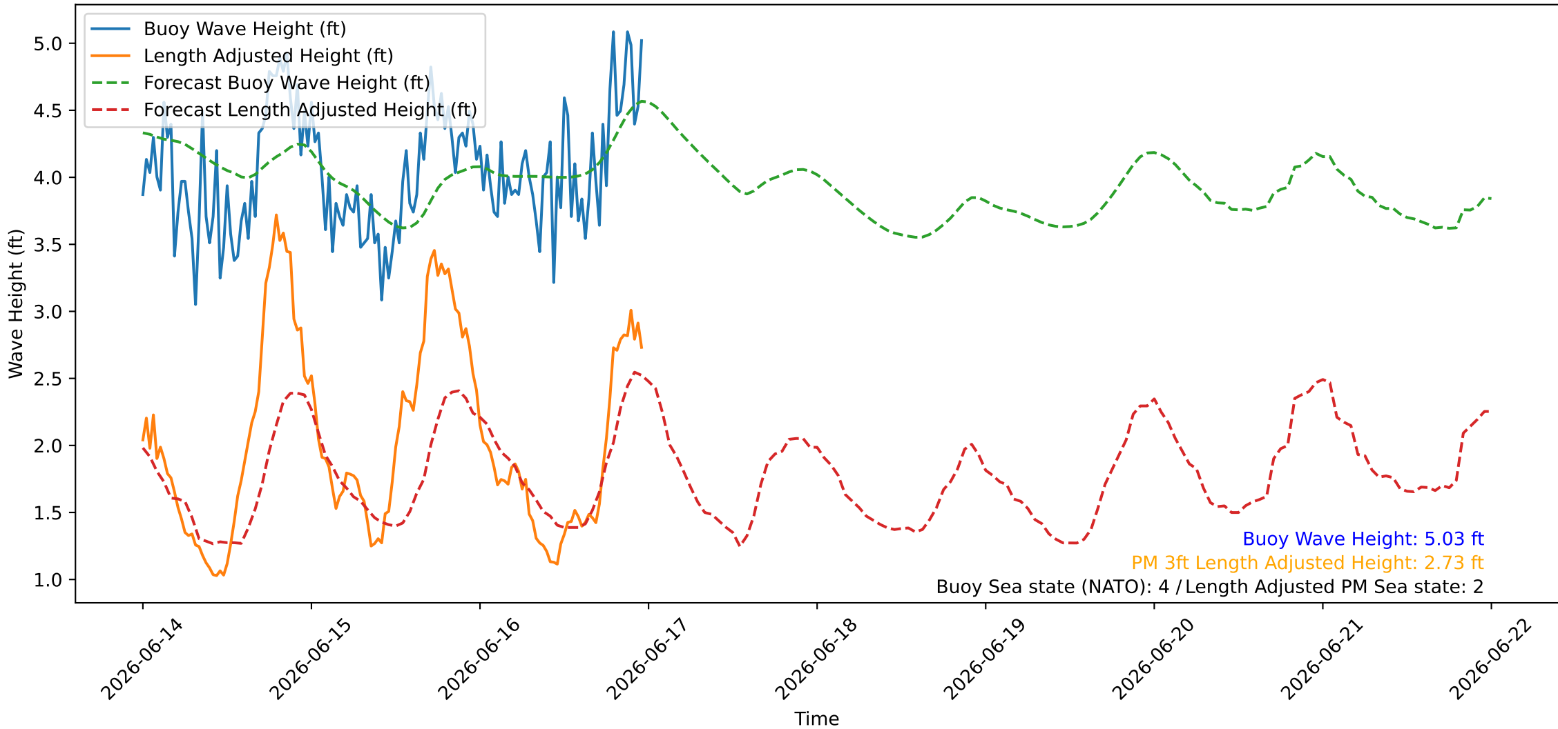
Wave Heights over Time for Green Beach at 2026-06-17 00:01:07
