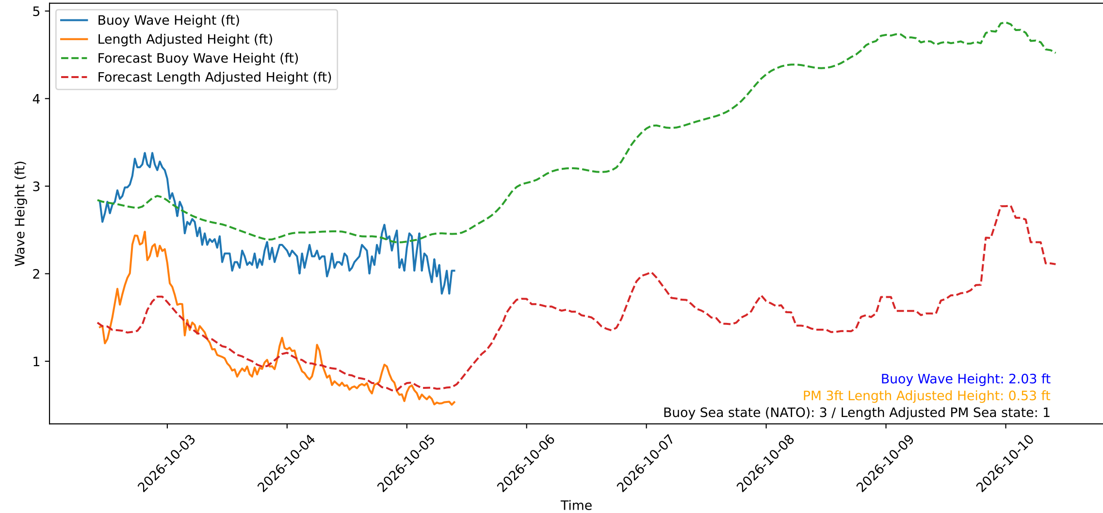
Wave Heights over Time for Green Beach at 2026-10-05 10:11:11
