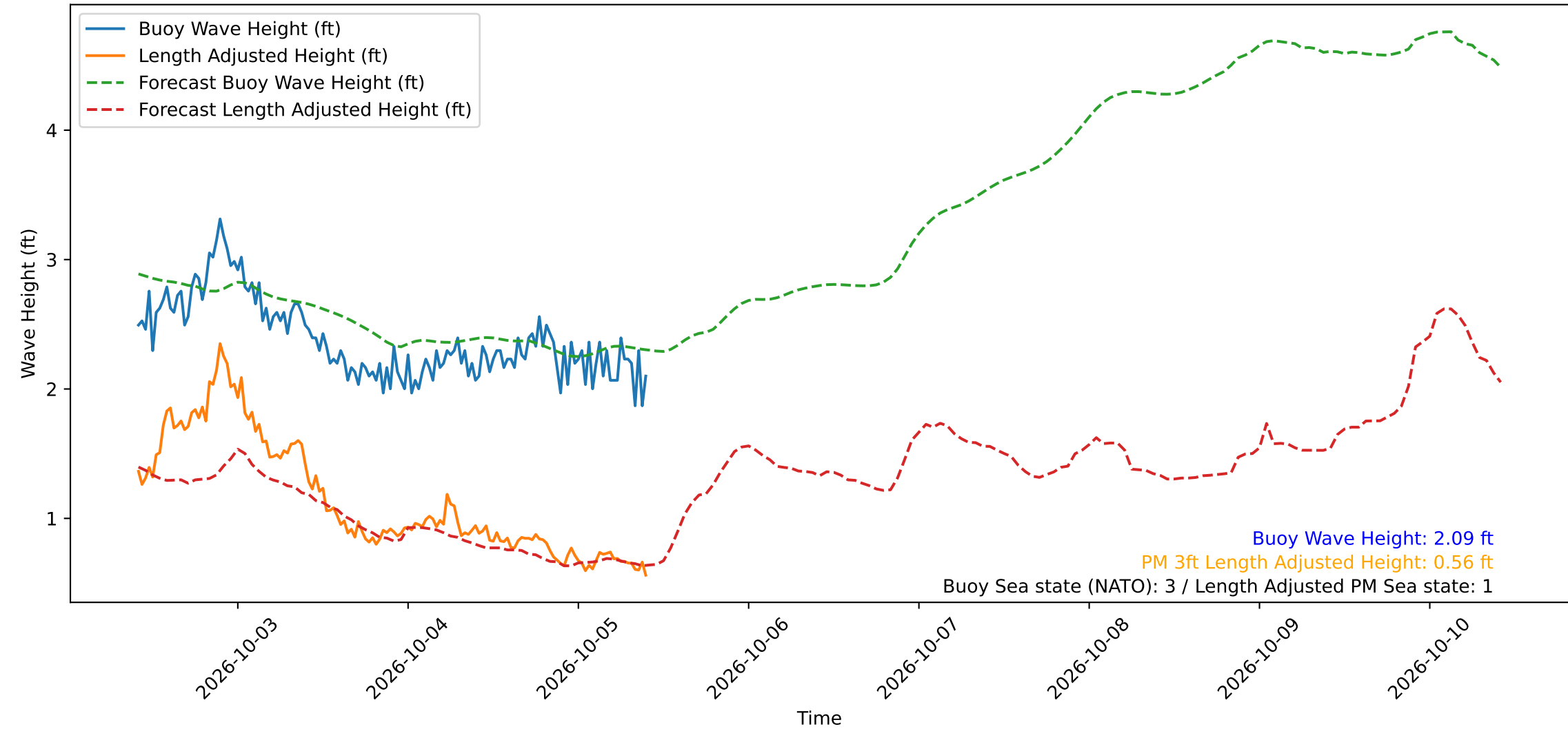
Wave Heights over Time for Oceanside Harbor at 2026-10-05 10:10:29
