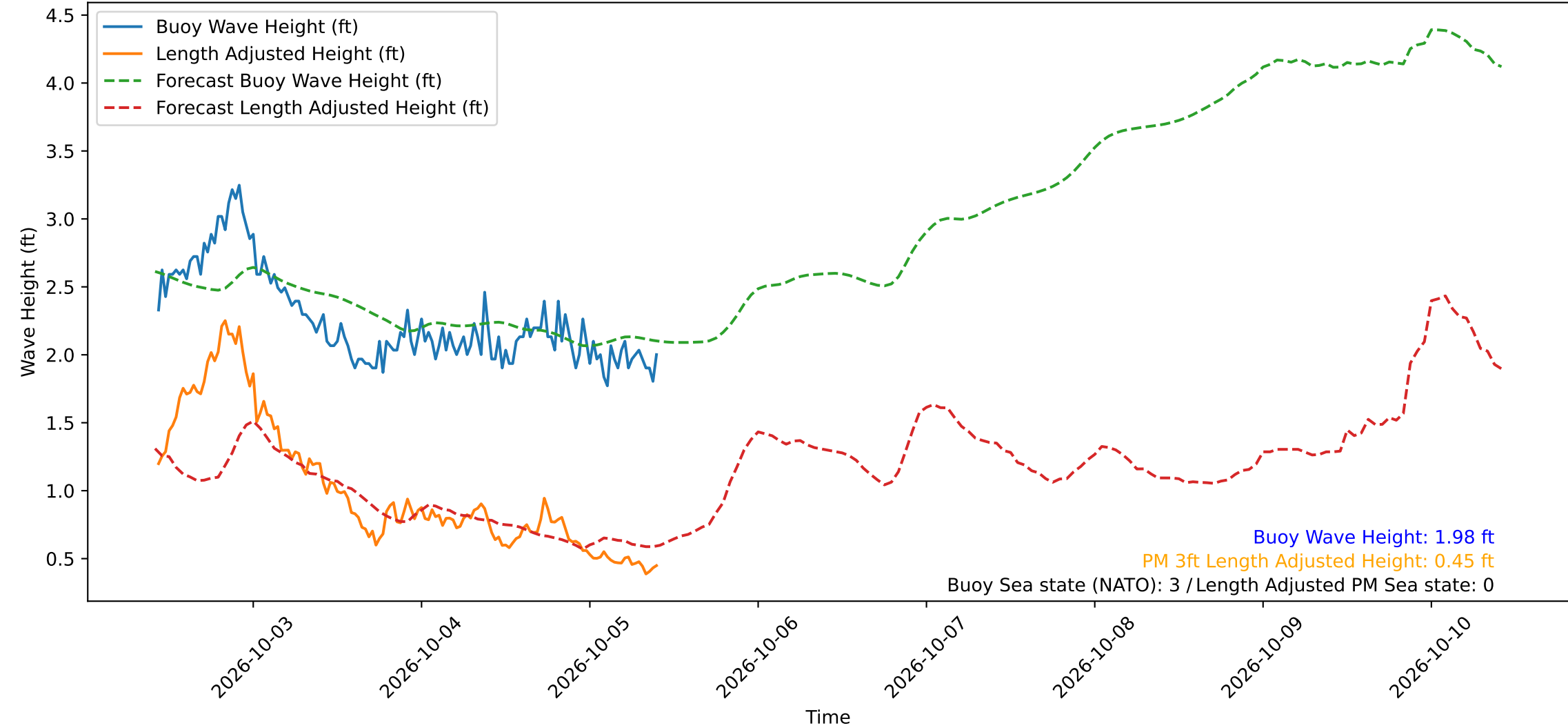
Wave Heights over Time for Red Beach at 2026-10-05 10:10:48
