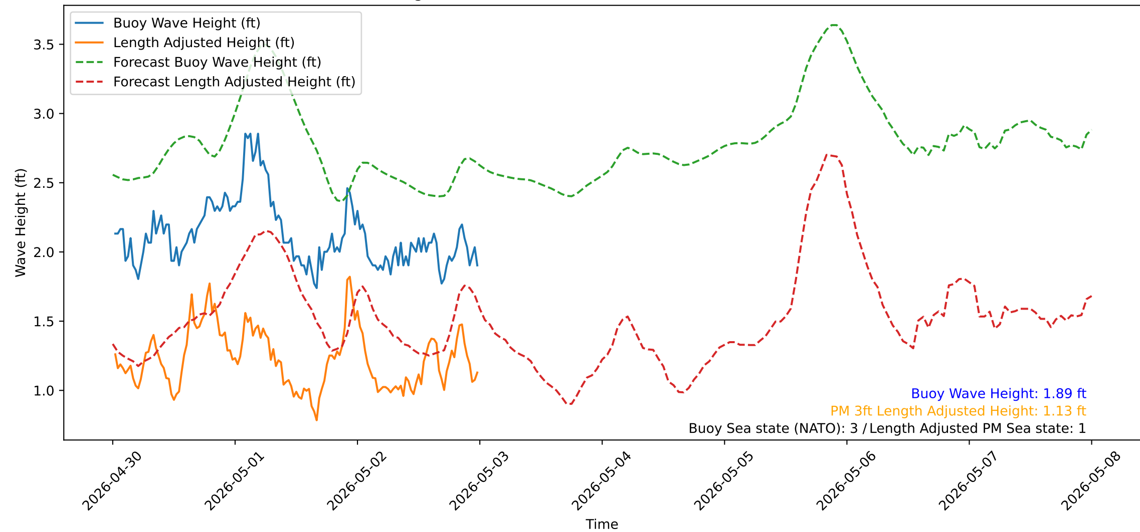
Wave Heights over Time for Green Beach at 2026-05-03 00:21:13
