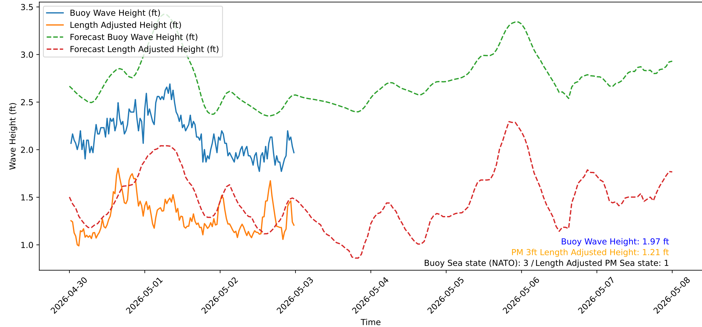
Wave Heights over Time for Oceanside Harbor at 2026-05-03 00:20:31
