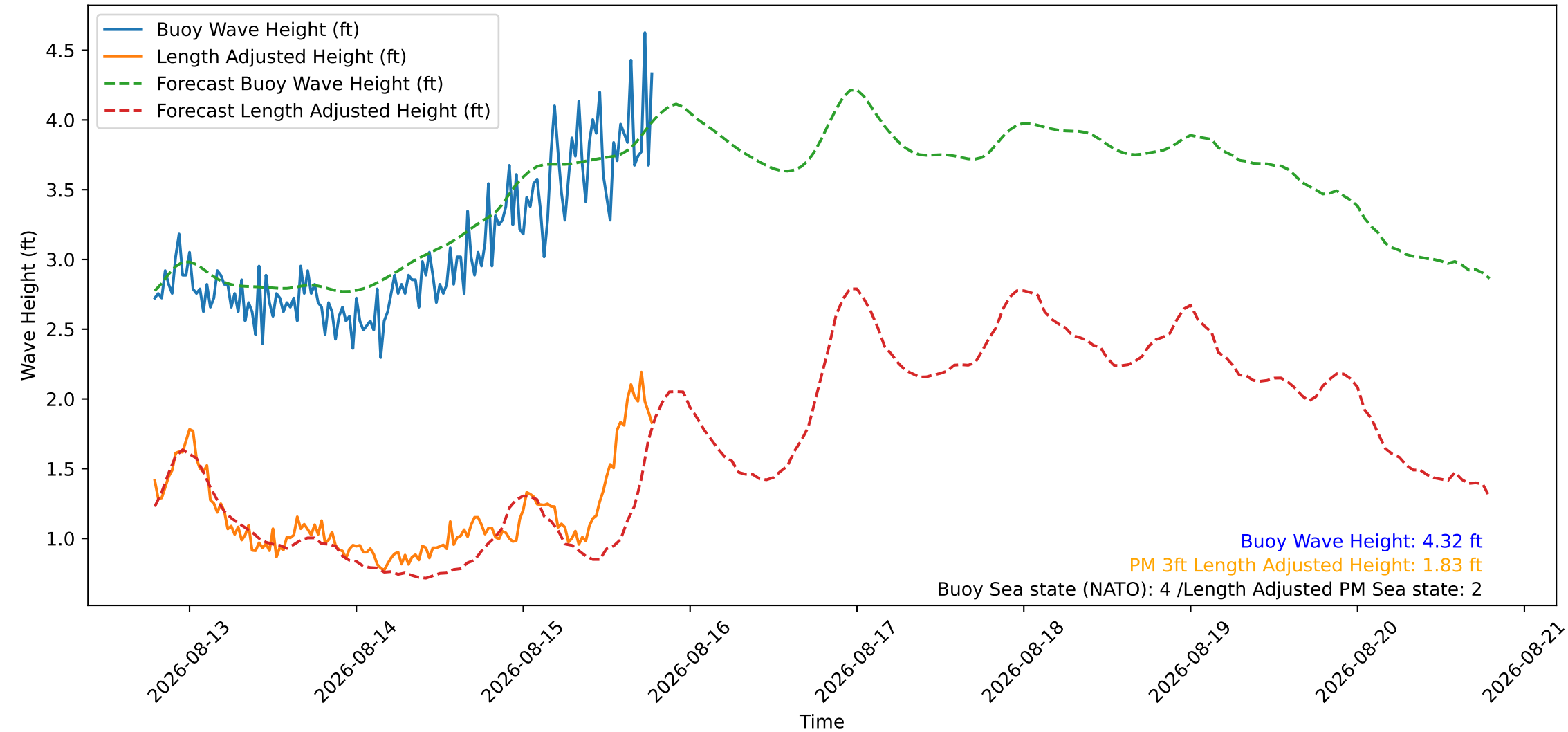
Wave Heights over Time for Oceanside Harbor at 2026-08-15 19:00:26
