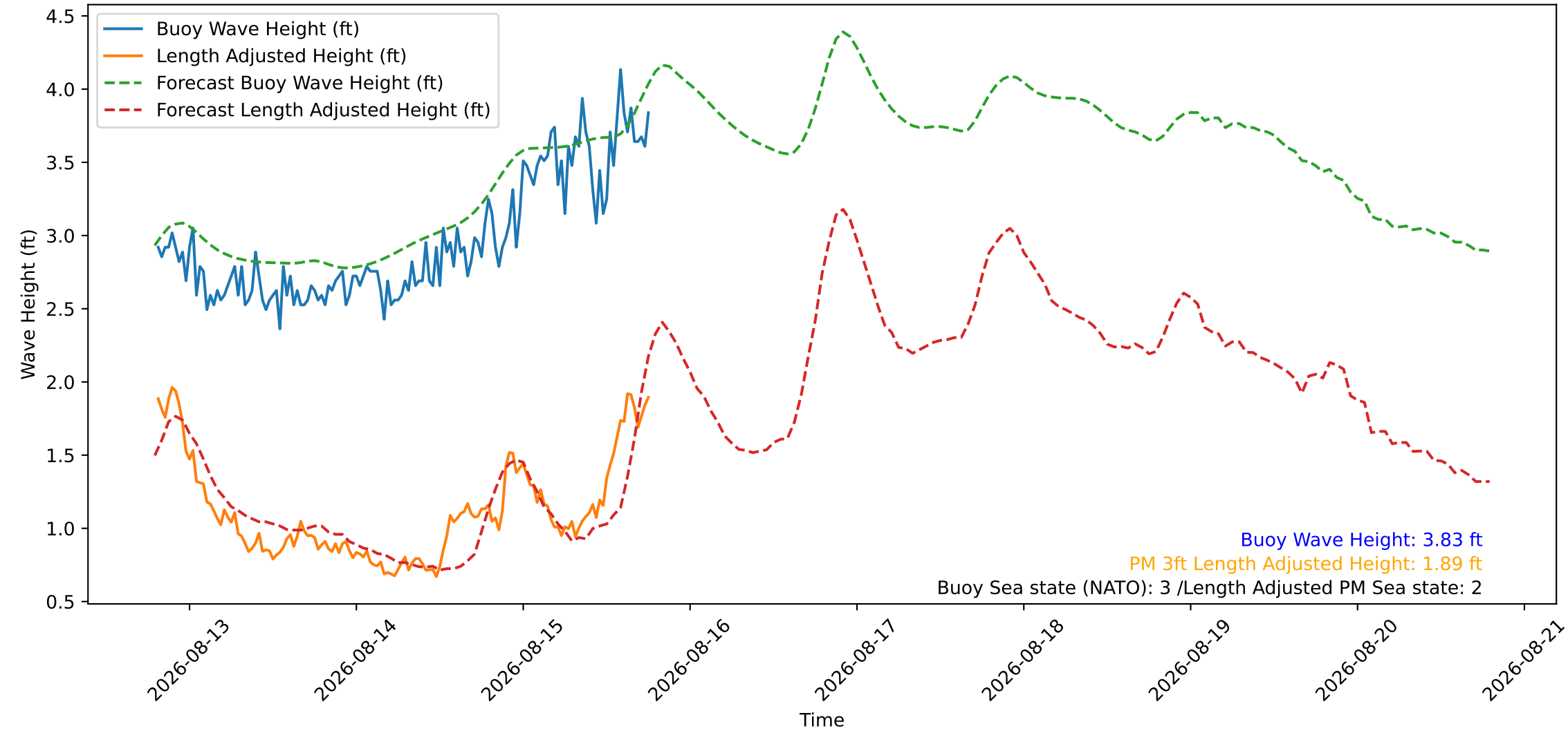
Wave Heights over Time for Green Beach at 2026-08-15 19:01:08
