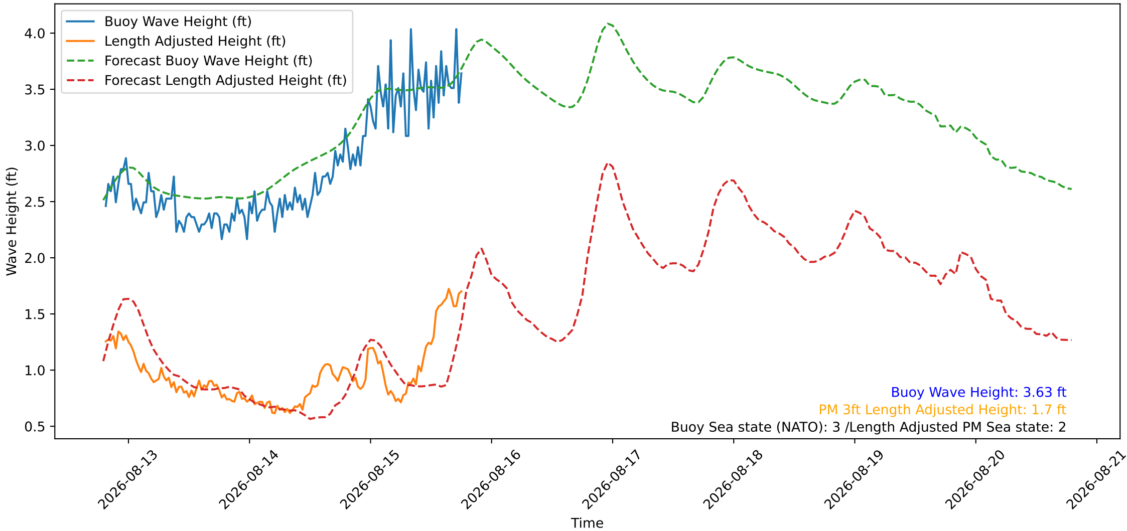
Wave Heights over Time for Red Beach at 2026-08-15 19:00:46
