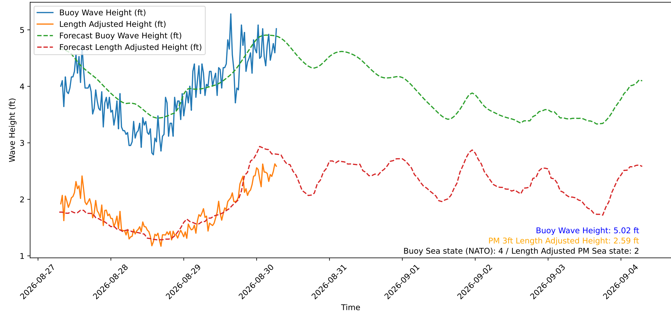
Wave Heights over Time for Oceanside Harbor at 2026-08-30 07:20:29
