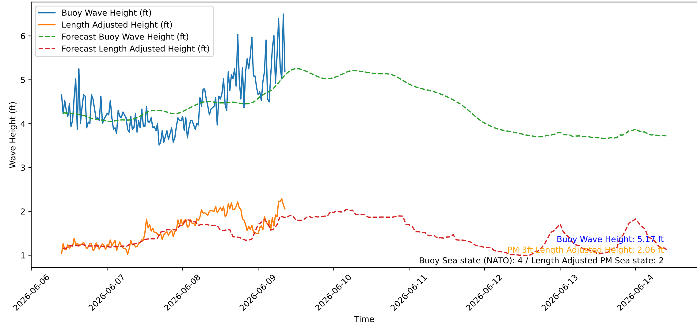
Wave Heights over Time for Oceanside Harbor at 2026-06-09 09:30:26
