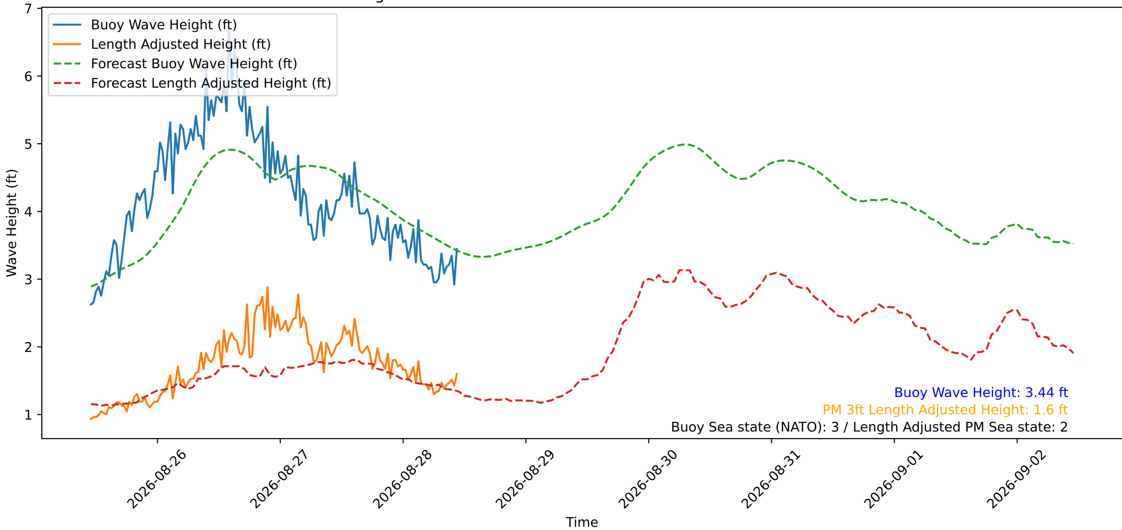
Wave Heights over Time for Oceanside Harbor at 2026-08-28 11:00:31
