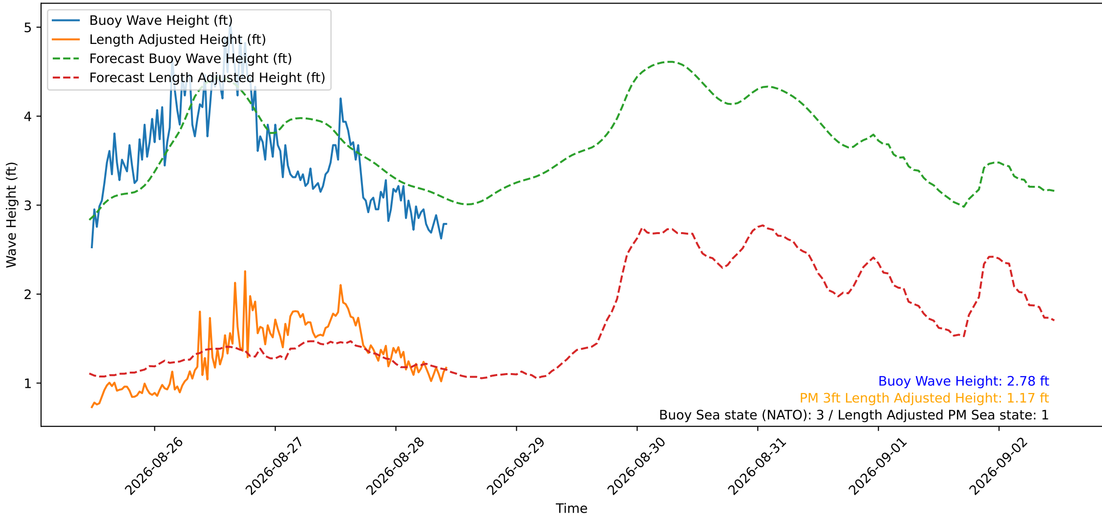
Wave Heights over Time for Red Beach at 2026-08-28 11:00:50
