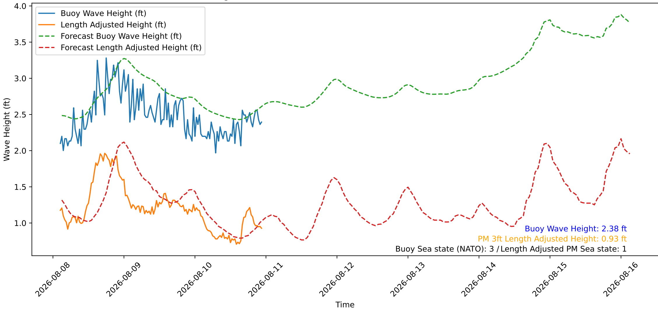
Wave Heights over Time for Oceanside Harbor at 2026-08-11 02:40:26
