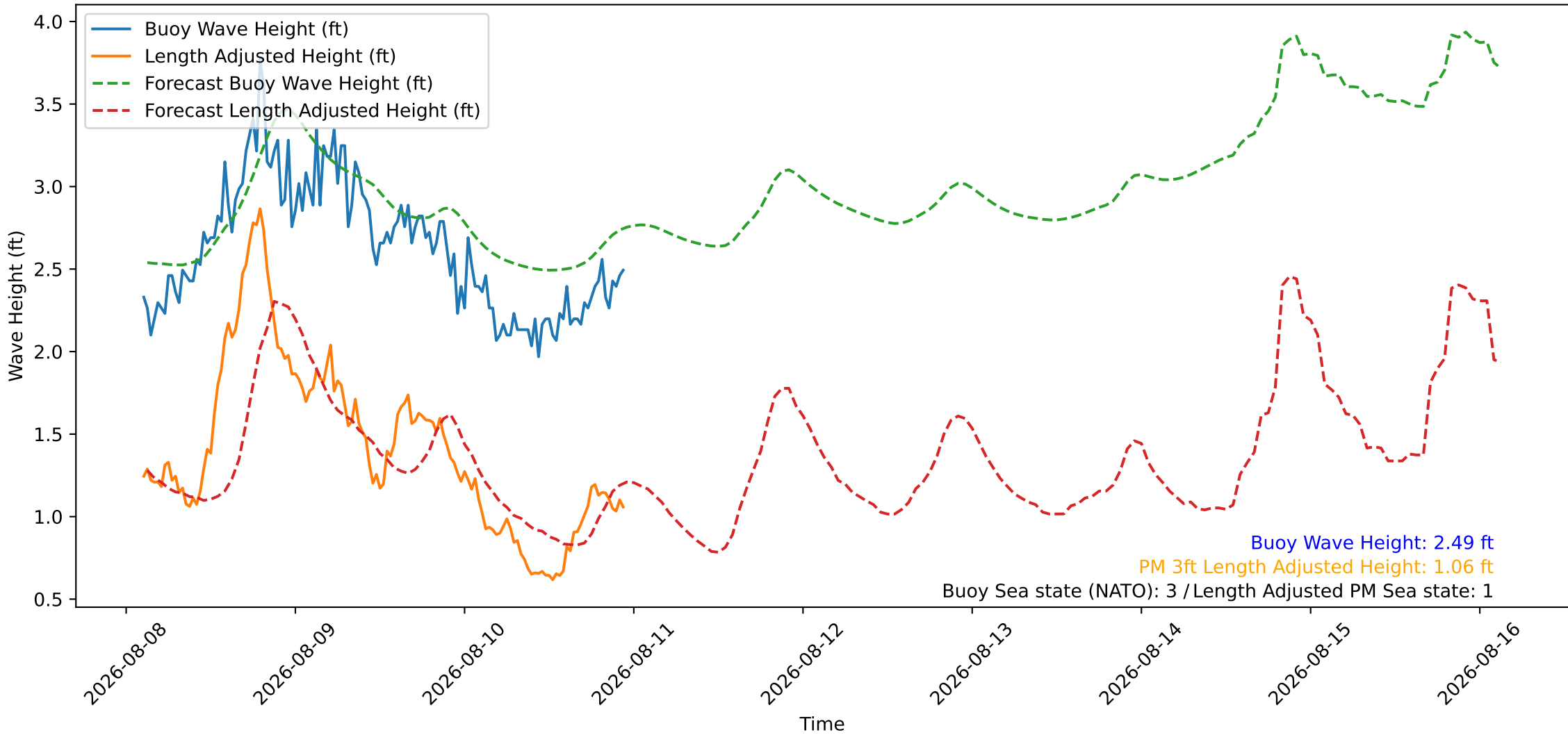
Wave Heights over Time for Green Beach at 2026-08-11 02:41:08
