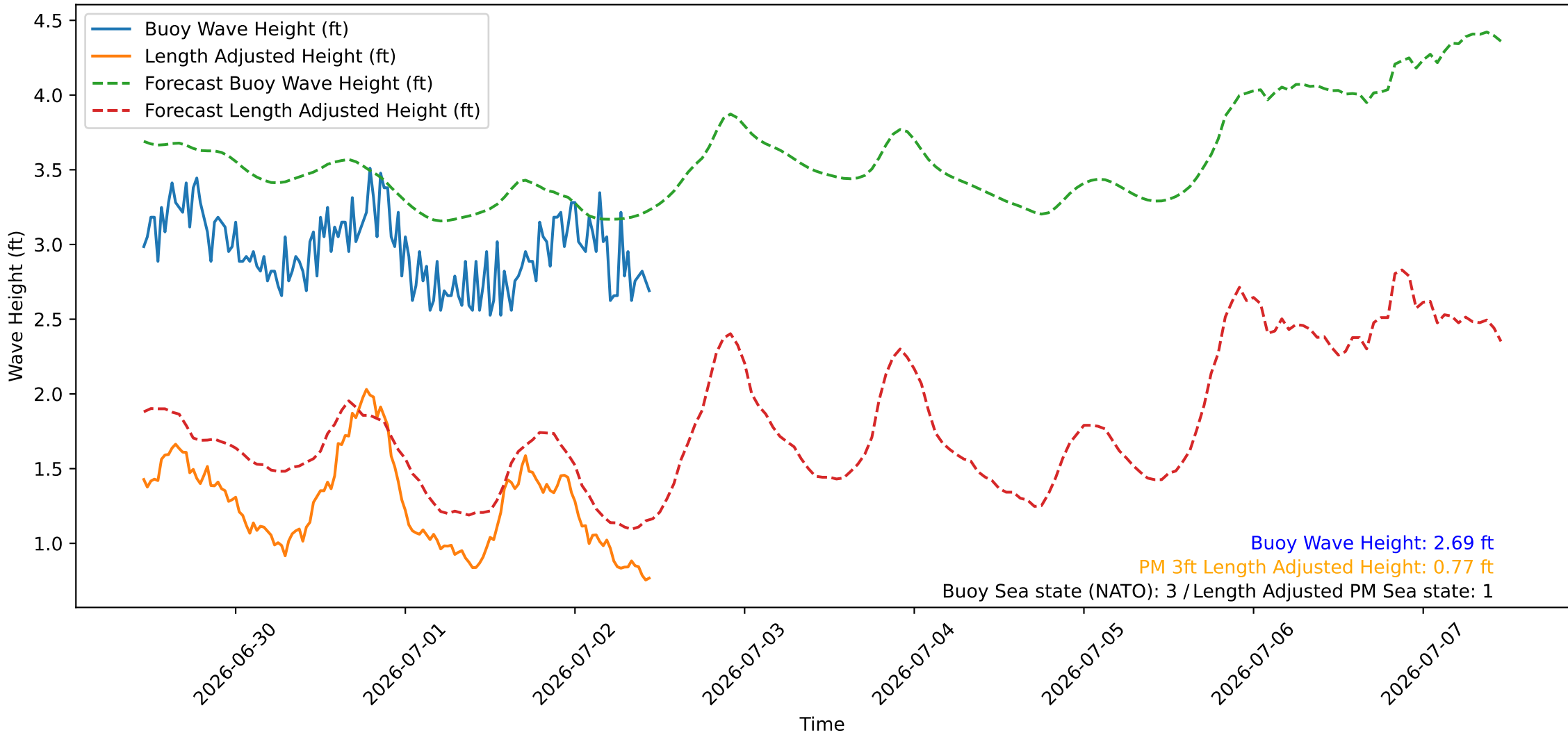
Wave Heights over Time for Green Beach at 2026-07-02 11:11:07
