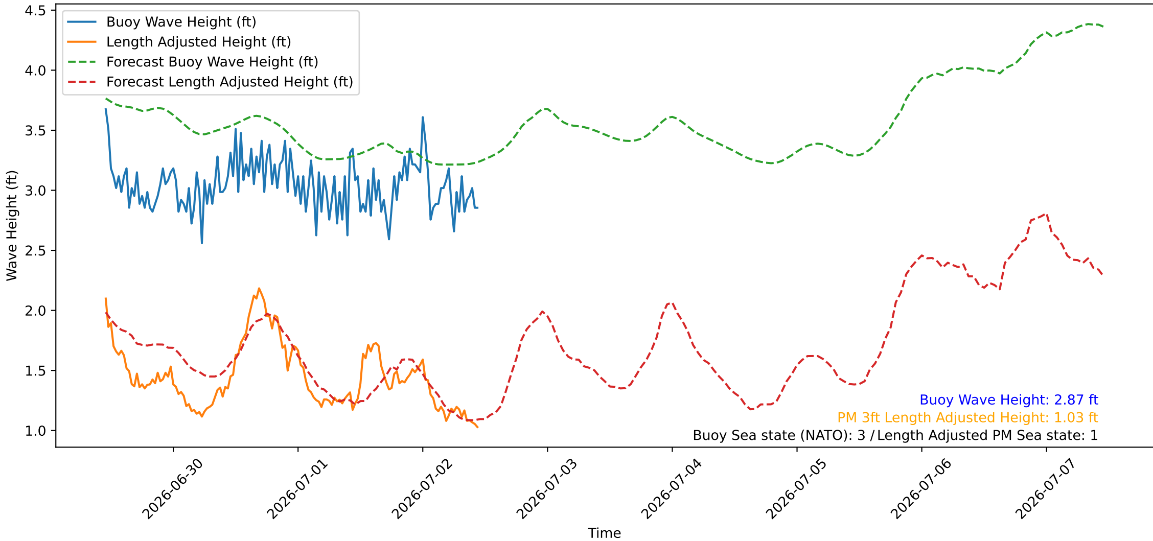
Wave Heights over Time for Oceanside Harbor at 2026-07-02 11:10:26
