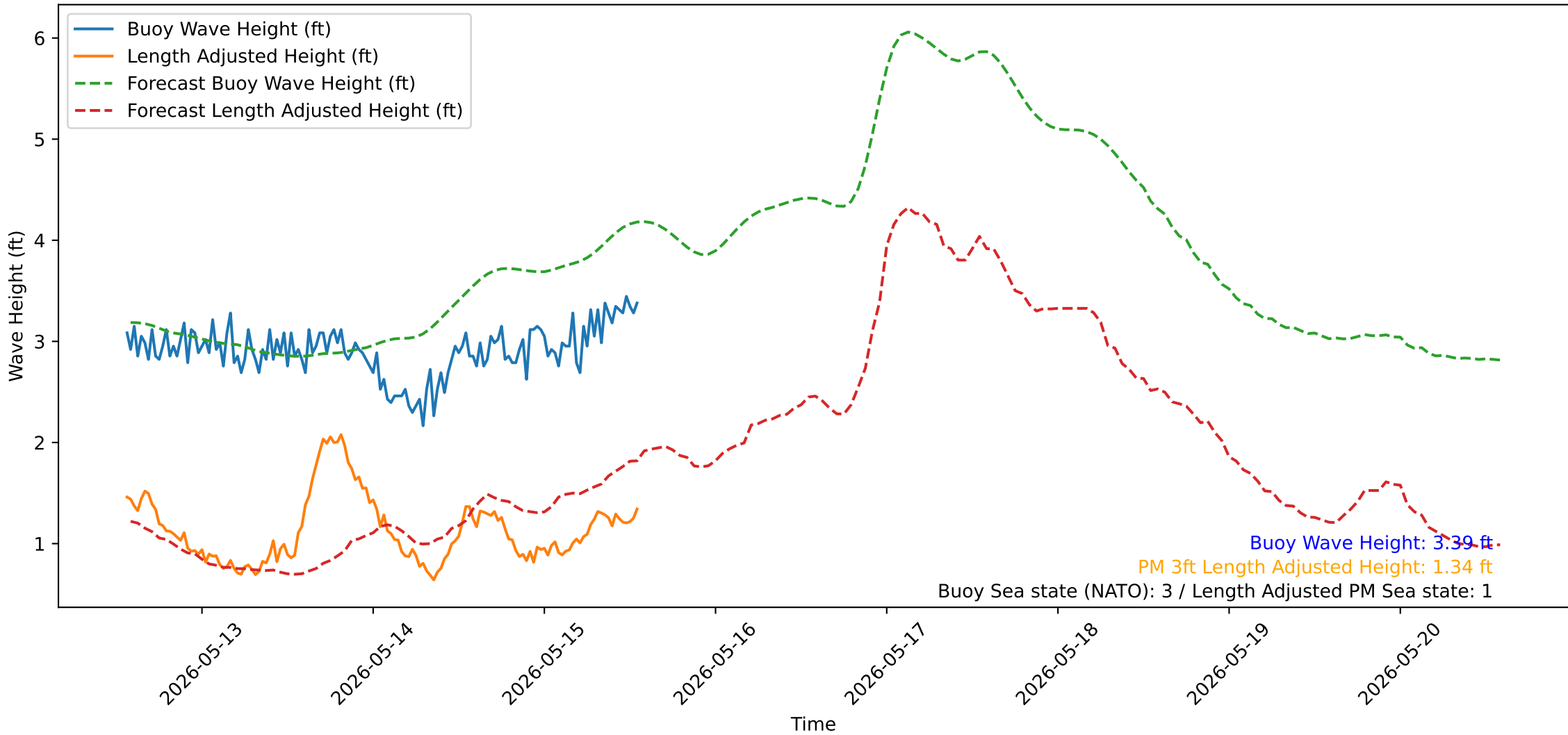
Wave Heights over Time for Oceanside Harbor at 2026-05-15 13:40:31
