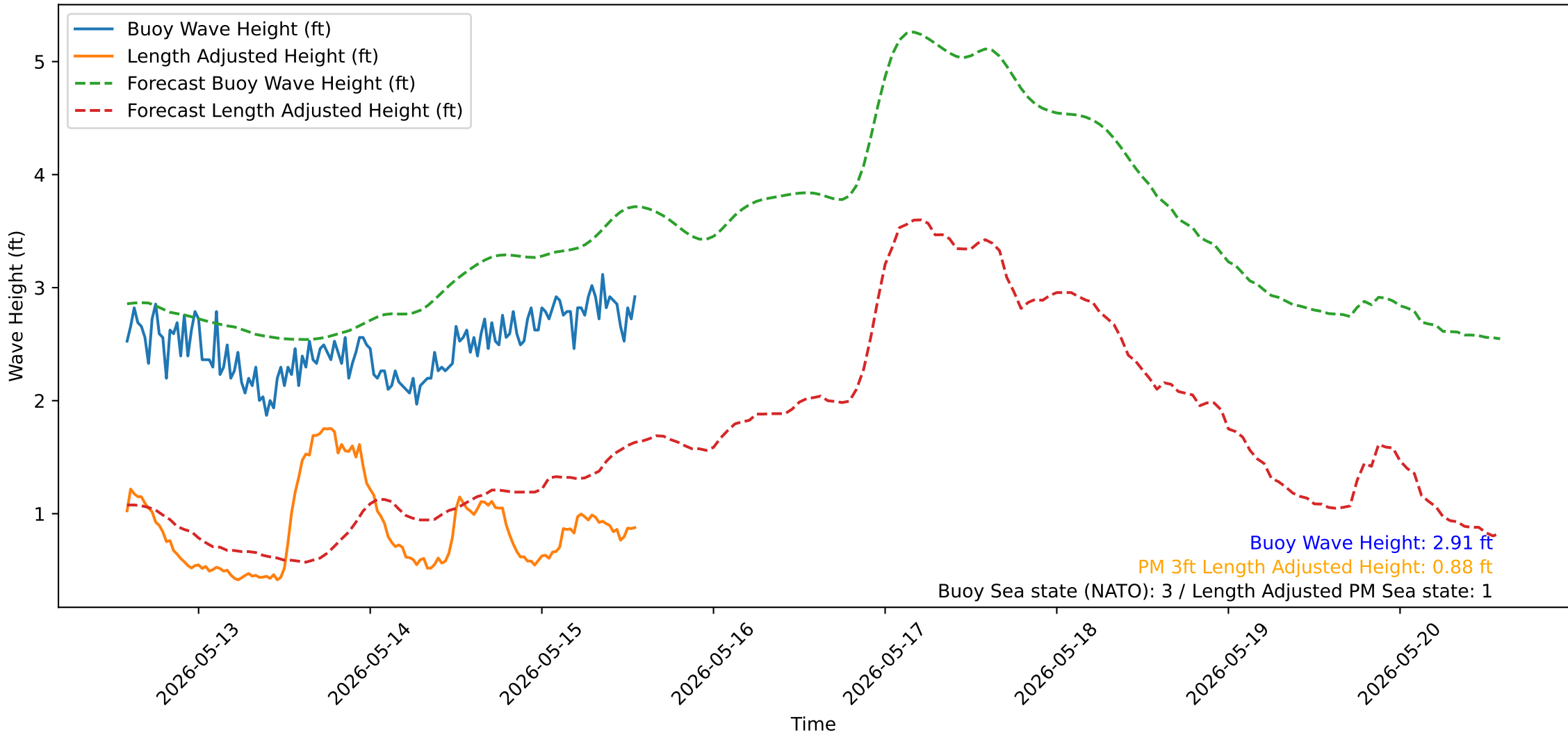
Wave Heights over Time for Red Beach at 2026-05-15 13:40:50
