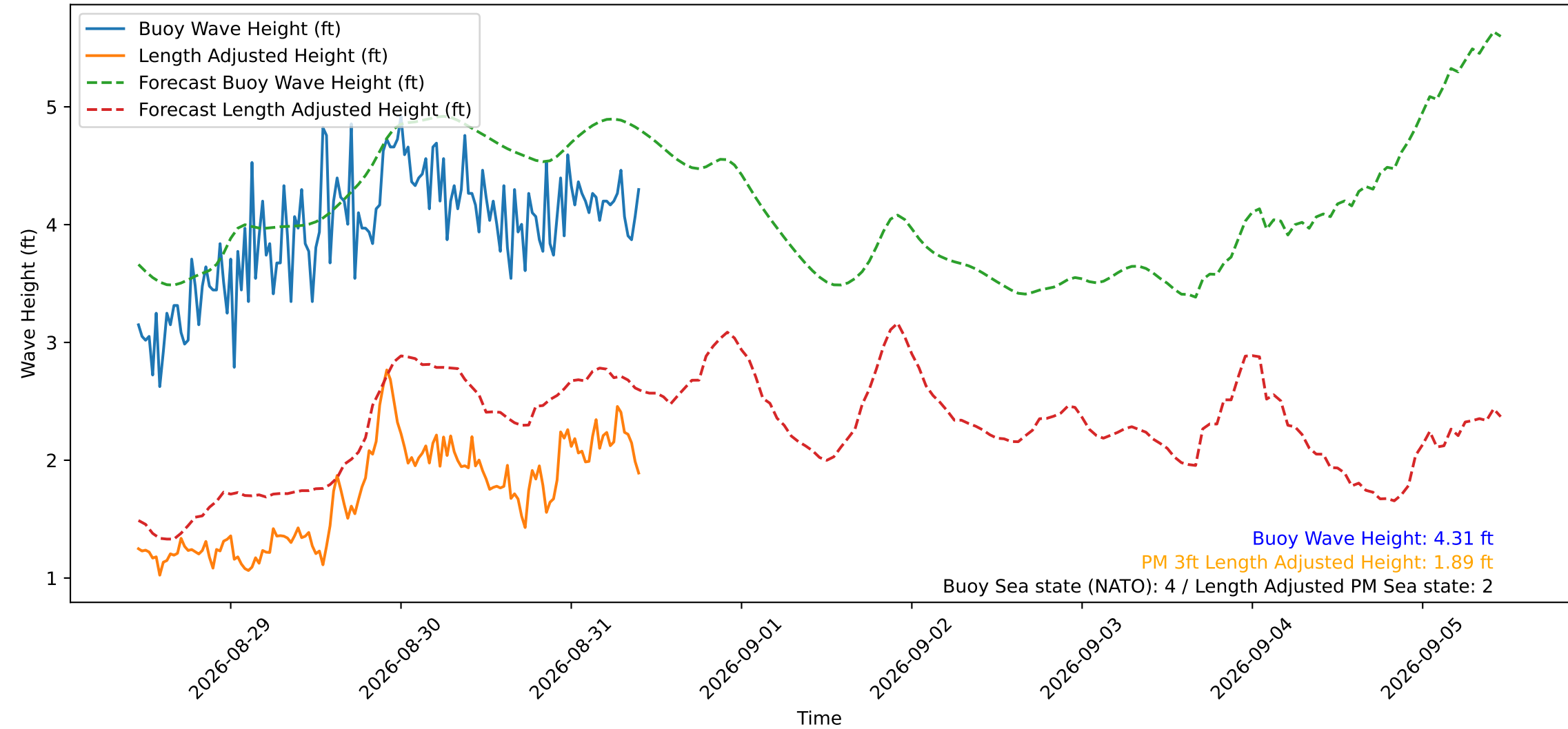
Wave Heights over Time for Green Beach at 2026-08-31 10:31:12
