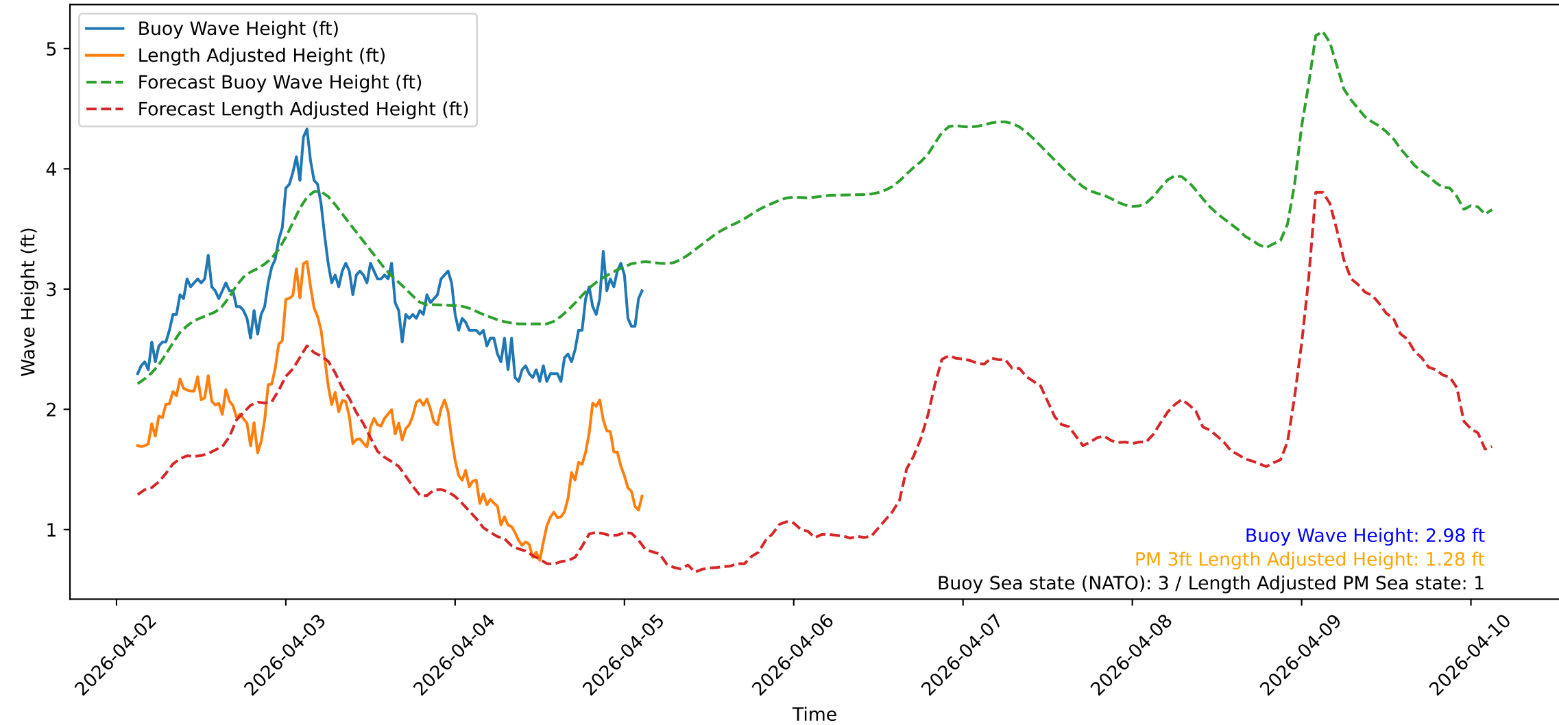
Wave Heights over Time for Green Beach at 2026-04-05 03:11:09
