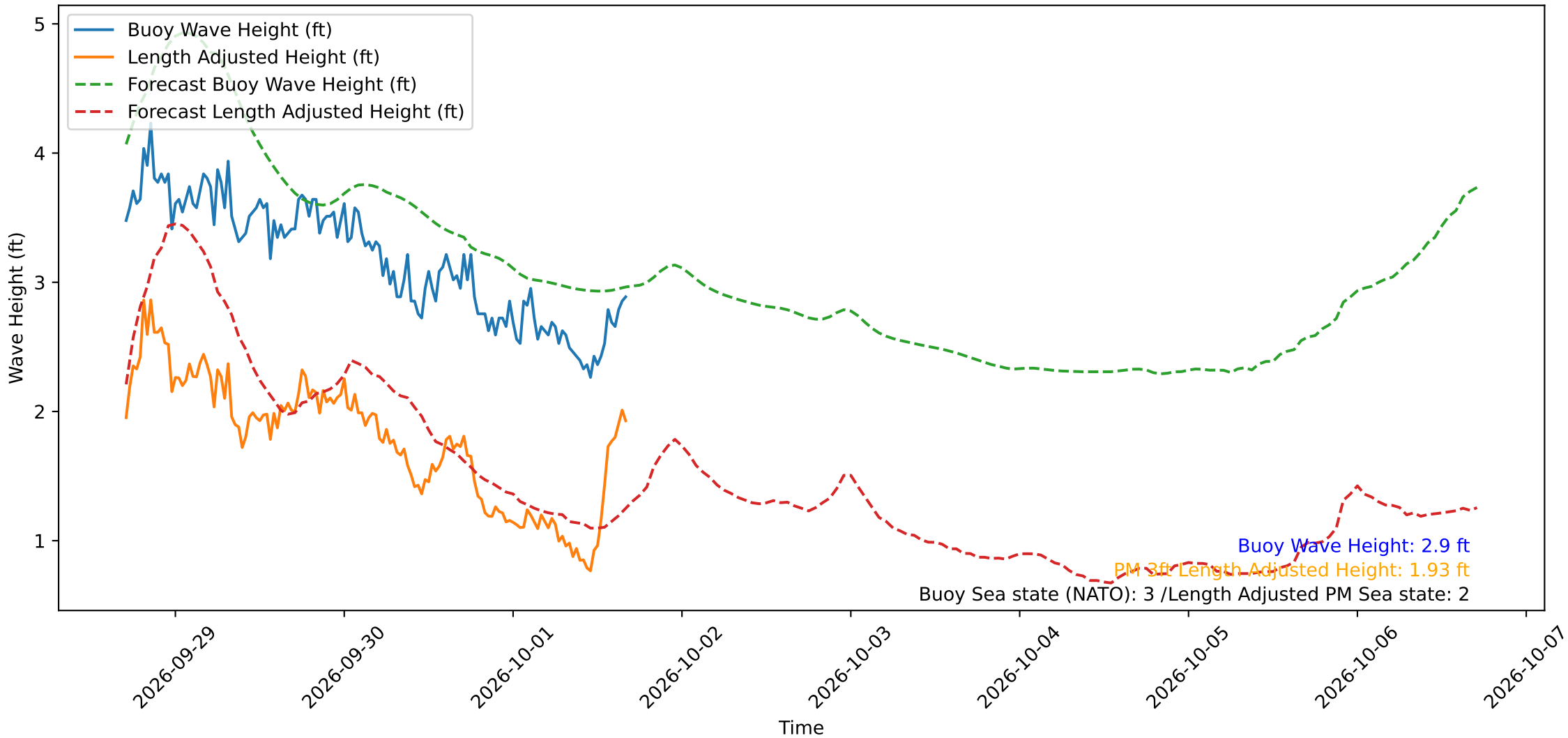
Wave Heights over Time for Oceanside Harbor at 2026-10-01 16:50:29
