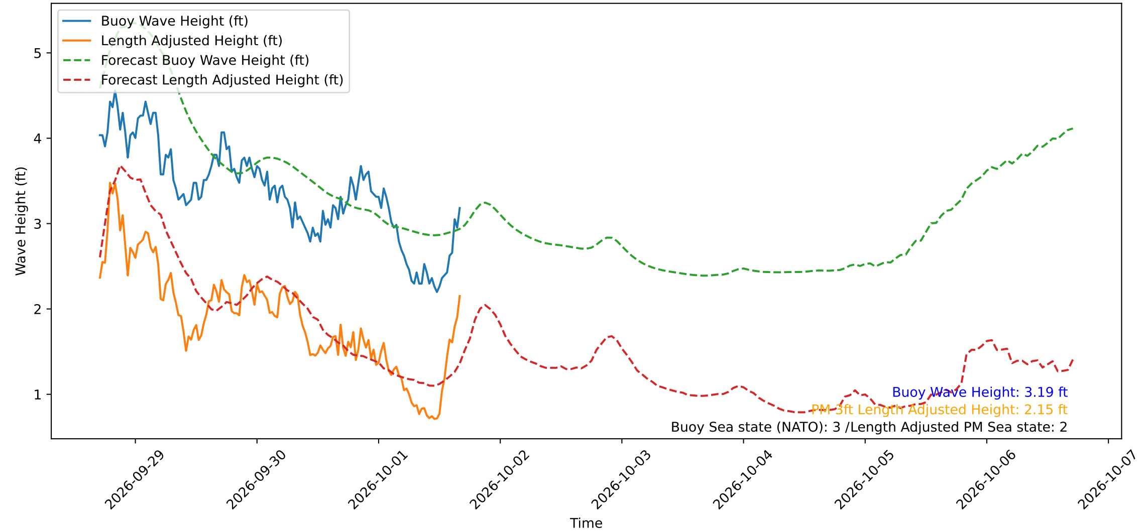
Wave Heights over Time for Green Beach at 2026-10-01 16:51:14
