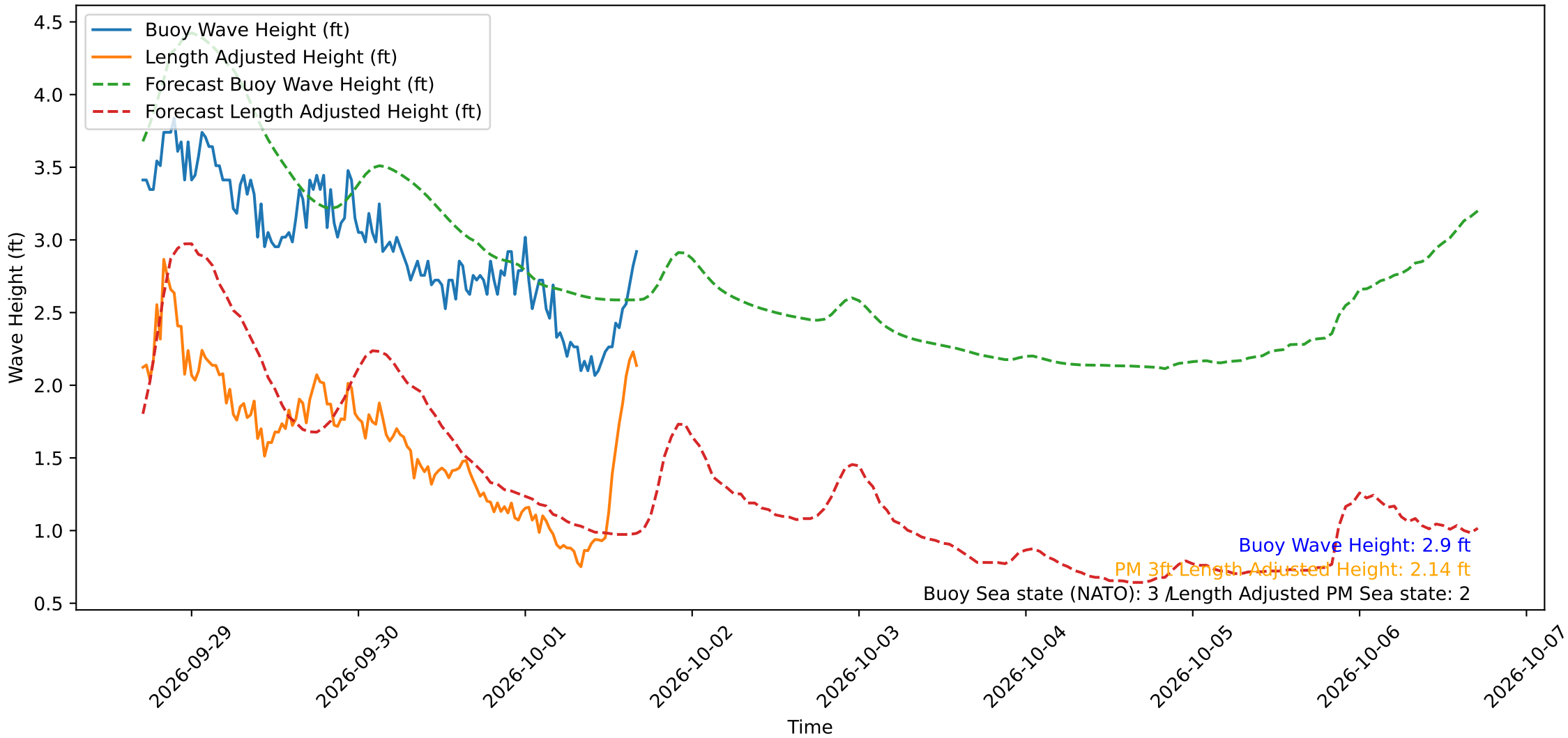
Wave Heights over Time for Red Beach at 2026-10-01 16:50:50
