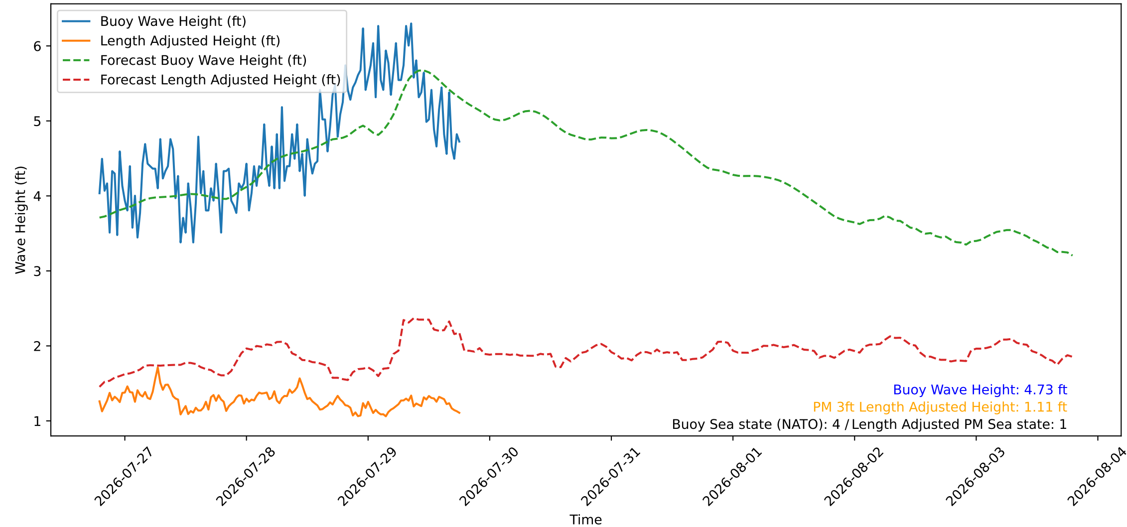
Wave Heights over Time for Green Beach at 2026-07-29 18:51:10
