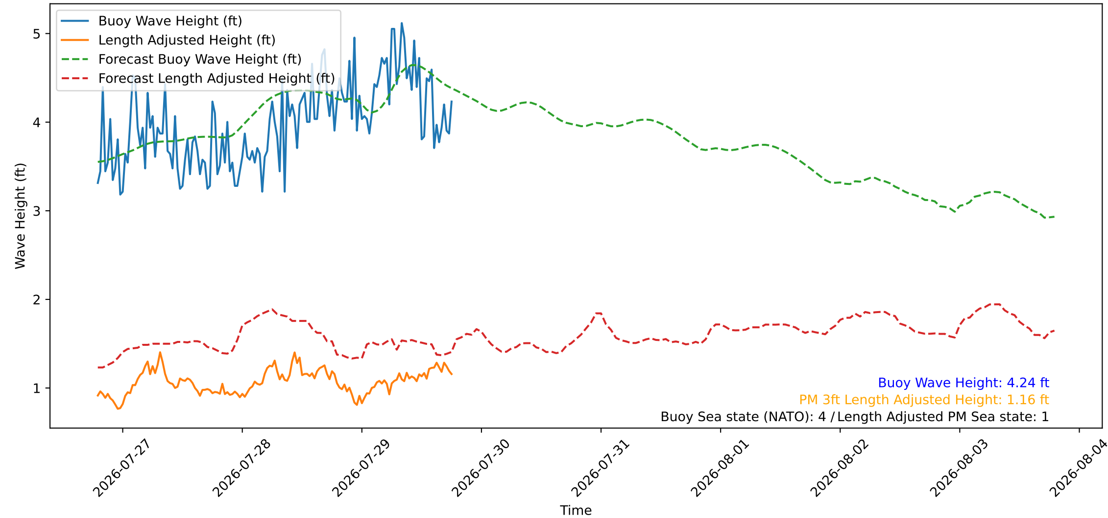
Wave Heights over Time for Red Beach at 2026-07-29 18:50:47
