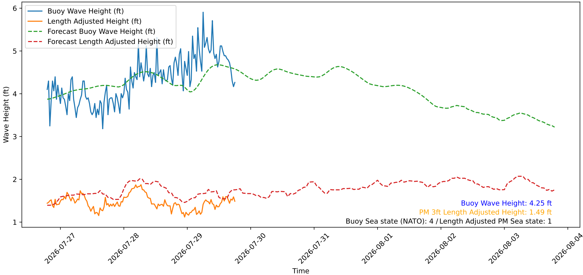
Wave Heights over Time for Oceanside Harbor at 2026-07-29 18:50:26
