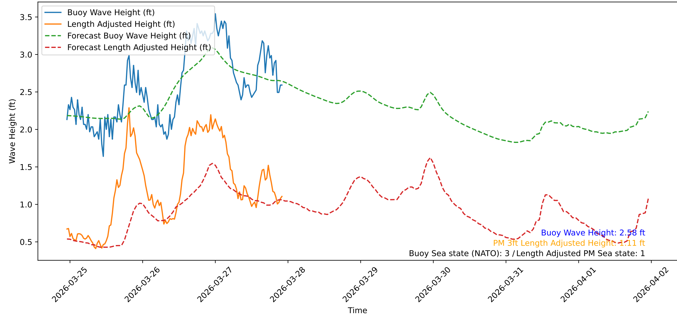
Wave Heights over Time for Green Beach at 2026-03-27 23:01:09
