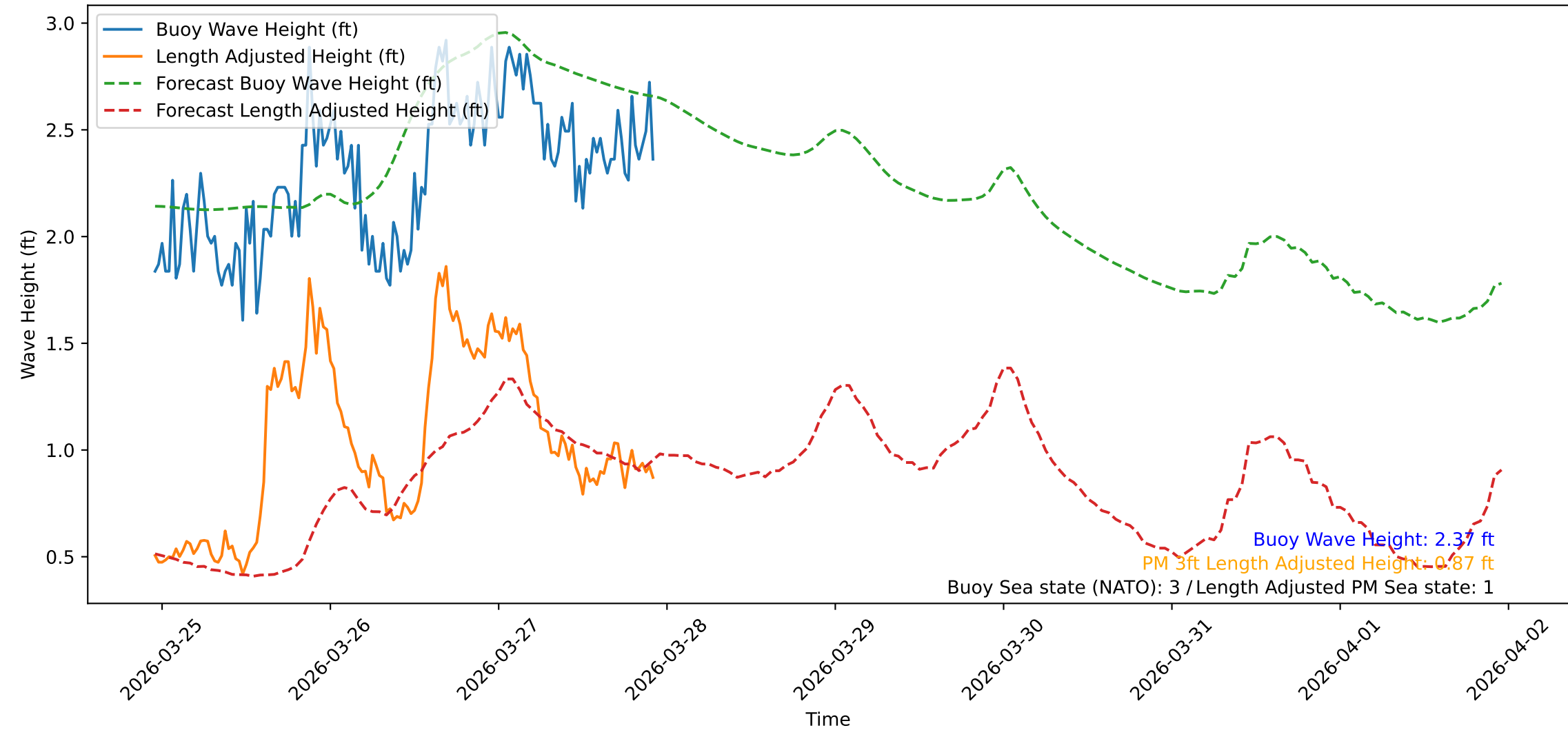
Wave Heights over Time for Oceanside Harbor at 2026-03-27 23:00:31
