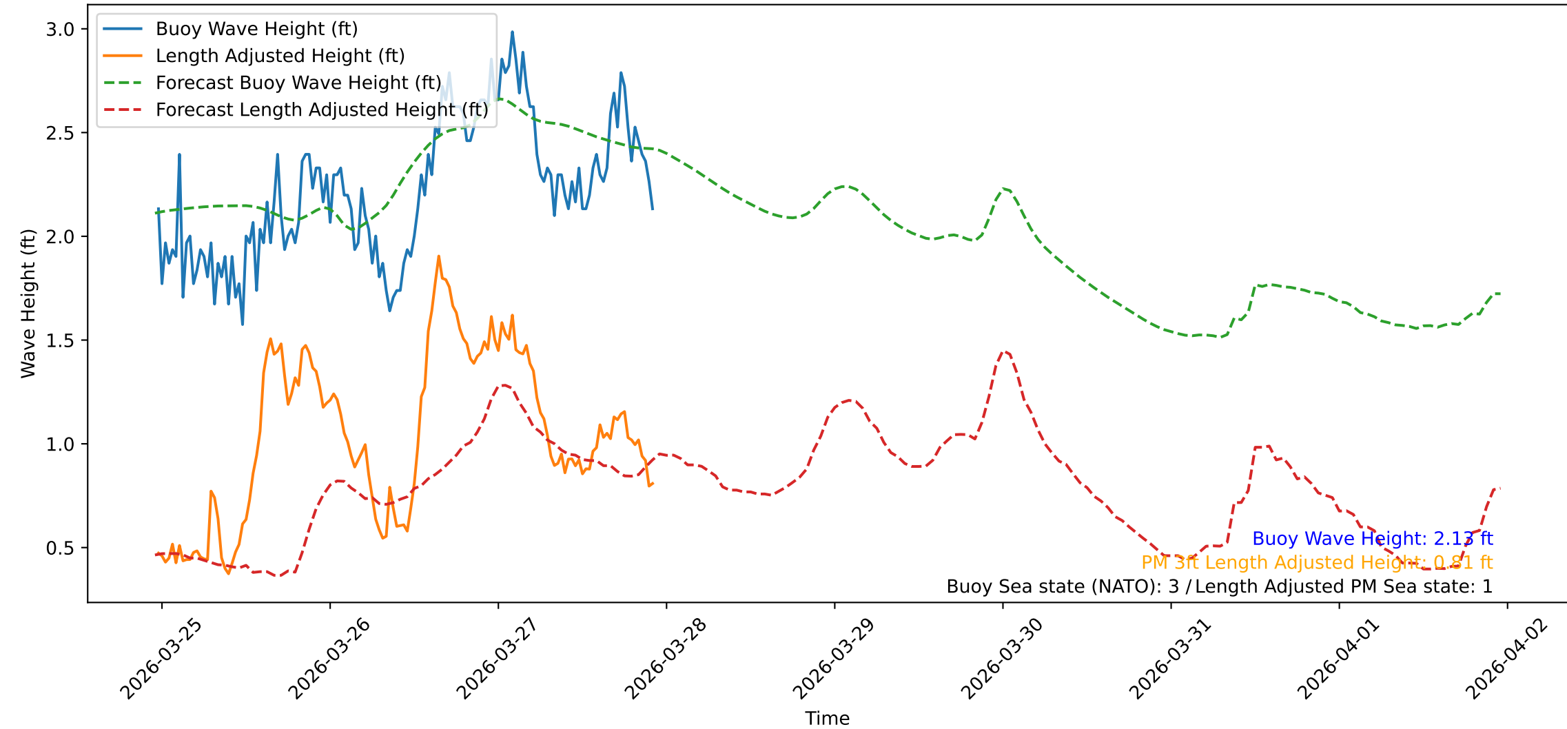
Wave Heights over Time for Red Beach at 2026-03-27 23:00:47
